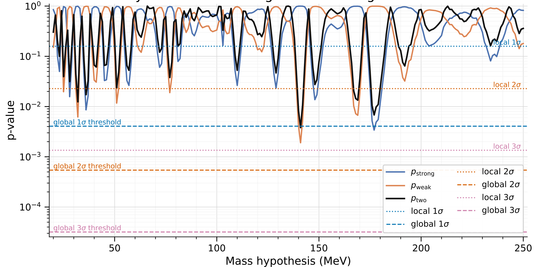
90% CL toy-band tail-area diagnostics with significance references
