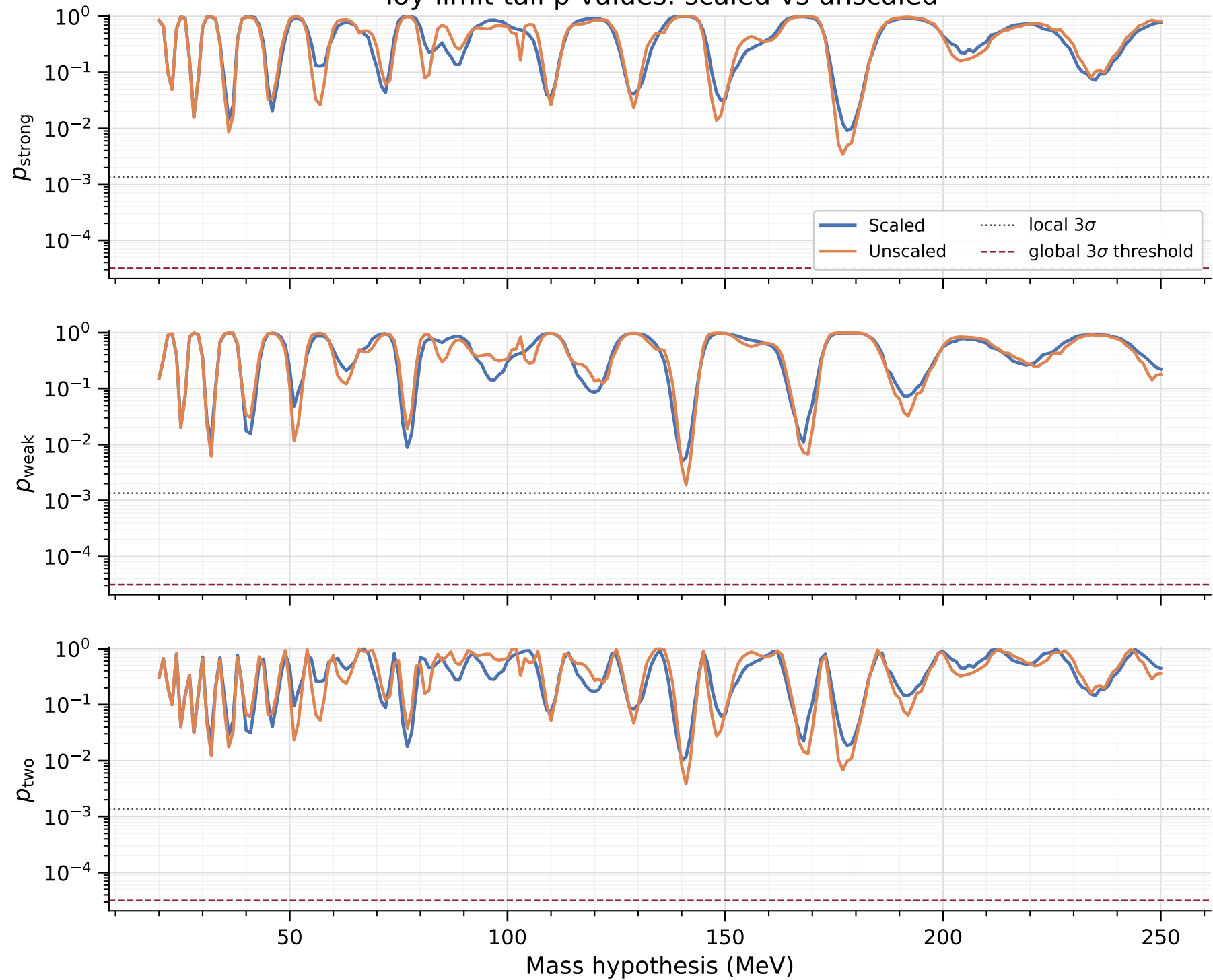
Toy-limit tail p-values: scaled vs unscaled
