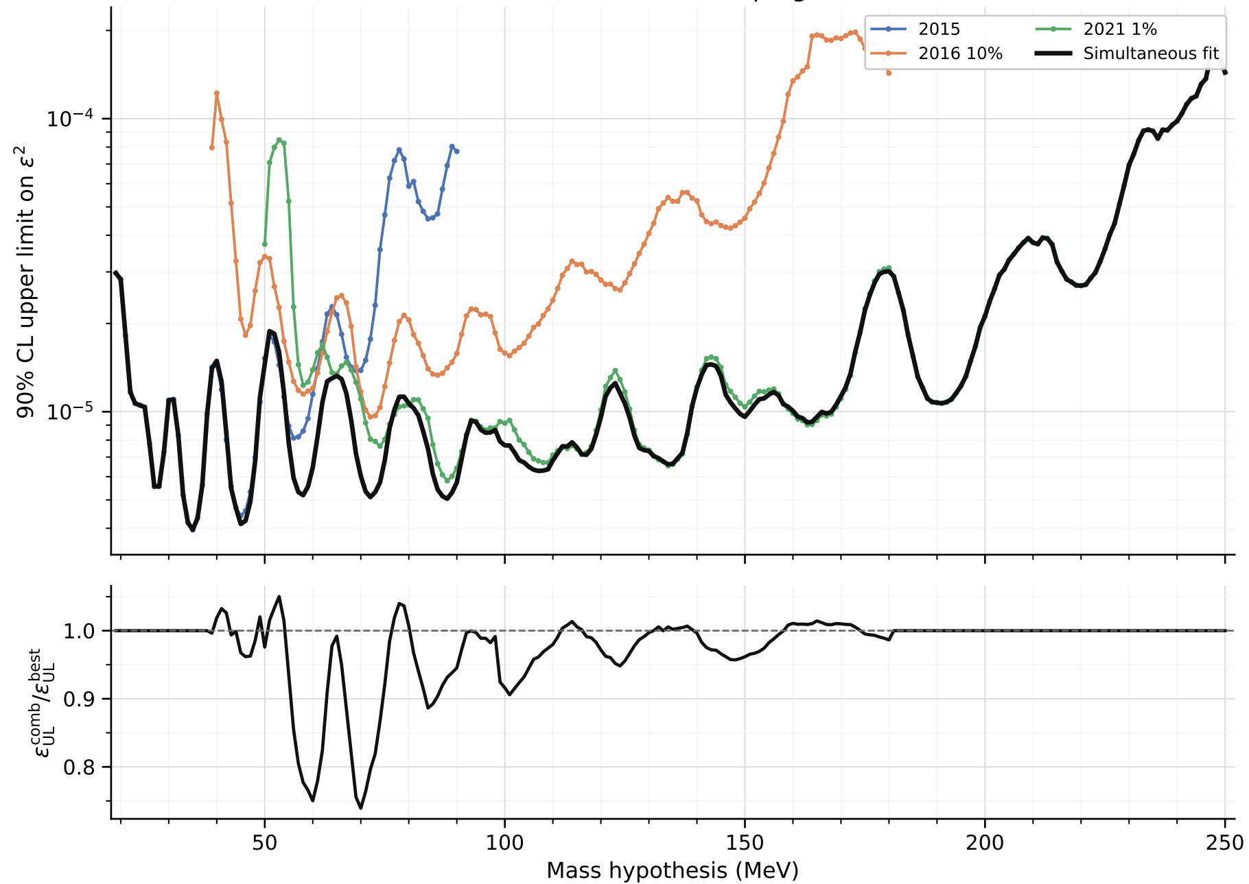
Observed limits from the individual campaigns and simultaneous fit
