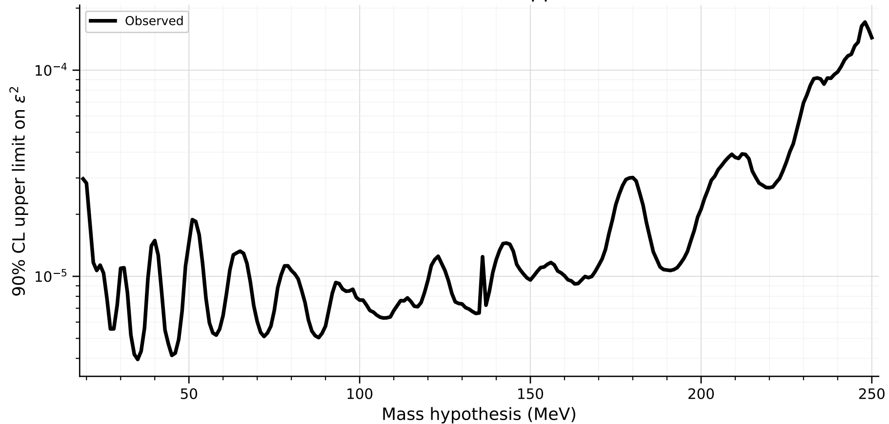
Observed 90% CL upper limit
