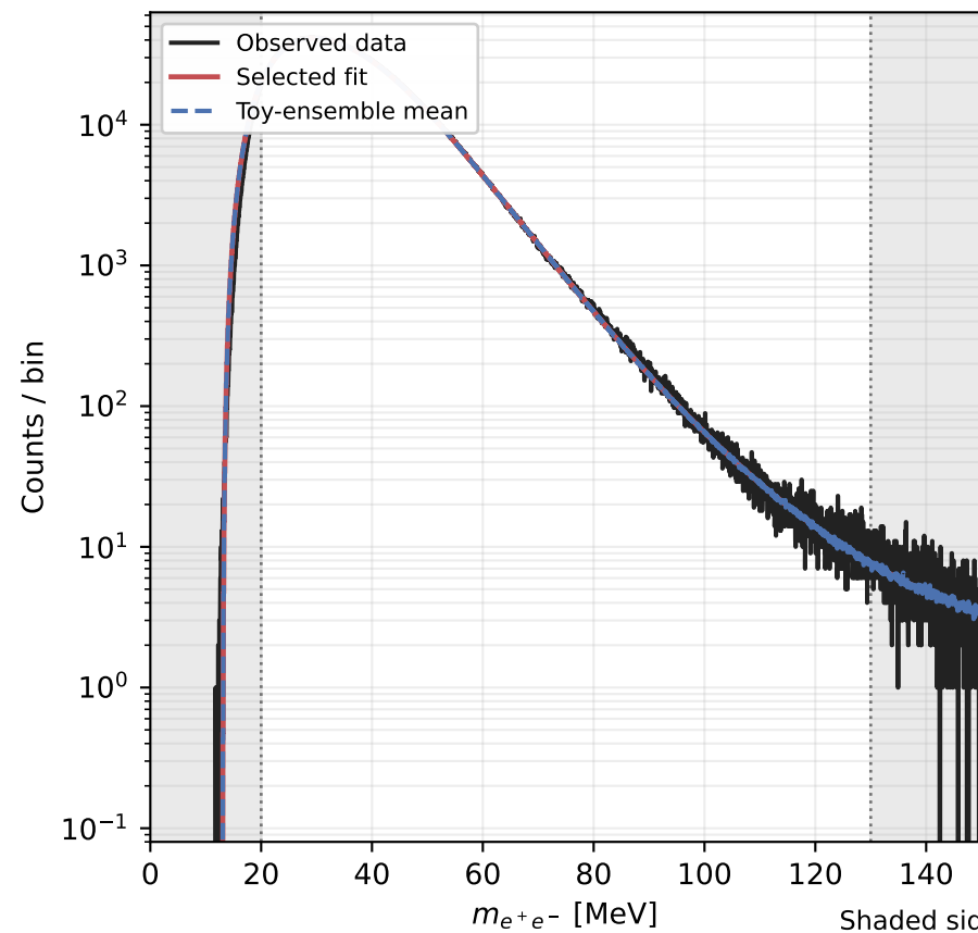
HPS 2015 / shifted sigmoid*power*exp + tail Scan [20, 130] MeV / N events = 2.145e+07
