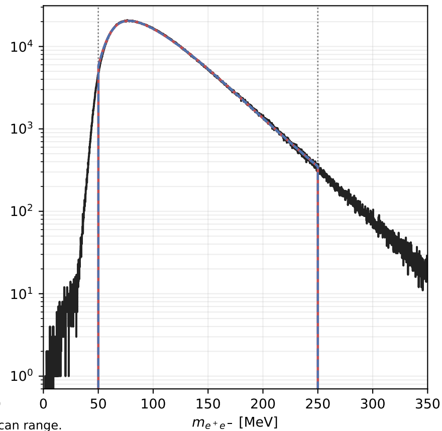
HPS 2021 1% / sigmoid*power*exp + raw expquad Scan [50, 250] MeV / N events = 1.229e+07
