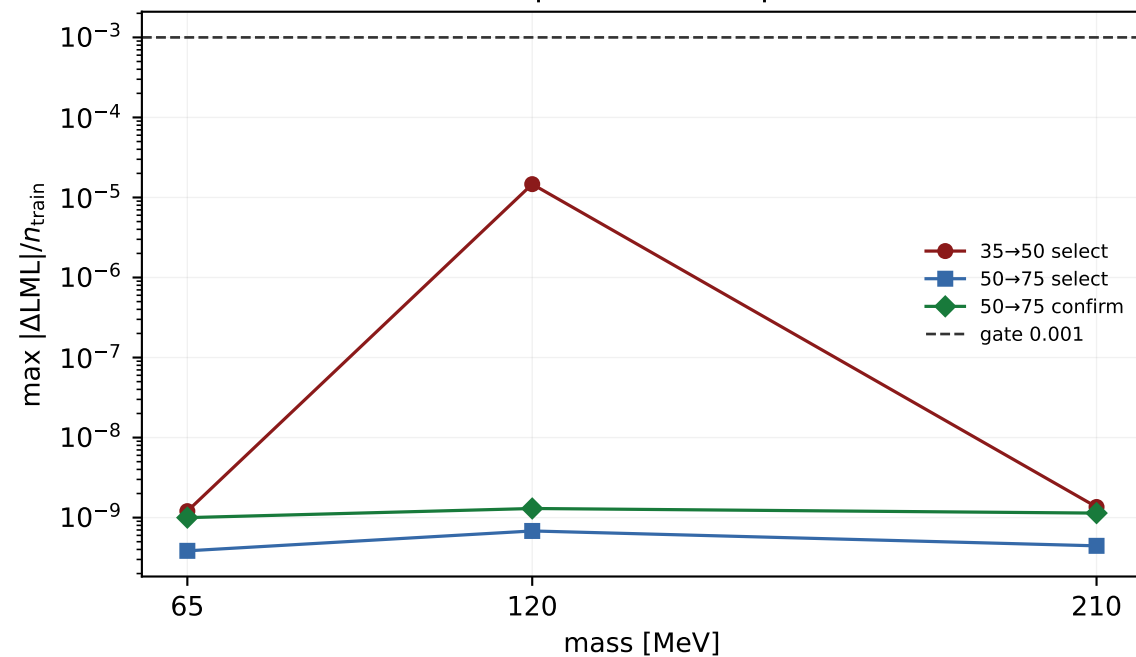
Same-input likelihood plateau
