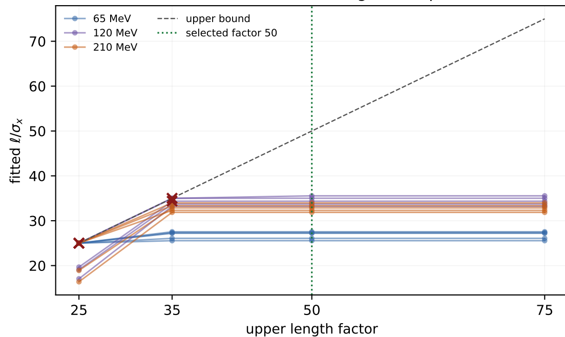
Same-input length-coordinate plateau
