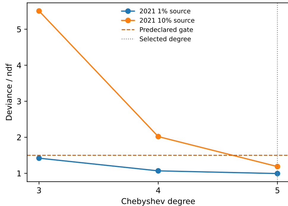
Native-bin Poisson deviance
