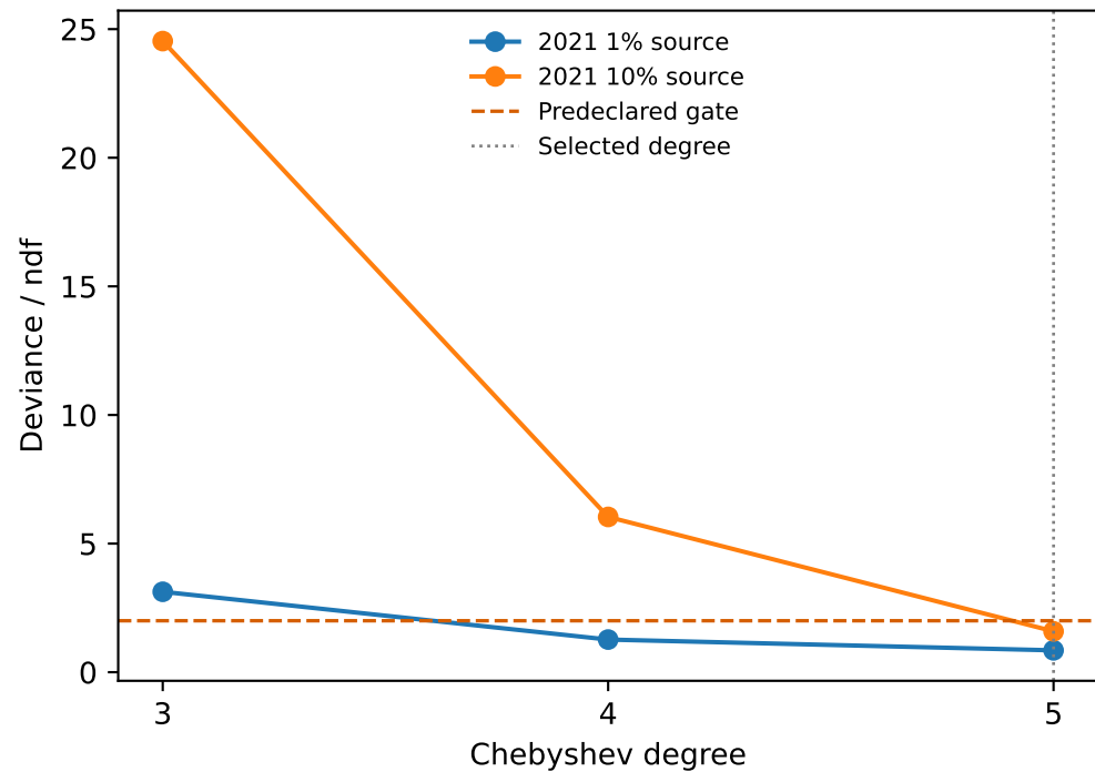
Five-bin Poisson deviance
