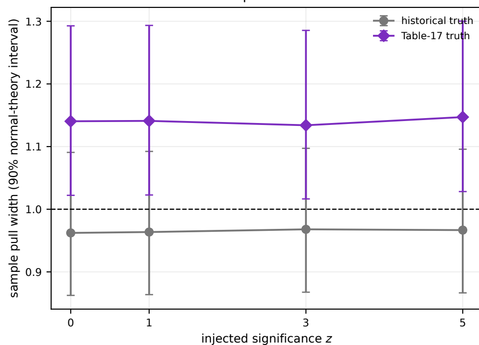
Width response at 65 MeV
