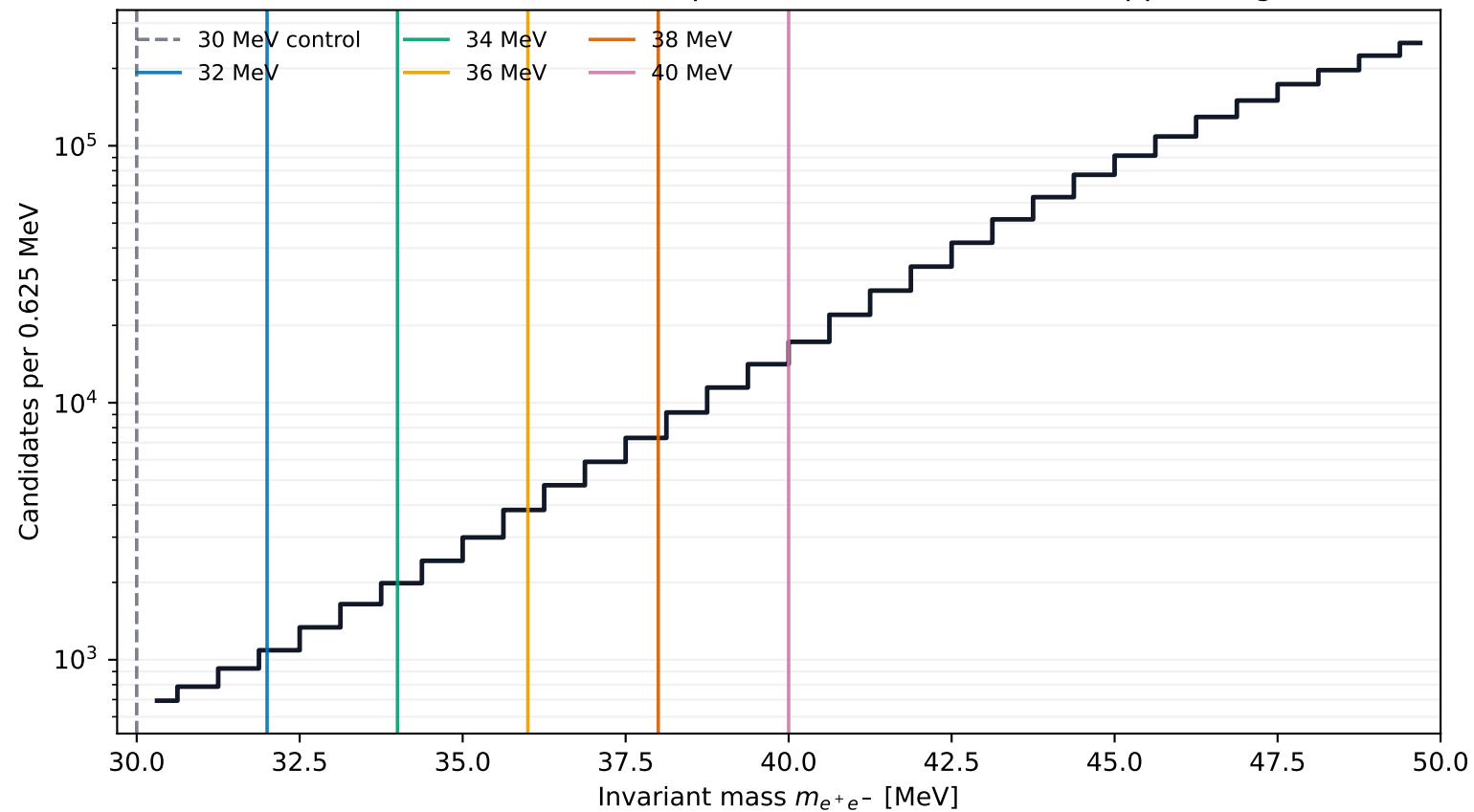
2021 native-10% threshold spectrum and scanned GP-support edges
