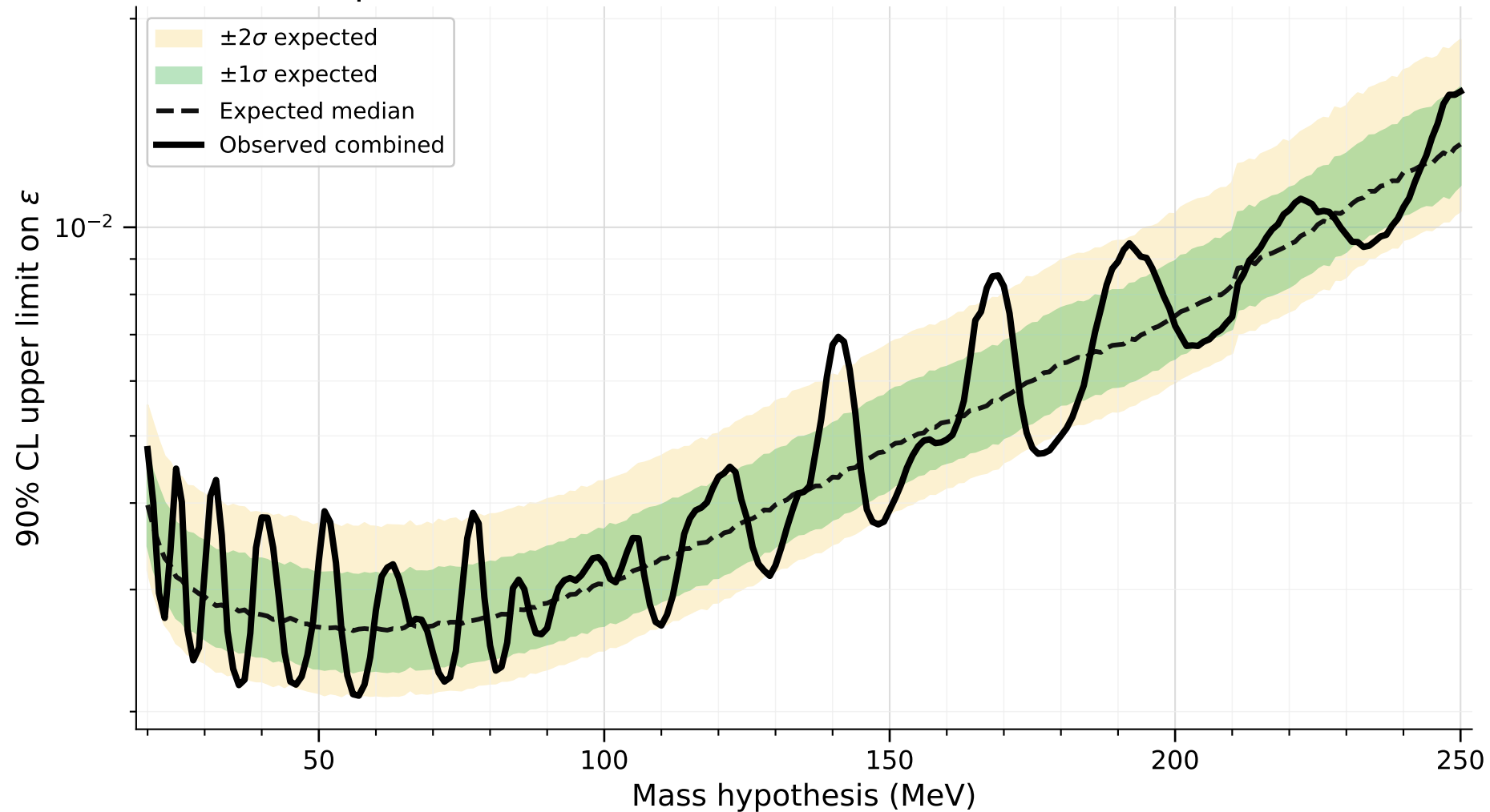
90% CL expected bands and observed simultaneous-combination limit
