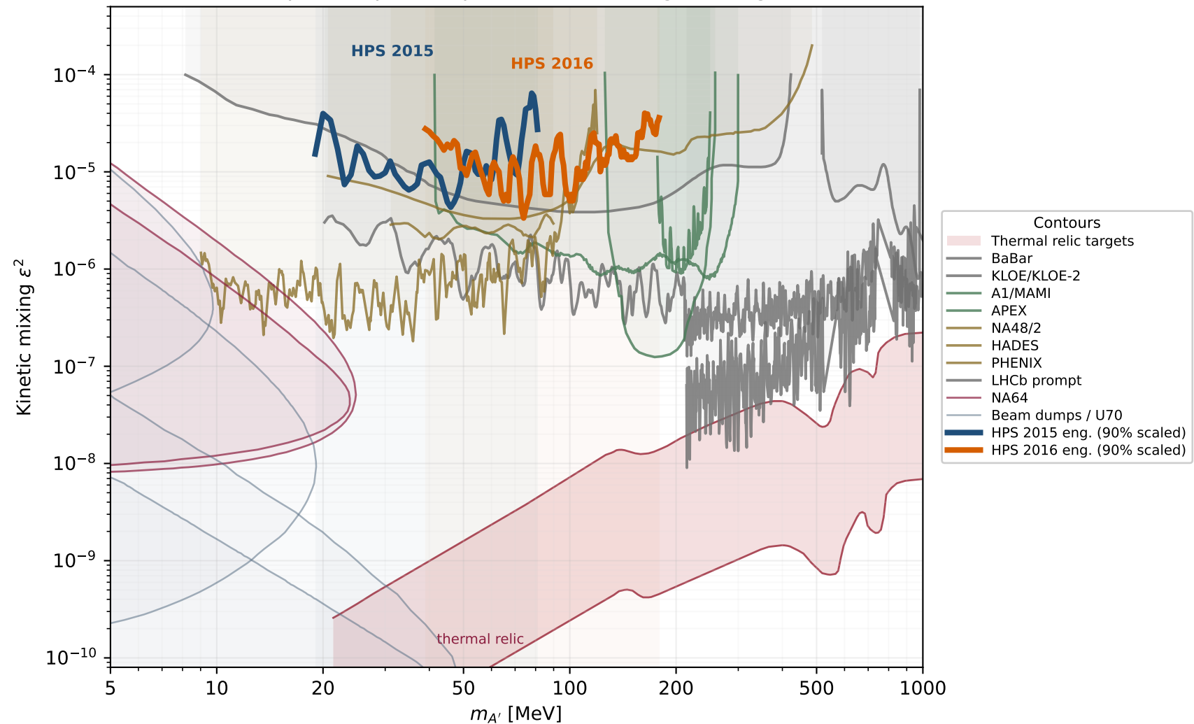
Visible dark-photon phase space with HPS engineering-run limits
