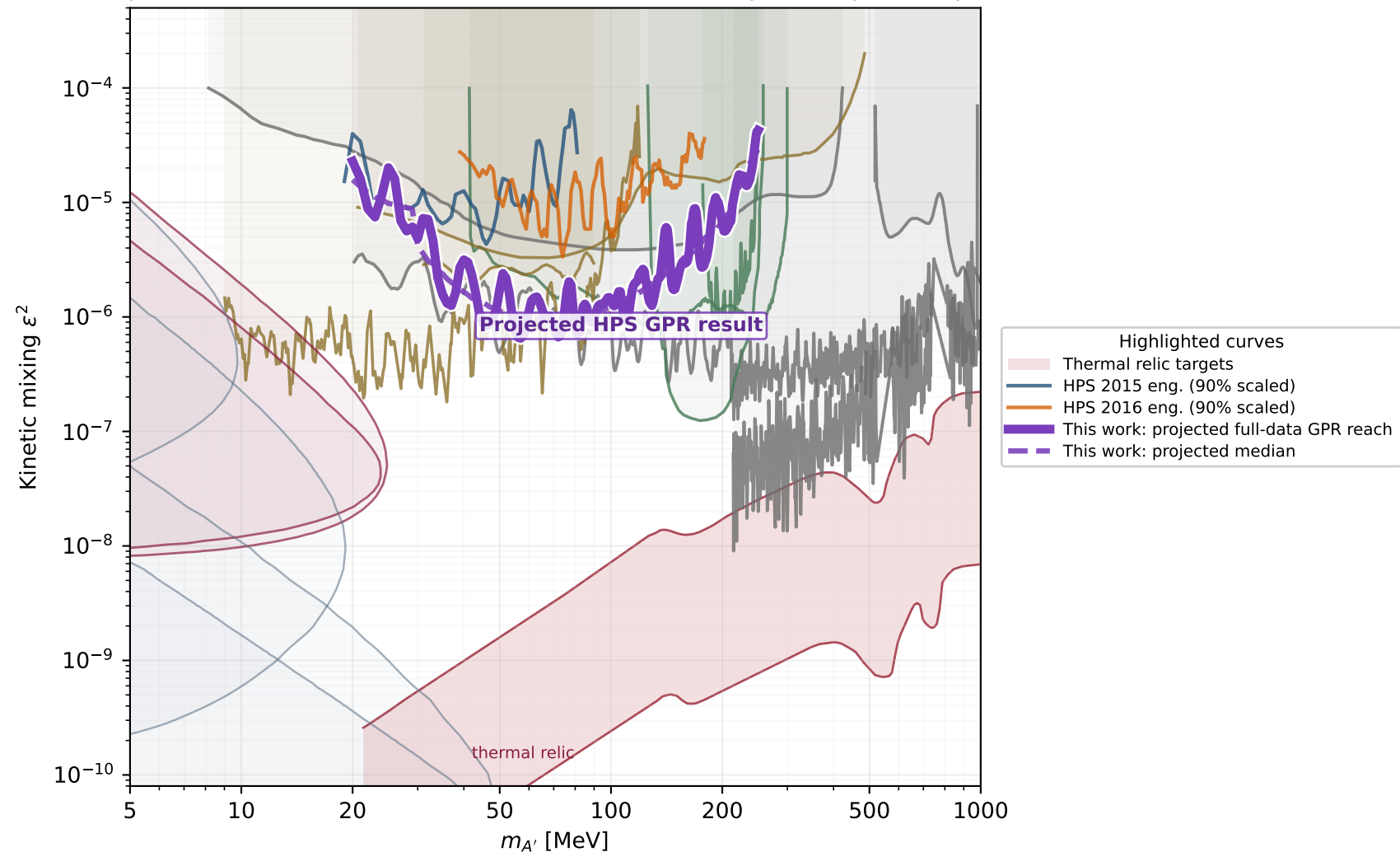
Projected full-data HPS GPR reach in visible dark-photon phase space
