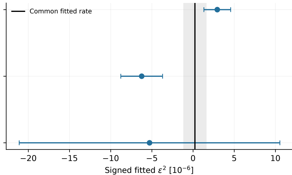
76 MeV: \Delta D = 9.405 (2 freed amplitudes)
