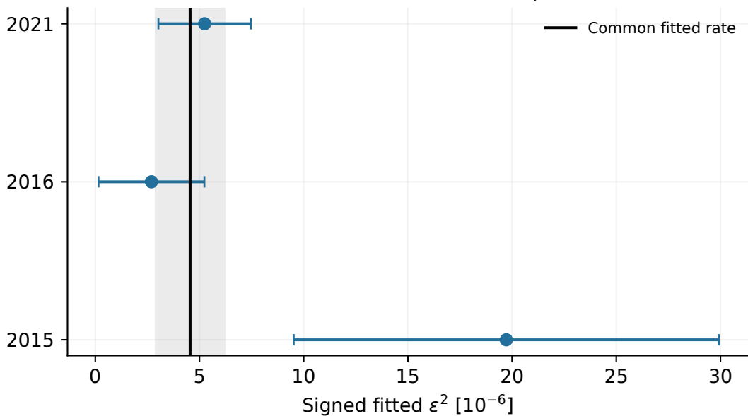
66 MeV: \Delta D = 2.845 (2 freed amplitudes)
