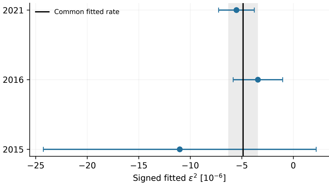
72 MeV: \Delta D = 0.713 (2 freed amplitudes)
