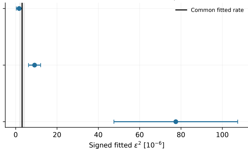
92 MeV: \Delta D = 11.552 (2 freed amplitudes)
