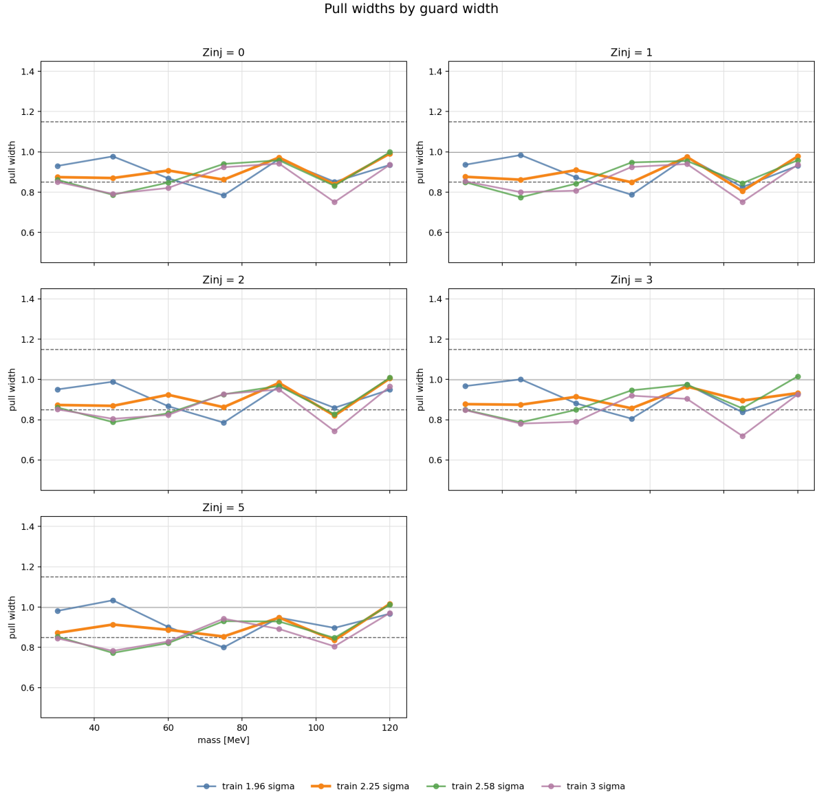
Figure 44: Signal-extraction pull widths from the same historical training-exclusion comparison. They test the reported uncertainty scale alongside the pull means in Fig. 43. The recovery, mean and width diagnostics informed the 2.25\sigma_m training choice; the subsequent extraction-geometry comparison is shown separately below.
