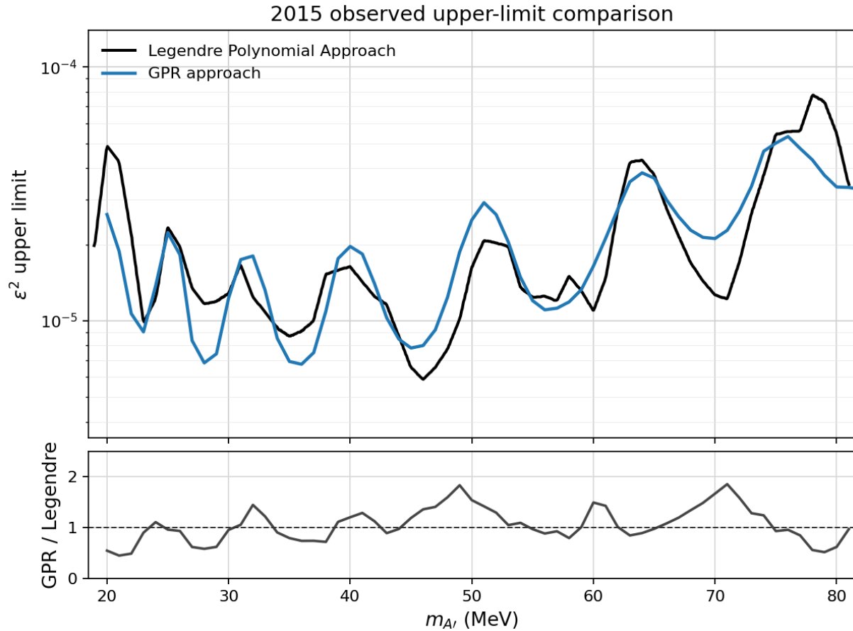
Figure 111: Restored historical 2015 observed 95% confidence-limit comparison from Appendix E of v4.9.7. The black “Legendre Polynomial Approach” curve is the corrected 2015 re-analysis digitized from Fig. 71 of the 2016 internal note; the blue curve is the earlier GPR comparison for the same full 2015 sample. The lower panel is the pointwise ratio of these saved curves, with median 0.99 and mean 1.06 over 20 MeV to 81 MeV. Both curves predate the current v5 settings. Their similar normalization scale does not establish coverage or absence of signal absorption.
