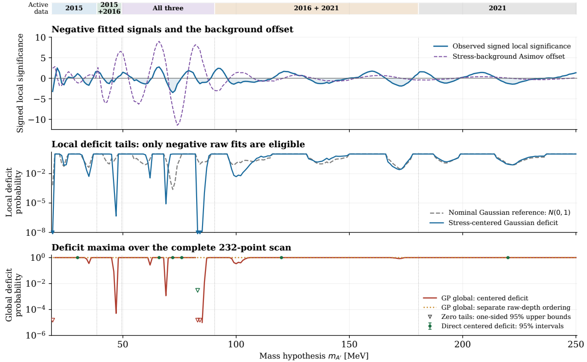
Figure 97: Profiled deficit scan. Top: observed signed local significance and the stress-background offset; shading marks negative fitted contributions. Middle: raw-root Gaussian reference and conditional Gaussian-response tails. Both assign one to nonnegative raw roots. Local triangles mark the 10^{-8} display floor. Bottom: two separate global orderings; triangles mark one-sided 95% zero-count bounds. Direct error bars are central 95% intervals.
