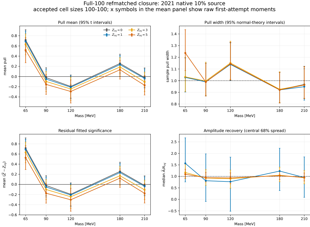
Figure 103: As in Fig. 102, for the native-10% ensemble. All cells retain 100 toys. The largest mean offset is at 65 MeV. The only accepted width outside 0.8–1.2 in the complete study is 1.237 for the 65 MeV, z = 5 cell; its normal-theory 95% interval is [1.086, 1.437].
