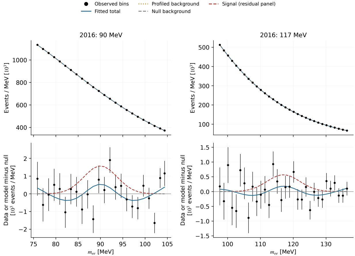
Figure 95: Traditional baseline fits to full 2016 data. At 90 and 117 MeV the nominal local coordinates are 1.998 and 1.525, with D/\text{dof} = 125.35/113 and 165.59/155 . The display sums five adjacent native bins to 1.25 MeV; any partial endpoint is retained. Counts, residuals and predictions are divided by each displayed width. Fits and probabilities still use the original 0.25 MeV bins. Both baseline positive roots are weaker than their GP values. Reducing the polynomial degree gives negative yields and larger deviances (Table 18). All alternatives are retained. Numerical convergence does not establish that a background describes the data; nominal local probabilities refer only to that model at the already selected mass.
