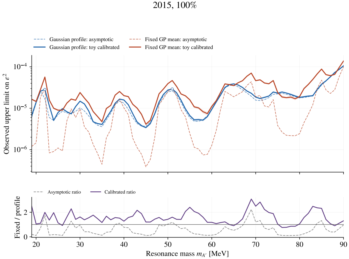
Figure 84: Observed asymptotic and calibrated 90% CL_s limits for 2015 using the two background treatments. Calibration envelopes cover the two stated generating shapes. Shading and open precision markers refer to finite Monte Carlo accuracy; they are not expected-limit bands.
