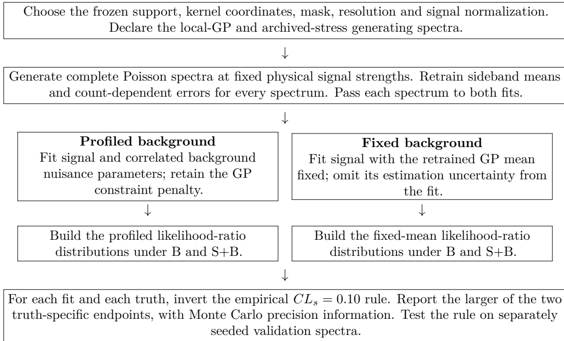
Figure 83: How the two background treatments are calibrated. Both branches receive identical spectra. The primary comparison uses two declared background truths for each method; it does not average the two methods or select whichever gives the tighter observed limit. B denotes background only and S+B denotes signal plus background.
