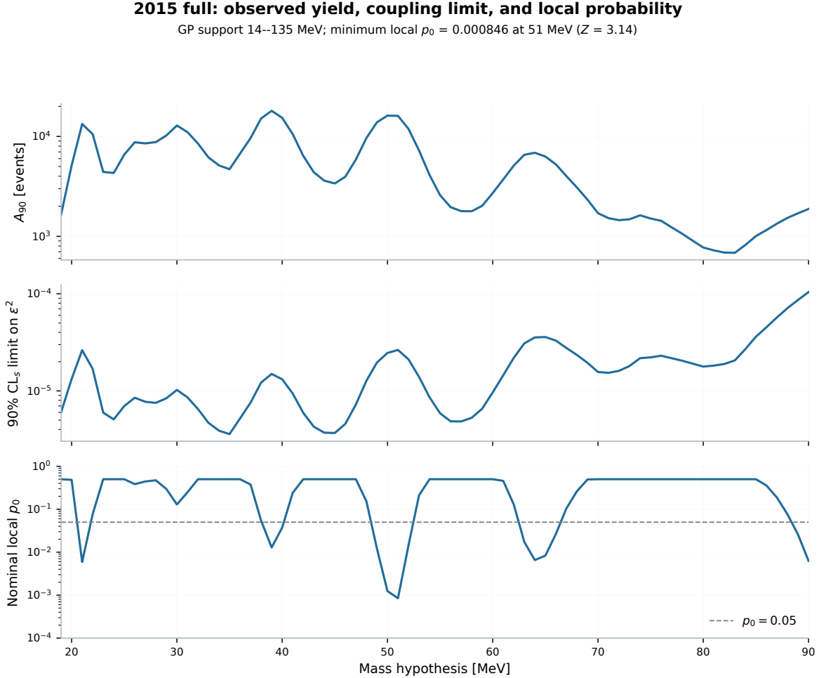
Figure 55: Observed 2015 full-sample scan on 19–90 MeV with 14–135 MeV GP support. From top to bottom: the 90% CL s full-template signal-yield upper limit A_{90} , the corresponding \epsilon^2 upper limit, and nominal local asymptotic p_0 . The same frozen released fits supply all panels. The dashed line marks p_0 = 0.05 ; no expected bands or look-elsewhere correction are included.
