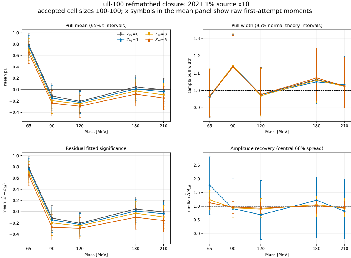
Figure 102: Full-100 refmatched closure for 1\% \times 10 . Every cell retains 100 accepted toys. The persistent positive 65 MeV pull means and the corresponding analytic-mean result are local stress-truth/model offsets; the other masses have near-unit widths and substantially smaller means. Crosses in the mean panel show raw first-attempt moments before the predeclared LML/reproducibility selection.
