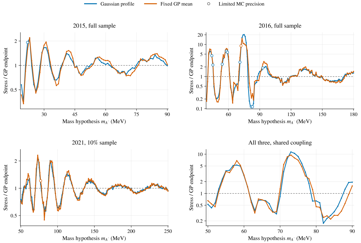
Figure 88: Ratio of the stress-truth to local-GP calibrated endpoint. Values above one indicate that the stress background controls the larger endpoint; values below one indicate that the local-GP control does. Open circles mark limited precision in at least one component, and gaps retain unavailable or censored ratios. This comparison diagnoses the chosen background family rather than certifying either member.
