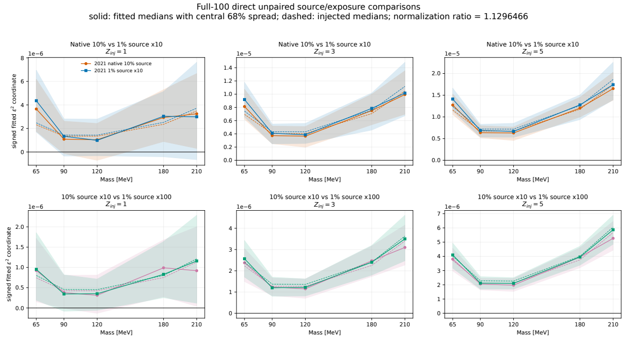
Figure 107: Direct full-100 comparisons between native 10% and 1% \times 10 (top) and between 10% \times 10 and 1% \times 100 (bottom). Solid curves and bands are fitted medians and empirical 16–84% spreads; dashed curves are injected medians. The source functions are fitted independently and the cross-source ensembles are unpaired. Their expected-normalization ratio is 1.1296466 in both comparisons, so differences combine source/selection shape and normalization and are not pure exposure effects or paired tests. The ribbons are descriptive coordinate spreads, not expected-limit bands.
