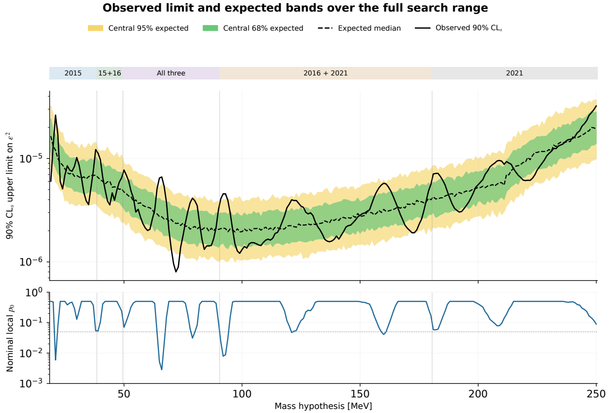
Figure 52: Complete 19–250 MeV observed search, with the preassigned active datasets shown above the curves. The upper panel shows 90% CL s limits and the median, central 68% and central 95% ranges of the original 300 conditional background-only toys per mass. The lower panel adds the unchanged fixed-mass asymptotic p_0 . The observed polyline connects every adjacent tested mass, including membership transitions; no numerical endpoint is changed by those connections. The physical visible-branching correction is applied once above the dimuon threshold. These are pointwise bands; 2016-inclusive values retain the numerical exception.
