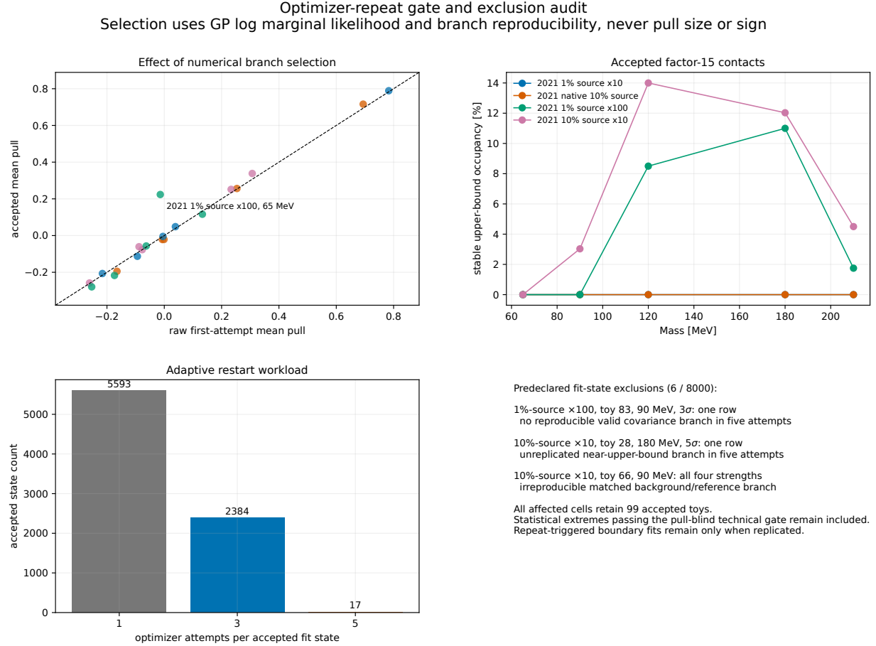
Figure 99: Optimizer-repeat gate and exclusion audit. The upper-left panel compares zero-signal means from the raw first attempts with the accepted LML-selected states; the visibly repaired 1\% \times 100 , 65 MeV point is numerical rather than a pull-based deletion. The upper-right panel reports accepted factor-15 contacts. The lower-left panel gives the adaptive attempt workload, and the lower-right panel lists all six excluded states. Statistical extremes that pass the pull-blind technical gate remain in the headline summaries; repeat-triggered boundary solutions are retained when replicated.
