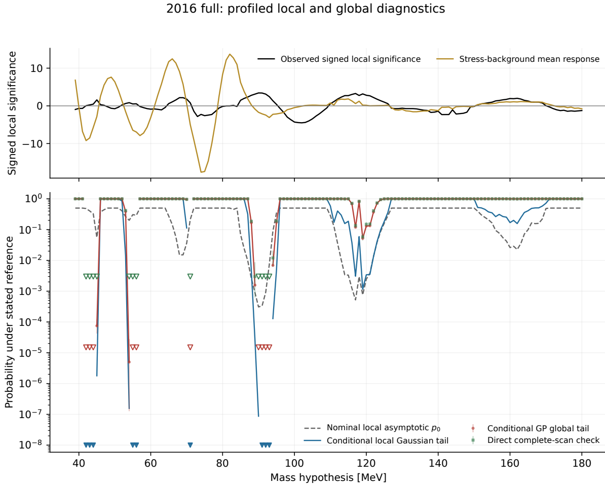
Figure 79: Profiled 2016 conditional global study. The leading principal-ordering threshold at 42 MeV has no exceedance in either ensemble. The corresponding one-sided 95% bounds are 1.498 \times 10^{-5} for 200,000 GP fields and 0.002991 for 1,000 direct scans. They are finite-sampling bounds under the specified models, not a resolved rare particle probability. A qualified final 2016 global result remains outstanding.
