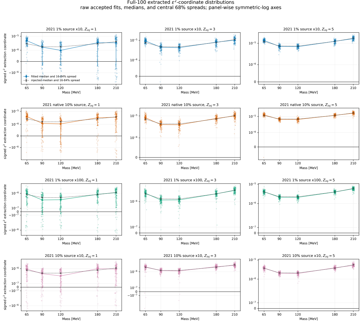
Figure 106: Signed \varepsilon^2 extraction-coordinate distributions for the 1-, 3-, and 5- \sigma_A injections. Points are all accepted fits; solid summaries are medians and empirical 16–84% intervals, while dashed summaries describe the toy-local injected coordinates. Panel-wise symmetric-log axes retain negative fitted values and broad 1- \sigma fluctuations. Because both K_{stm} and \sigma_{A,stm}^{\text{ref}} are toy-local, the injected coordinates are distributions. These are extraction diagnostics, not limits, physical negative couplings, or expected bands.
