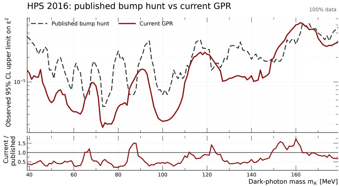
Figure 112: Saved 2016 observed 95% confidence-limit comparison from 5 August 2026, using the full already analyzed 2016 sample. The published reference uses the polynomial CL_s method; the curve labeled “current” in this archived graphic means the then-current v4.1 factor-12 GPR candidate. It does not mean the v5.0.1 configuration. The lower panel gives the pointwise observed GPR/published ratio, whose median is 0.5579 over 141 matched masses. This was an observed, asymptotic comparison with fixed reviewed kernel coordinates, no new toys, and no expected-limit bands.
