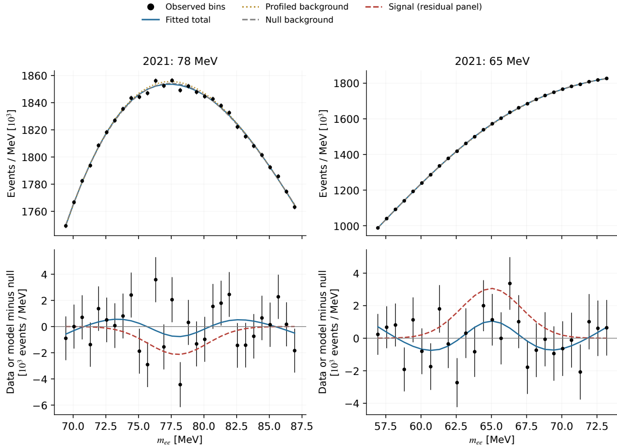
Figure 96: Traditional baseline fits to the released 2021 10% sample. At 78 and 65 MeV the signed local coordinates are -1.350 and 1.960 , with D/\text{dof} = 29.16/24 and 17.36/22 . Original 0.625 MeV bins are retained and displayed as counts per MeV. The 78 MeV feature becomes a deficit for every specified conventional fit. The 65 MeV baseline remains a modest positive excess. Its degree-two alternative gives a very large positive root but D/\text{dof} = 28.10 , showing a severe background-model failure (Table 18). Counting bars and the fitted Gaussian component are visual aids, not independent residual significances. No additional 2021 data were opened.
