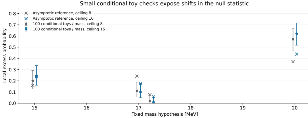
Figure 117: Toy upper-tail fractions with central 95% binomial intervals, compared with the asymptotic local reference. The two ceiling choices have their own conditional generating backgrounds. These small plug-in ensembles assess this fitting procedure under those means; they are not independent background validation or a final p-value calibration.
