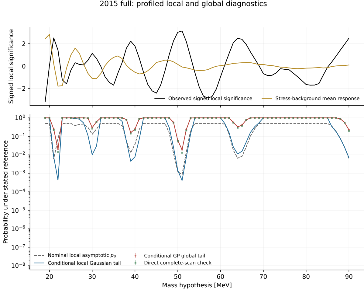
Figure 78: Profiled 2015 local and conditional GP global probabilities. The study used ten complete pilot scans, 1,000 independent validation scans and 200,000 GP fields. The principal global probability at the selected 51 MeV threshold is 0.018985 in the GP approximation; 13 of 1,000 direct scans exceed that threshold. The precision of either ensemble and the generating-background assumptions remain explicit.
