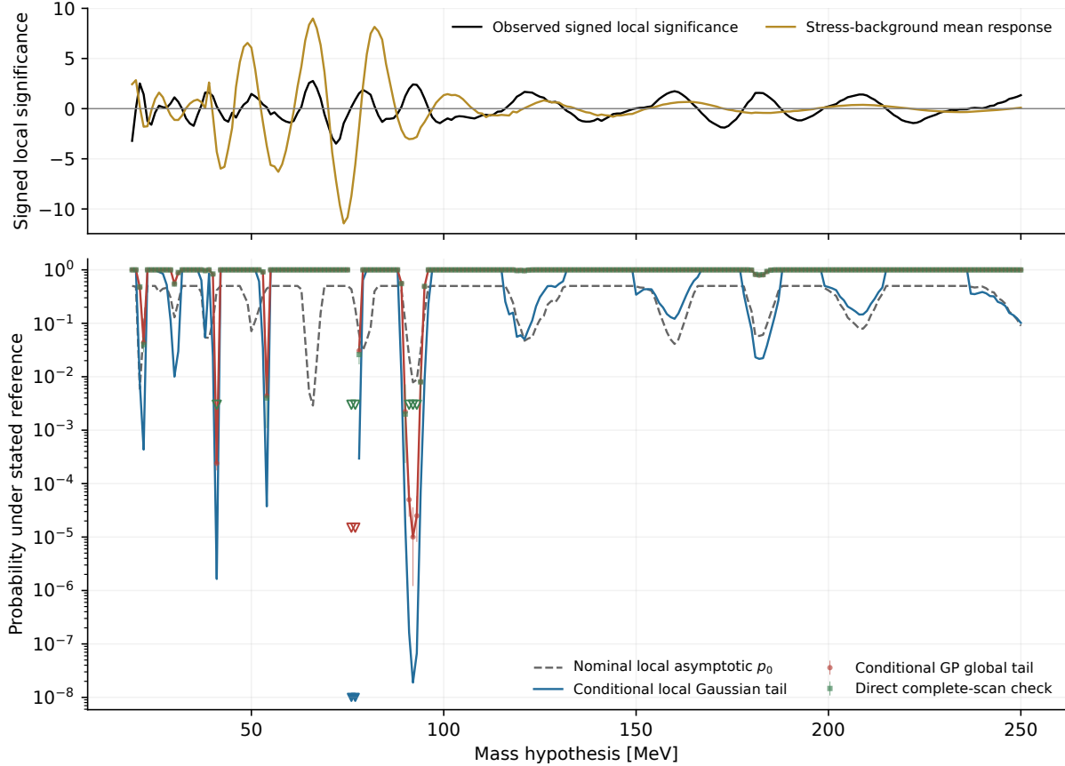
Figure 81: Full combined search with the same profiled local and conditional global probability conventions. The upper panel shows the observed local coordinate and the stress-background offset so that an extreme centered tail can be traced to its reference. Open downward triangles are one-sided 95% Monte Carlo upper bounds for zero counts; triangles at the local plotting floor mark analytic values below 10^{-8} . The raw and centered orderings are separate tests.
