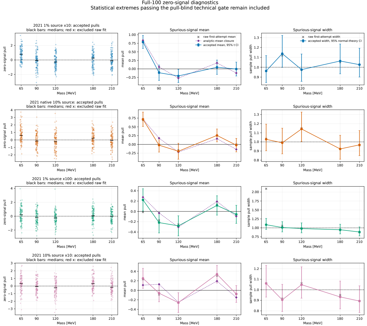
Figure 100: Full-100 spurious-signal study. Each row corresponds to one ensemble. The left panels show every accepted zero-signal pull and its median; the middle panels show raw first-attempt means, accepted means with 95% Student- t intervals, and the deterministic analytic-mean closure; the right panels show accepted sample widths with 95% normal-theory intervals. Red crosses mark excluded raw fit states where present. No accepted pull is clipped. The common mass dependence between analytic-mean and ensemble results diagnoses stress-truth/model closure rather than a statistical outlier.
