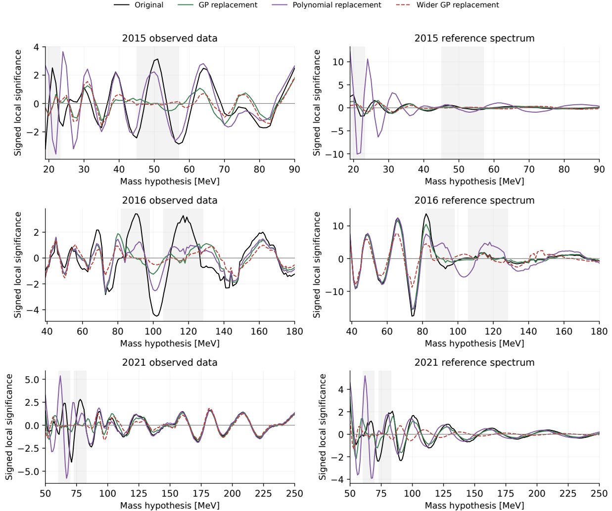
Figure 93: Both-hole replacements in observed counts (left) and the reference spectrum (right). Green: primary GP mean. Purple: exponential-polynomial fill. Dashed red: wider GP holes. The reference ordinate a_m = r_m(B) is the fitted root, not the background event rate. Gray shading marks primary holes; wider holes extend beyond it. All outcomes remain visible, including unsuccessful interpolation. No altered spectrum supplies a new observed-data probability.
