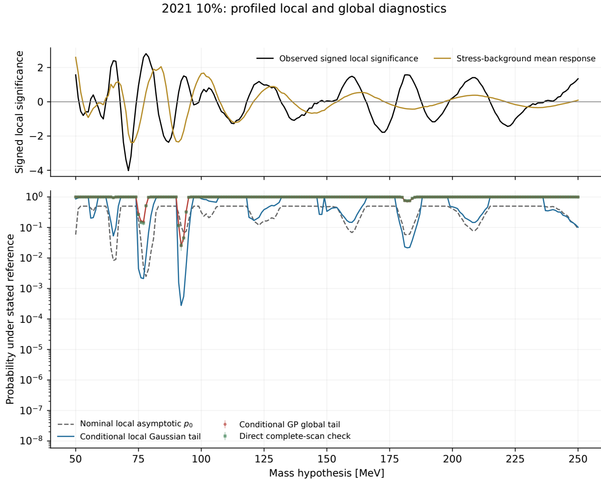
Figure 80: Profiled global study for the released 2021 10% sample. The principal ordering selects 92 MeV and gives GP global probability 0.02519, with 26 of 1,000 independent direct scans above the threshold. This selection differs from the largest raw positive fitted signal. Qualification of the generating background and the final analysis choices remains required for a final particle-global interpretation.
