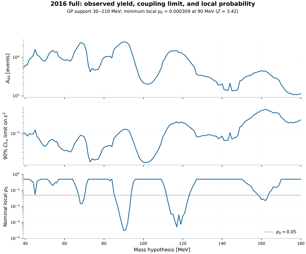
Figure 56: Corresponding observed 2016 full-sample scan on 39–180 MeV with 30–210 MeV GP support. The panels show the full-template A_{90} , \epsilon^2 limit, and nominal local asymptotic p_0 . The existing 2016 numerical and generating-source qualifications remain applicable.
