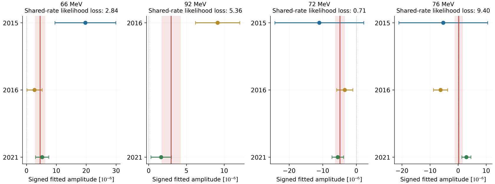
Figure 82: Separate campaign coupling estimates and local curvature errors compared with the common rate. The likelihood loss quantifies how much the local fit improves when each year can choose its own amplitude. The 66 MeV fit has positive contributions from all three years; the 92 MeV separate rates differ more visibly. These selected comparisons and local errors are not post-selection compatibility tests.
