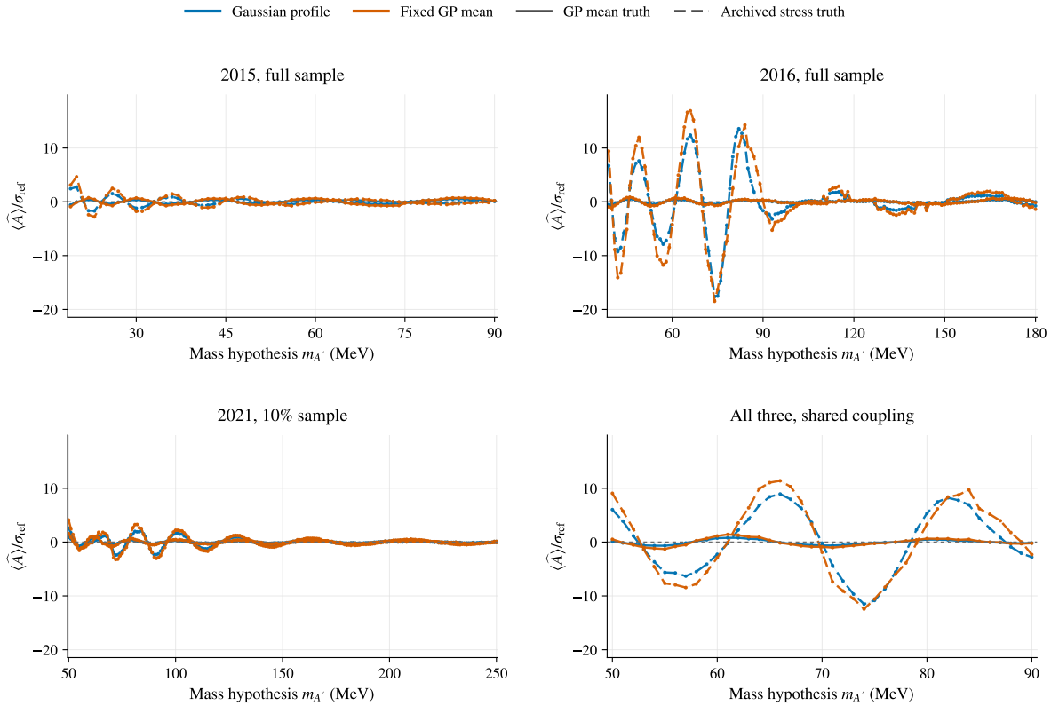
Figure 90: Mean fitted background-only yield in units of one fixed reference error, from 500 independently generated spectra per mass and truth. Solid and dashed curves distinguish the two backgrounds. Pointwise 95% intervals describe Monte Carlo precision on each mean. This normalization differs from a pull using each toy’s random fitted error; the plot does not measure a bias in observed data.
