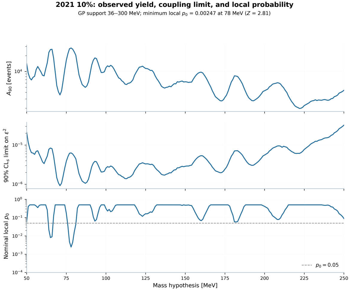
Figure 57: Corresponding observed 2021 10% scan on 50–250 MeV with 36–300 MeV GP support. The panels show the full-template A_{90} , minimal-visible \epsilon^2 limit, and nominal local asymptotic p_0 . Above the dimuon threshold the inherited branching correction enters the coupling conversion once; it does not change the visible electron-pair yield or local probability.
