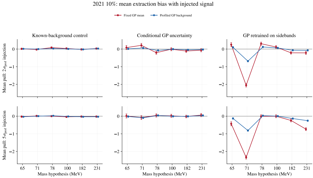
Figure 37: Mean signal-extraction pull for injections of 2\sigma_{\text{ref}} and 5\sigma_{\text{ref}} , where the profiled Fisher reference error fixes the event yield before generation. Each mass–strength–background cell contains 500 spectra, shared by the fixed and profiled methods. Pull denotes (\hat{A} - A_{\text{true}})/\hat{\sigma}_A ; bars are Monte Carlo errors on its mean. At 71 MeV, a signal injected at 71 MeV into the retrained smooth-background construction has mean pull -2.33 for the fixed fit and -0.81 for the profiled fit at the stronger injection. Profiling reduces this conditional offset below one fitted standard error, but the associated exclusion test still fails. Adapted from Fig. 9 of the v4.9.13 calibration report.
