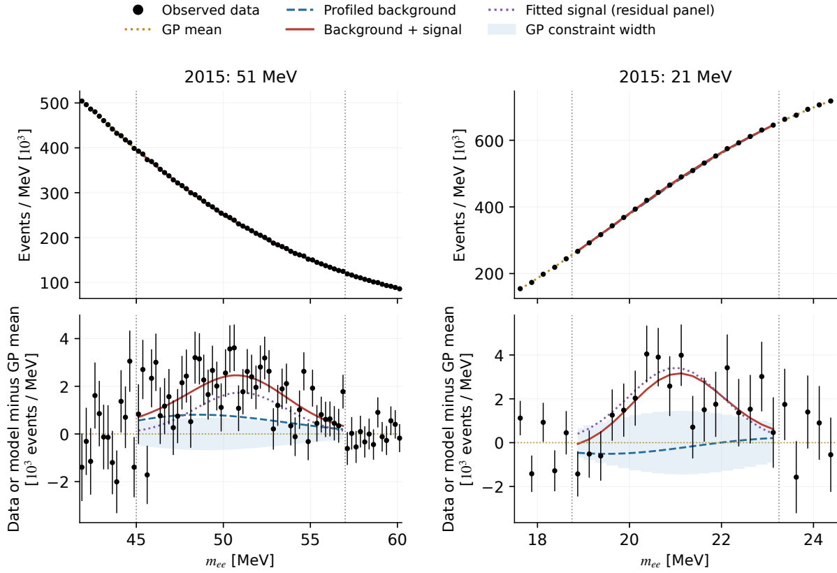
Figure 70: The two leading separated 2015 excesses at 51 and 21 MeV. The 21 MeV feature lies close to the search endpoint and has strong background-model dependence in the traditional-fit cross-check. Bars show counting error only; residual shading shows the zero-centered GP constraint width, not fitted-background or total residual uncertainty.
