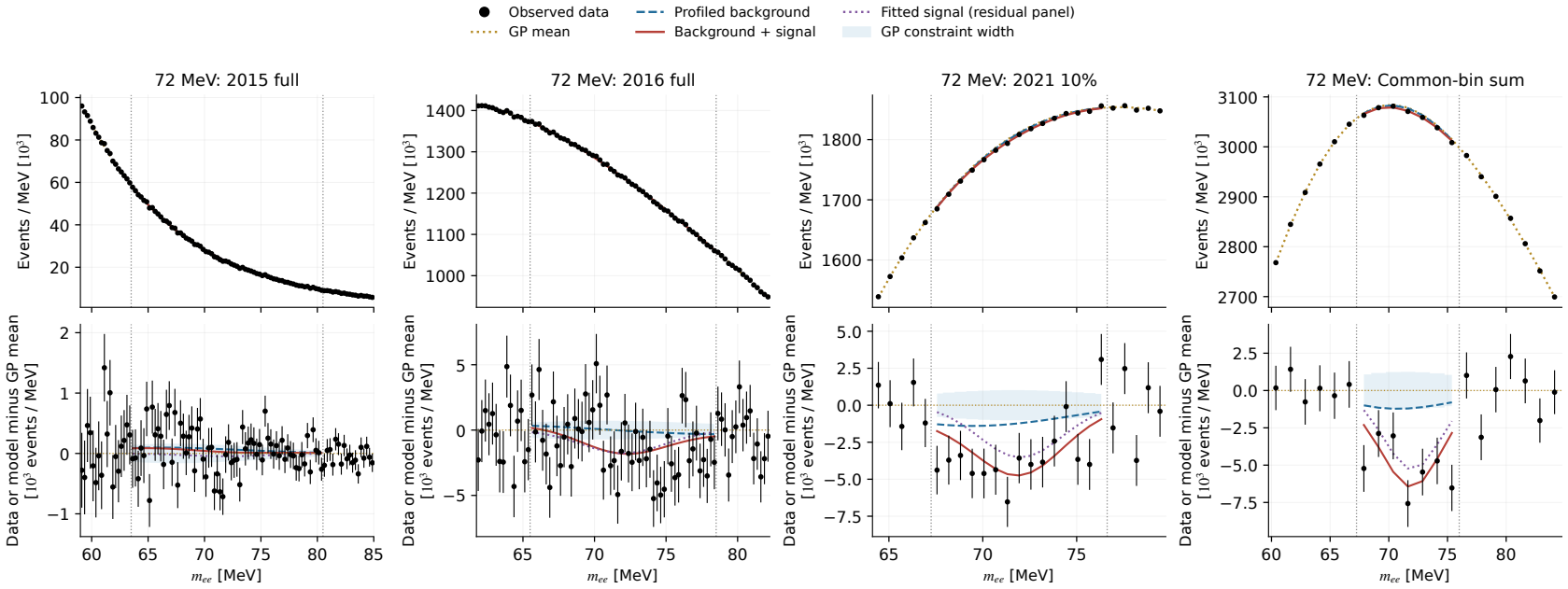
Figure 69: The deepest combined observed deficit at 72 MeV has signed local significance -3.49 and an auxiliary amplitude \hat{\epsilon}^2 = -4.88 \times 10^{-6} . The negative signal template describes missing counts relative to the fitted background. Bars show counting error only; residual shading shows the zero-centered GP constraint width, not fitted-background or total residual uncertainty.
