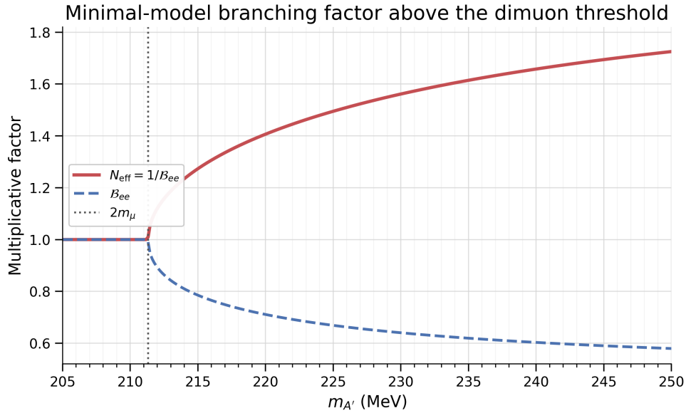
Figure 35: Minimal-model branching factor used to reinterpret electron-channel \varepsilon^2 limits above the dimuon threshold. The red curve shows N_{\text{eff}}^{\text{BR}} = 1/\mathcal{B}(A' \rightarrow e^+e^-) and the blue dashed curve shows \mathcal{B}(A' \rightarrow e^+e^-) .
