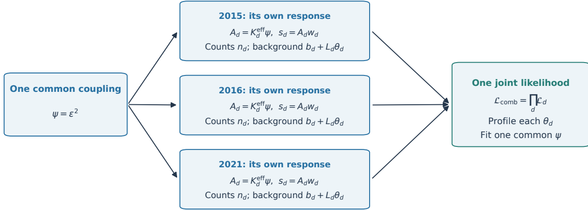
Figure 34: One coupling predicts a campaign-specific signal through its normalization and resolution. Each campaign retains its own counts and correlated background constraint; the likelihoods are multiplied and fitted with one common coupling. Only datasets whose declared search contains the tested mass contribute.
