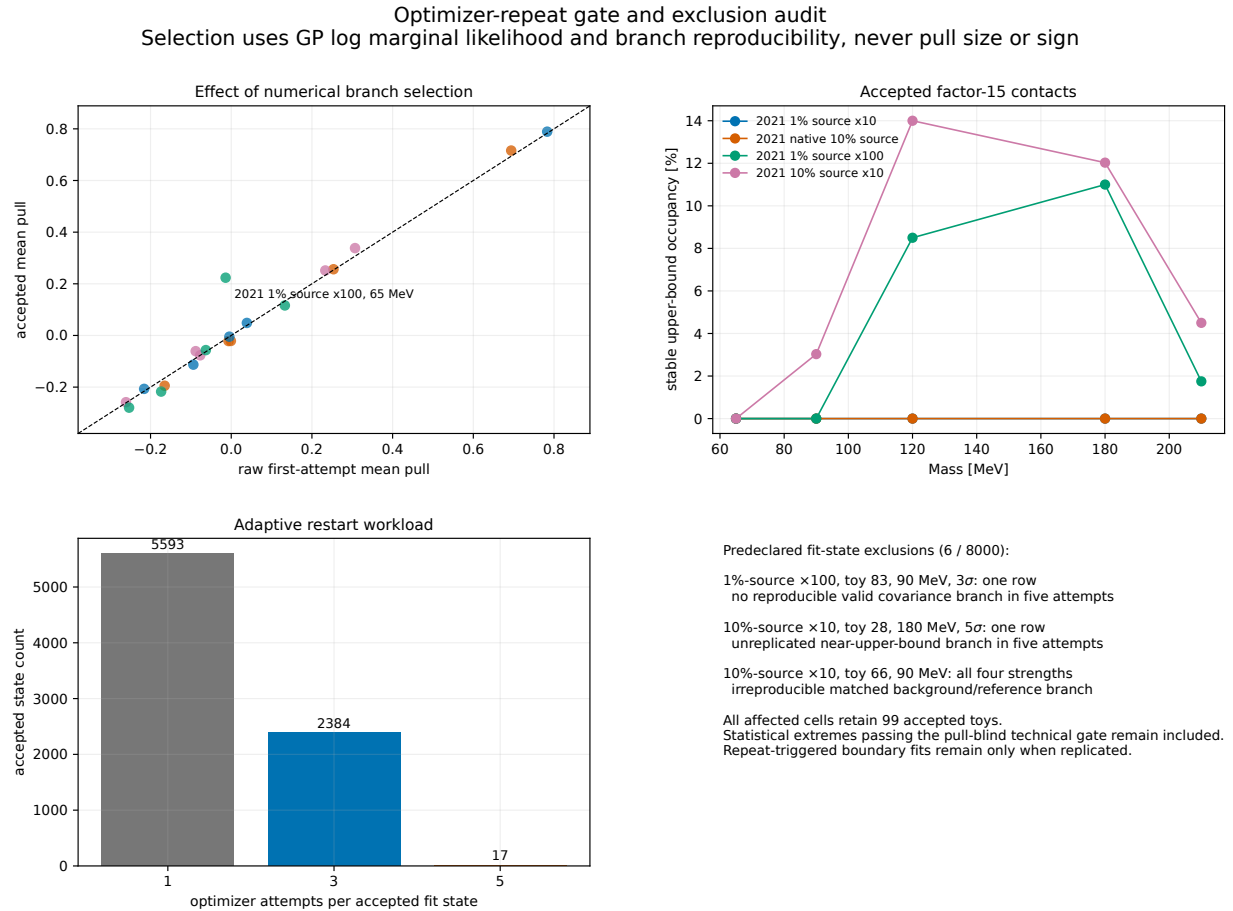
Figure 102: Optimizer-repeat gate and exclusion audit. The upper-left panel compares zero-signal means from the raw first attempts with the accepted LML-selected states; the visibly repaired 1\% \times 100 , 65 MeV point is numerical rather than a pull-based deletion. The upper-right panel reports accepted factor-15 contacts. The lower-left panel gives the adaptive attempt workload, and the lower-right panel lists all six excluded states. Statistical extremes that pass the pull-blind technical gate remain in the headline summaries; repeat-triggered boundary solutions are retained when replicated.
