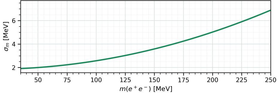
Figure 18: Mass-resolution parameterizations used by the analysis over the adopted scan ranges. The 2016 scan ends at the polynomial boundary of 180 MeV, so its configured high-mass continuation is not used. The 2021 panel shows the target-constrained V0 parameterization after multiplication by the TC smearing scale s_{\text{TC}} = 2.186/1.745 \simeq 1.25 and extended to 250 MeV.
