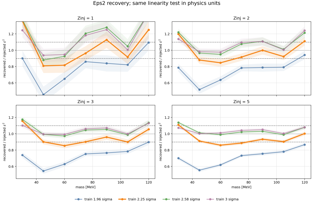
Figure 41: Historical 2015 matched-reference training-exclusion comparison, restored from the v4.9.7 validation archive. The extraction width was 1.64\sigma_m , while the training exclusion was varied through 1.96, 2.25, 2.58 and 3.00\sigma_m . Recovered coupling coordinates are divided by the injected values. The 2.25\sigma_m choice substantially reduces under-recovery relative to the narrow guard, while avoiding the larger uncertainty cost of wider exclusions. The plotted spreads belong to the archived ensembles, not a new confidence-limit calibration.
