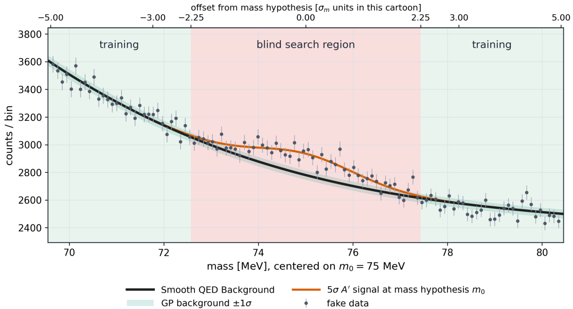
Figure 40: Selected 2.25\sigma_m blind and training-exclusion geometry. The GP is trained outside the widened interval, while all bins inside it enter the local signal-plus-background likelihood. This retains the signal tails for extraction without allowing those same bins to influence the sideband fit.
