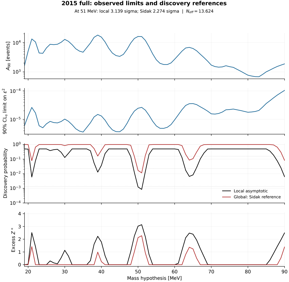
Figure 55: Observed 2015 full-sample scan on 19–90 MeV with 14–135 MeV GP support. From top to bottom: the 90% CL s full-template signal-yield upper limit A_{90} , the corresponding \epsilon^2 upper limit, discovery probabilities, and aligned Z^+ values. The local asymptotic reference is black and the Sidak reference is red, with N_{\text{eff}} = 13.624 . At 51 MeV they give Z = 3.139 and Z_{\text{Sidak}} = 2.274 . The same frozen released fits supply all panels. The Sidak reference is distinct from the conditional GP global calculation in Section 6.11.
