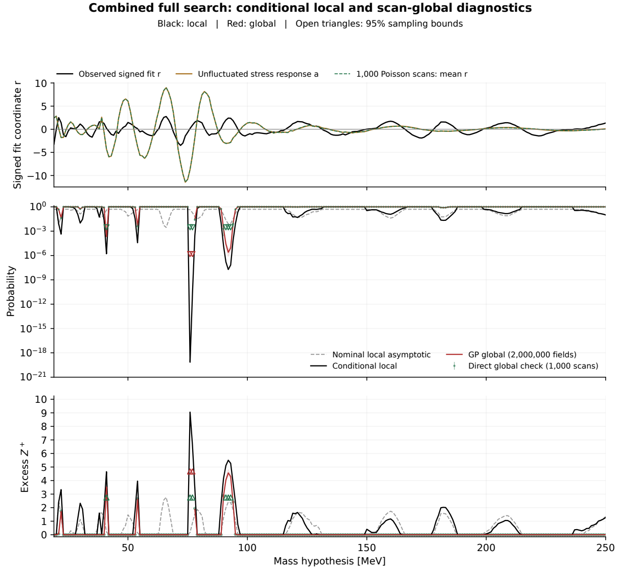
Figure 81: Full combined search with observed and stress-reference responses above, probabilities in the middle, and Z^+ below. Black is conditional local and red conditional GP global; this correlated-field global is different from the Sidak global reference in Figure 52. The GP continuation totals 2,000,000 complete fields and leaves 76 and 77 MeV at zero exceedances. Open triangles give one-sided 95% bounds: p < 1.498 \times 10^{-6} or Z > 4.671 for the GP model, and the weaker direct-scan bounds at 1,000 scans. The finite local Gaussian tails are shown without the former 10^{-8} plotting cutoff. Z^+ = 0 for probabilities of at least one half; the signed fit above retains deficit information. These are conditional diagnostics.
