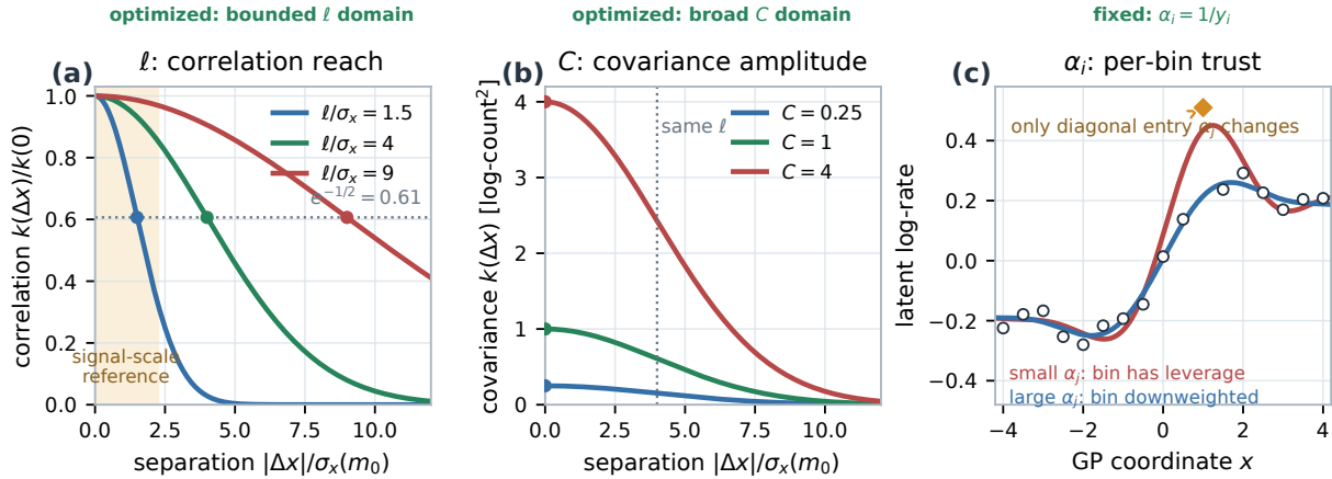
Figure 26: Roles of the three quantities in the GPR covariance. Panel (a) shows the normalized RBF correlation for three illustrative values of \ell/\sigma_x(m_0) ; at a separation equal to \ell , every curve has correlation e^{-1/2} \simeq 0.61 . The length scale sets the correlation range. Panel (b) varies C at fixed \ell . It changes the covariance amplitude, with pointwise prior standard deviation \sqrt{C} , without changing the normalized correlation range. Panel (c) holds the kernel fixed and changes one diagonal variance \alpha_j , thereby changing that bin's statistical weight. We optimize C and \ell on the sidebands and fix \alpha_i from the count-based variance rule. The curves are schematic.
