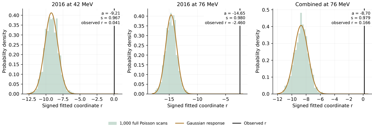
Figure 82: Representative background-only distributions from the saved 1,000 complete Poisson scans. Green histograms show the signed fitted coordinate, gold curves the unfluctuated-response Gaussian approximation, and black lines the observed fit. These panels show why the apparently large centered scores at 2016 42 MeV and combined 76 MeV can coexist with nearly zero raw observed fits. At 2016 76 MeV the observed fit is negative and is excluded by the positive-fit gate. Agreement of the histograms with the gold curves tests the approximation under that reference, not the physical correctness of the reference spectrum.
