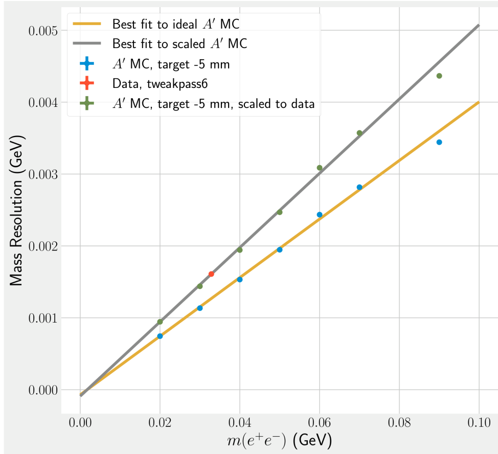
Figure 14: 2015 mass-resolution parameterization from scaled A' MC and Møller data [31]. The Møller point anchors the absolute detector response in data, while the scaled A' simulation supplies the mass dependence across the search window. Because the prompt dark-photon width is negligible, this curve directly sets the resonance width assumed in the search and therefore the local background entering the limit.
