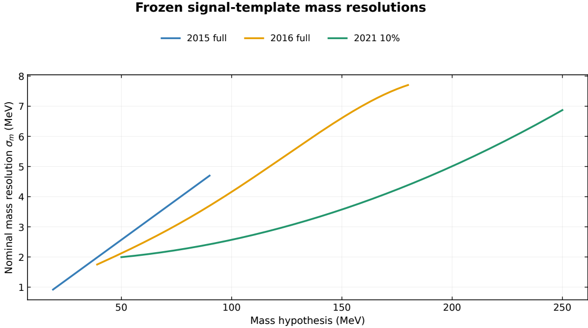
Figure 13: Frozen nominal mass-resolution parameterizations over the current search intervals. These inputs set the signal-template widths, moving fit windows and resolution-scaled kernel constraints. Their signal-width variations are examined in Section 6.8.
