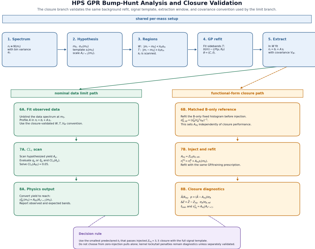
Figure 39: Analysis and validation flow. In the data path, sidebands around each mass hypothesis train the GP and the blinded bins enter the signal-plus-background likelihood. In the validation path, a smooth source-fitted mean is Poisson fluctuated, a known signal may be added, and the complete GP fit and extraction are repeated. The zero-injection ensemble tests spurious signal; nonzero injections test signal recovery and uncertainty calibration. These are extraction-closure tests, not confidence-limit coverage or a scan-wide significance calibration.
