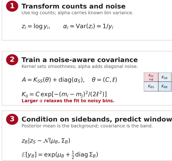
(a) Log-count transform, noise-aware covariance training, and window prediction. The filled covariance boxes indicate the sideband-sideband, sideband-blind, and blind-blind kernel blocks used when conditioning the GP.
