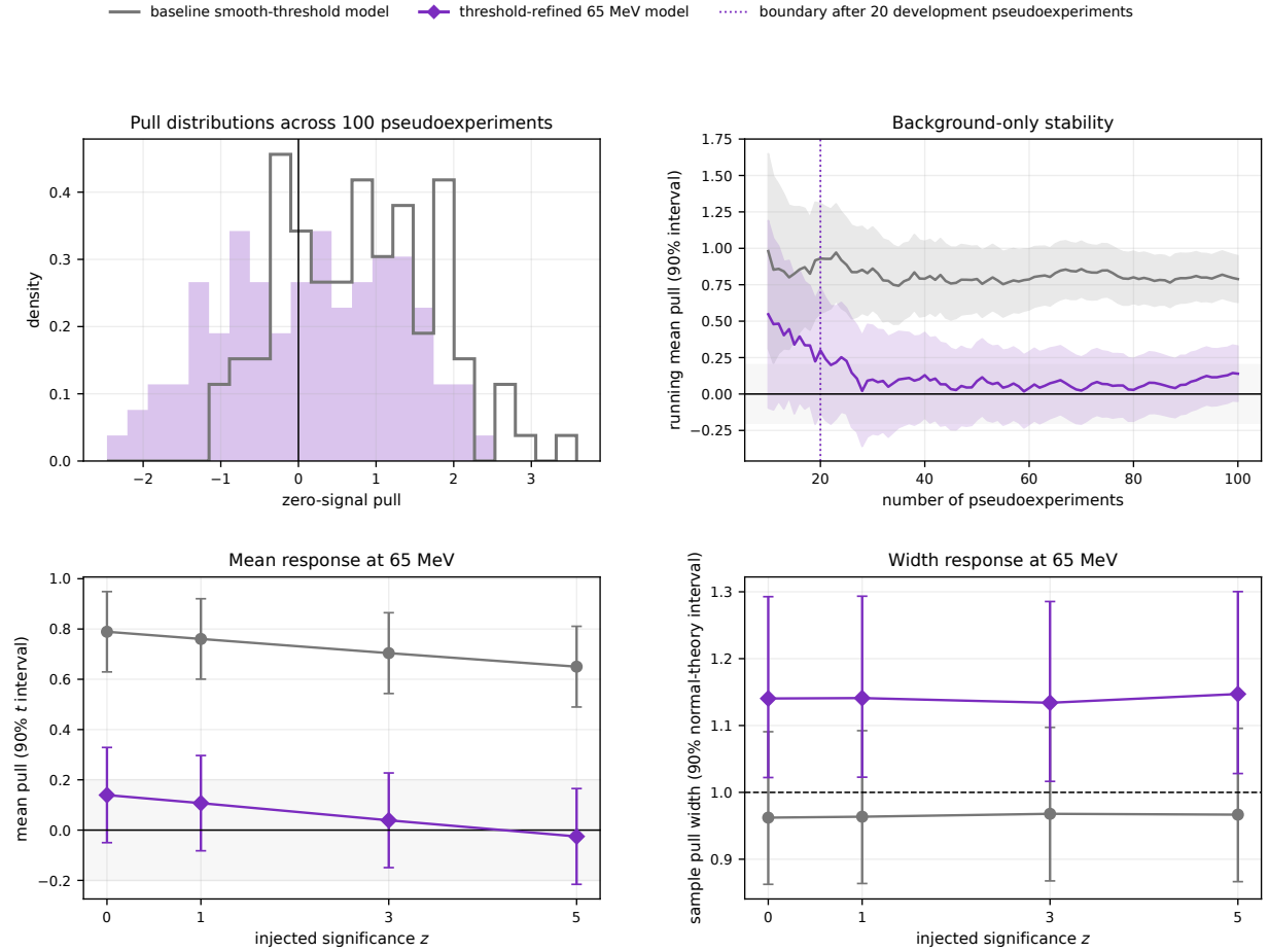
Figure 48: Targeted 1\% \times 10 test at 65 MeV, comparing the threshold-refined and baseline smooth-threshold models. The upper panels show the zero-injection pull distribution and the running mean; the lower panels show the mean and width across the correlated z = 0, 1, 3, 5 extractions. Mean intervals are two-sided 90% Student- t intervals and width intervals are exact normal-theory 90% chi-square intervals. The full sample contains the 20-background development subset; the independent continuation in Table 8 gives the same qualitative result.
