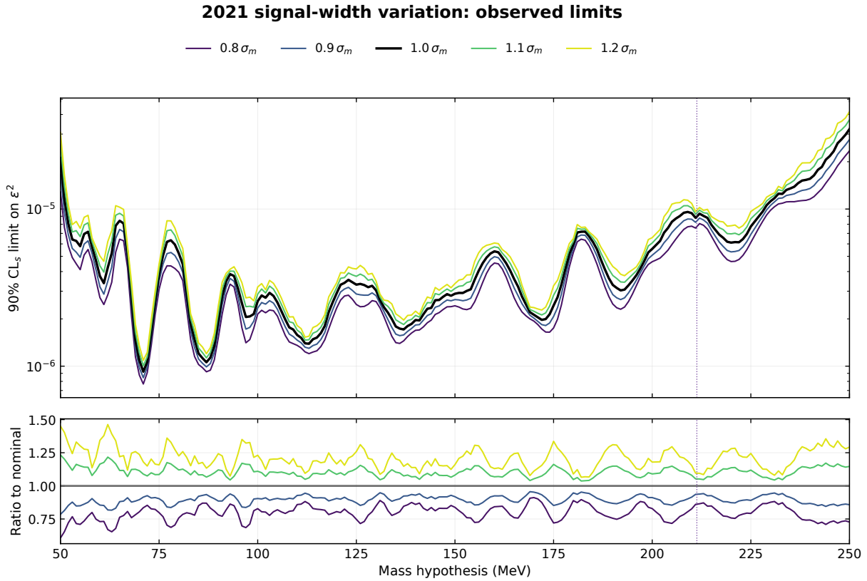
Figure 65: 2021 observed 90% CL s limits for the five signal-template widths, with ratios to the nominal limit below. Every curve uses the same archived GP prediction and yield conversion. The visible-branching correction is common to all curves and cancels in the ratios. The plots retain all 1,005 saved limits.
