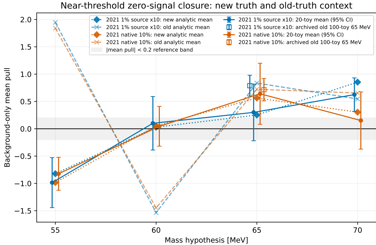
Figure 112: Historical 20-background near-threshold closure. Points carry 95% Student- t intervals; deterministic responses to the old and new analytic means expose the truth-shape dependence. The known 65 MeV response improves in the 1%-source test, while neighboring offsets remain. The later 100-background replacement results in the main text use their own identified truth and support; they are not pooled into these curves.
