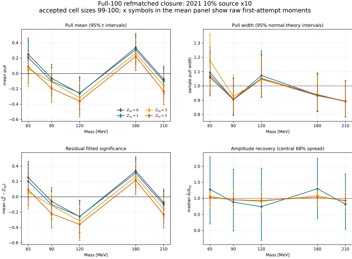
Figure 108: As in Fig. 105, for 10\% \times 10 . The four 90 MeV cells and the 180 MeV, z = 5 cell retain 99 toys; all others retain 100. The repeat gate repairs the dramatic 65 and 180 MeV optimizer branches seen in the v4.5 pilot without discarding those background pseudoexperiments. Among 1995 accepted fits, 134 stably contact the factor-15 upper bound.
