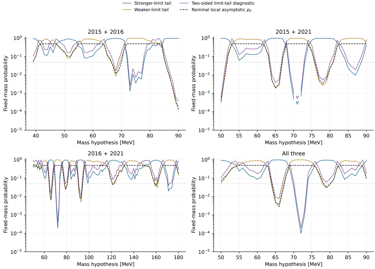
Figure 64: The same empirical limit-tail diagnostics for the pairwise and all-three combinations. Finite estimates and zero-count bounds remain visually distinct. Additional sampling can improve the precision of these conditional diagnostics, but cannot establish physical background validity or a discovery probability.
