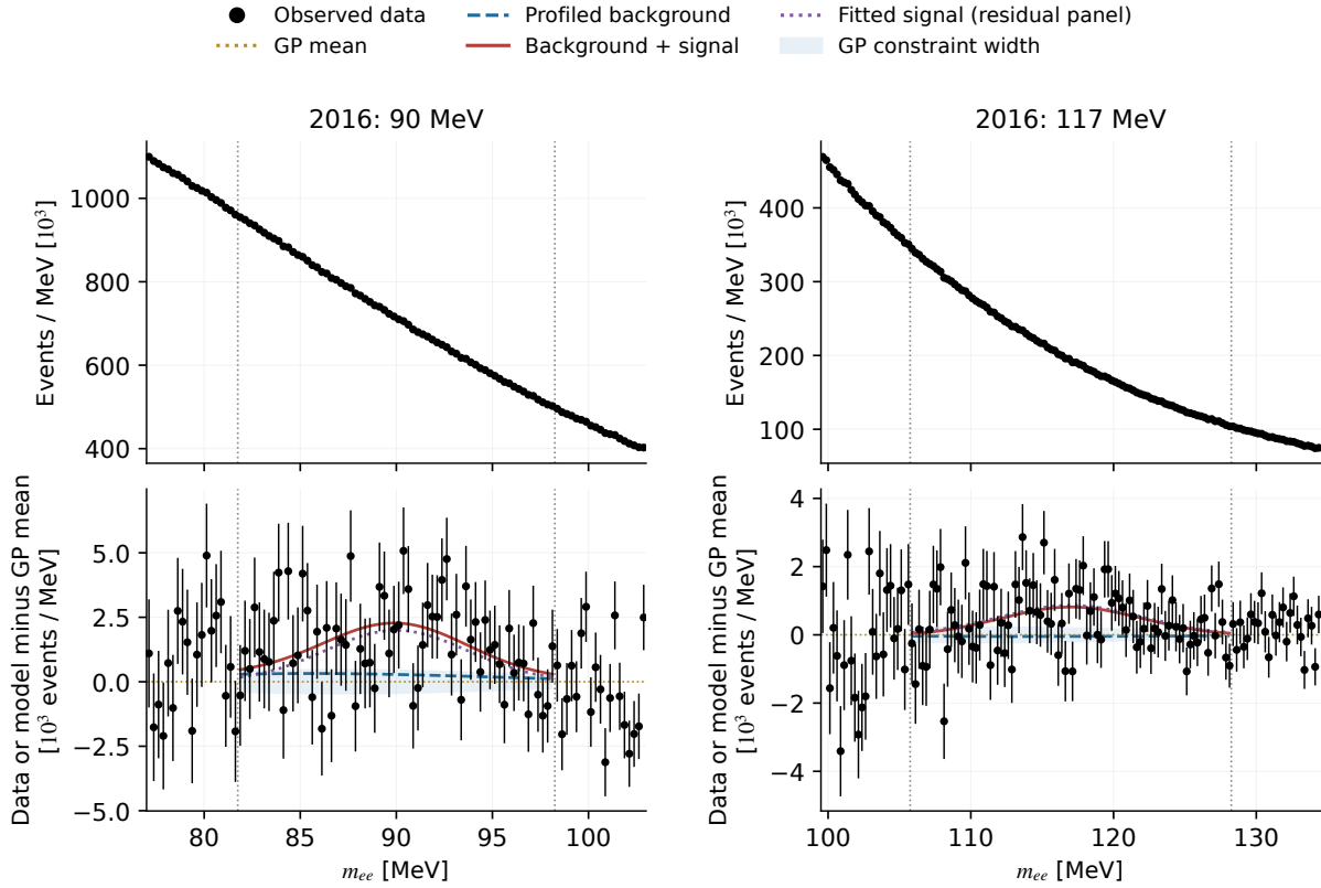
Figure 71: The leading separated 2016 excesses at 90 and 117 MeV. These fits retain the inherited 2016 numerical and background-source qualifications. Bars show counting error only; residual shading shows the zero-centered GP constraint width, not fitted-background or total residual uncertainty.
