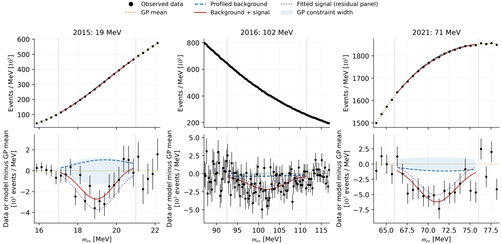
Figure 73: Individual deficit extractions at 19, 102 and 71 MeV in 2015, 2016 and 2021. The first is a search endpoint. Bars show counting error only; residual shading is the zero-centered GP constraint width, not fitted-background or total residual uncertainty. These are local background diagnostics. The joint deficit scan is retained in Appendix D.
