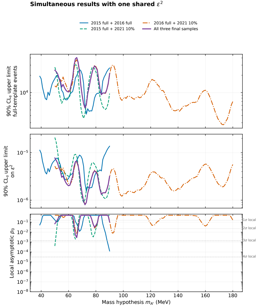
Figure 58: Observed shared- \varepsilon^2 results for the three pairwise combinations and the all-three overlap. For visual alignment, the top coordinate expresses the shared-coupling limit as the total compatible signal yield summed over the active campaigns. The middle panel gives the 90% bounded, piecewise-asymptotic \text{CL}_s upper limit on \varepsilon^2 , and the bottom panel gives the local asymptotic p_0 . No expected-limit bands are shown.
