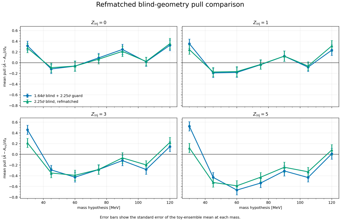
Figure 45: The subsequent matched-reference comparison of two extraction geometries in the same 2015 functional-form study. Both exclude training bins out to 2.25\sigma_m ; one retains a 1.64\sigma_m extraction and a separate guard, while the other fits all bins inside 2.25\sigma_m . The z = 0, 1, 3, 5 pull means and widths show similar conditional behavior. Together with the retained signal tails, this supported the widened blind/extraction window. Historical numerical values are unchanged.
