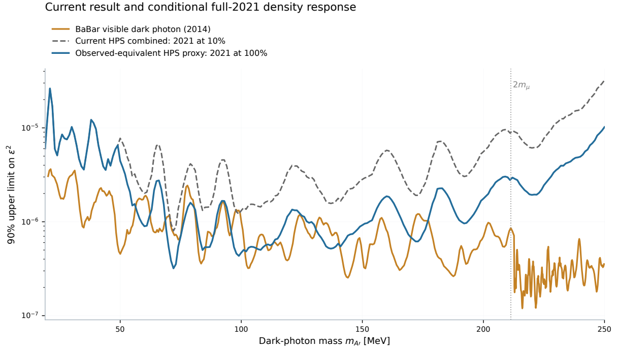
Figure 54: Current observed 90% upper limits and the conditional full-2021 density-response proxy compared with the published BaBar visible-dark-photon observed 90% contour [5]. The gray dashed curve is exactly the current maximal-available-dataset HPS result over 19–250 MeV. The blue curve applies Eq. (102) to its current observed normalization densities. It retains present fluctuations and is neither expected sensitivity nor a future observed limit or a fit to full-2021 data. HPS and BaBar use different statistical constructions. The inherited dimuon correction and 2016 qualifications remain applicable.
