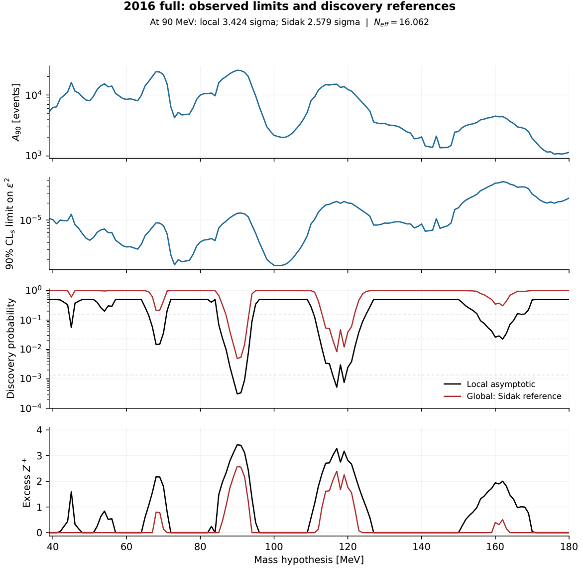
Figure 56: Corresponding observed 2016 full-sample scan on 39–180 MeV with 30–210 MeV GP support. The panels show the full-template A_{90} , \epsilon^2 limit, discovery probabilities, and aligned Z^+ values. Black is local and red is the Sidak reference with N_{\text{eff}} = 16.062 ; their values at 90 MeV are 3.424 and 2.579. The existing 2016 numerical and generating-source qualifications remain applicable.
