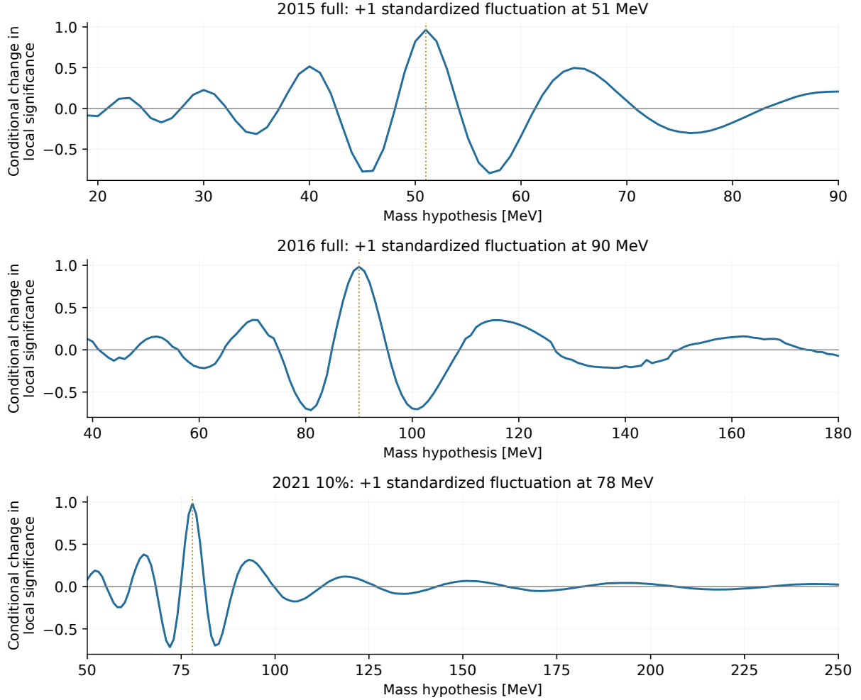
Figure 76: Conditional changes in the local-significance coordinate following a one-standard-deviation field fluctuation at 51 MeV in 2015, 90 MeV in 2016 and 78 MeV in 2021. The curves are s_m R_{m,m_0} , with each archived offset removed. Positive and negative lobes show the scale and sign of correlated fluctuations. These are Gaussian conditional means, not injected particles, probabilities of observed echoes, or independent significance gains.
