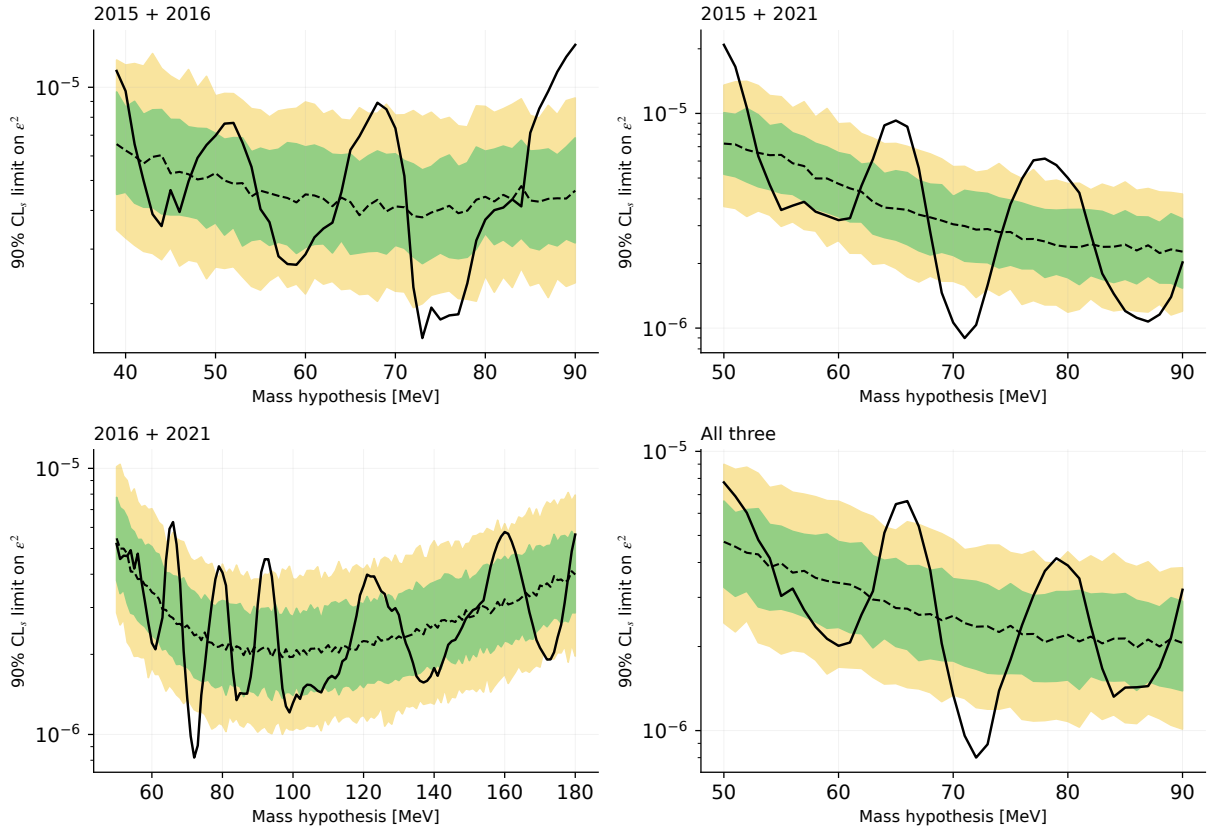
Figure 61: Pairwise and all-three results with the same conditional 300-toy pointwise bands. Comparisons at a given mass use paired constituent draws. Correlation between these panels does not supply correlation between separate mass hypotheses.
