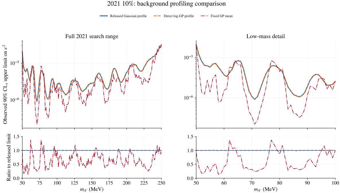
Figure 36: Controlled comparison of observed 2021 10% upper limits using the nominal correlated Gaussian background profile, a positive log-GP profile, and a fixed GP mean. All curves use the same observed counts and frozen analysis settings. The dimuon branching correction is applied once above threshold. The fixed-mean curve omits background-estimation uncertainty; its smaller uncalibrated limit is assessed against the injection and calibration studies below. Adapted from Fig. 1 of the v4.9.13 calibration report.
