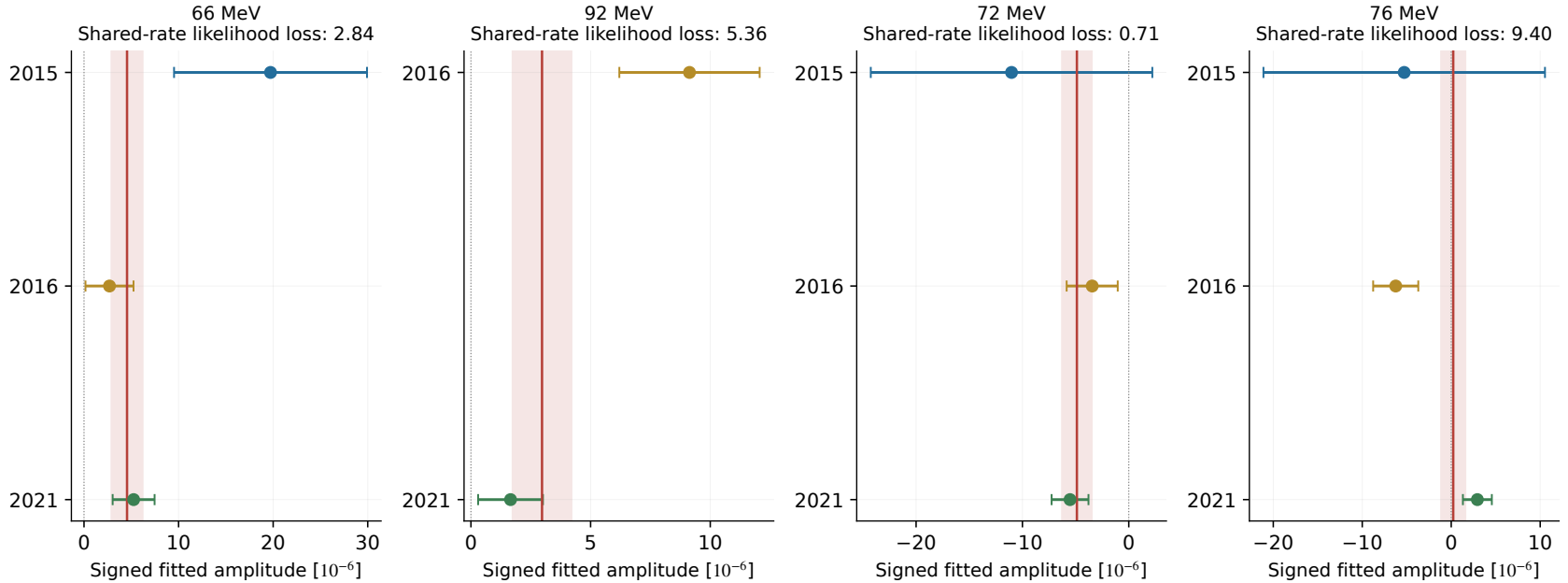
Figure 85: Separate campaign coupling estimates and local curvature errors compared with the common rate. The likelihood loss quantifies how much the local fit improves when each year can choose its own amplitude. The 66 MeV fit has positive contributions from all three years; the 92 MeV separate rates differ more visibly. These selected comparisons and local errors are not post-selection compatibility tests.
