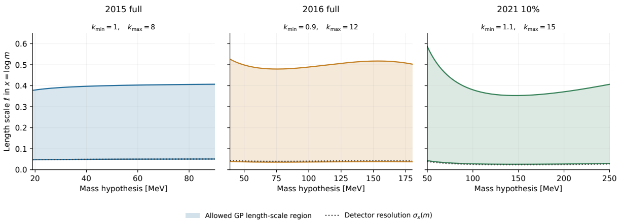
Figure 28: Allowed RBF length scales in x = \log m across the three search ranges. Shading lies between the lower and upper bounds evaluated from the frozen analysis card; the dotted curves show the local detector-resolution scale \sigma_x(m) . The lower/upper factors are 1.0/8, 0.9/12, and 1.1/15 for 2015, 2016, and 2021, respectively. These are numerical domains for the sideband fit, not fitted length scales or detector-resolution uncertainties.
