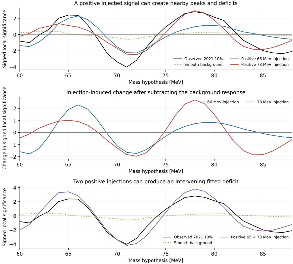
Figure 74: Positive injected signals can induce nearby fitted oscillations through the moving-mask background regression. The injection-induced change is \Delta r(m) = r_m(B + S) - r_m(B) for the same smooth reference spectrum. The 65+78 MeV pair can induce a deep fitted deficit even though both generating signal components are nonnegative. These are conditional response illustrations; their agreement with one selected dip does not establish the identity of the observed parent peak.
