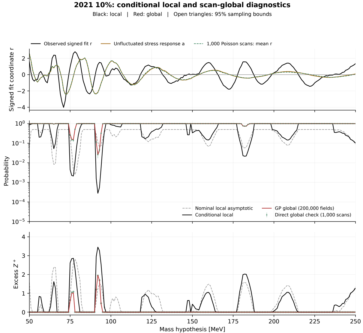
Figure 80: Profiled study for the released 2021 10% sample. The principal ordering selects 92 MeV and gives GP global probability 0.02519 ( Z = 1.957 ), with 26/1,000 direct exceedances. The GP ensemble retains 200,000 fields. Black is the conditional local probability and red the global probability, with the corresponding Z^+ below. This global calculation uses the correlated field rather than the Sidak correction used for the asymptotic references. Qualification of the generating background remains required for a particle-global interpretation.
