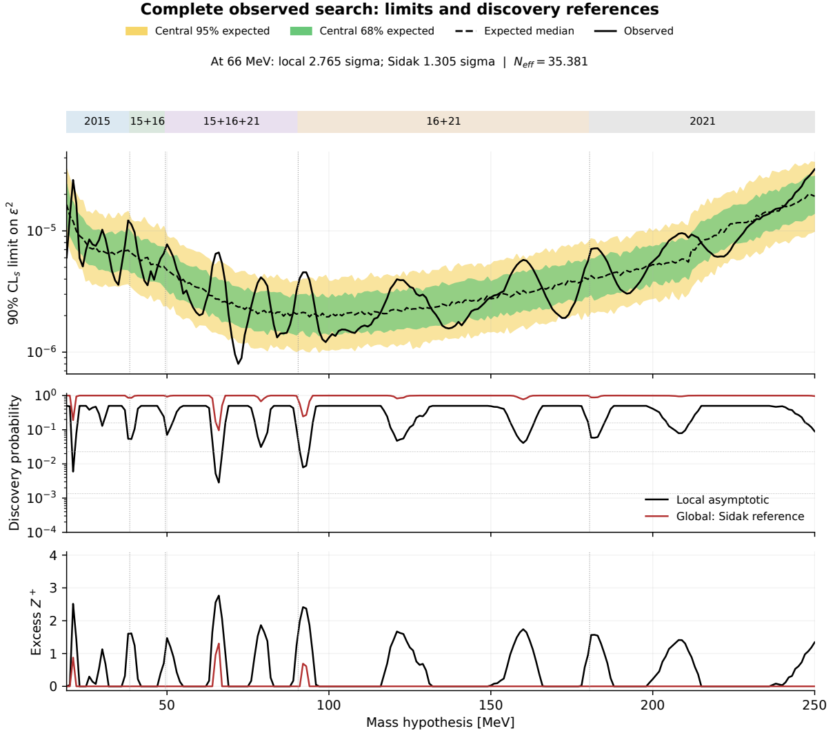
Figure 52: Complete 19–250 MeV observed search, with the preassigned active datasets shown above the curves. The upper panel shows 90% \text{CL}_s limits and the median, central 68% and central 95% ranges of the original 300 conditional background-only toys per mass. The next two panels show the unchanged fixed-mass asymptotic p_0 and its normal-quantile significance, with the local reference in black and the Sidak reference in red. The latter uses N_{\text{eff}} = 35.381 for the complete search; its value at 66 MeV is Z_{\text{Sidak}} = 1.305 , compared with local Z = 2.765 . The observed polyline connects every adjacent tested mass, including membership transitions; no numerical endpoint is changed by those connections. The physical visible-branching correction is applied once above the dimuon threshold. These are pointwise bands; 2016-inclusive values retain the numerical exception.
