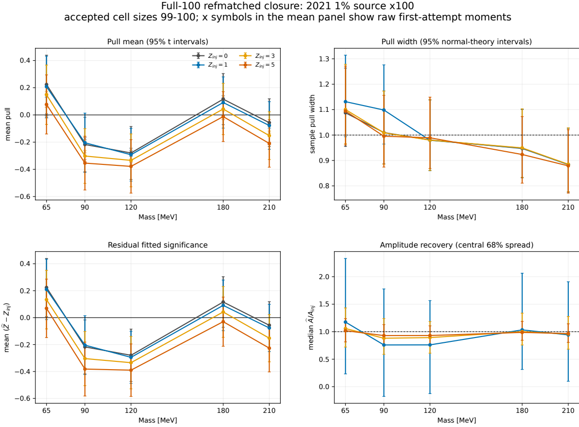
Figure 107: As in Fig. 105, for 1\% \times 100 . The 90 MeV, z = 3 cell retains 99 toys after one irreproducible injected refit is excluded; all other cells retain 100. Eighty-five of 1999 accepted fits contact the factor-15 upper length-scale bound. Stable contacts are reported rather than removed or used to change the frozen card.
