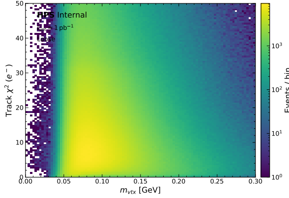
(a) Mass vs. electron \chi^2 (data).
