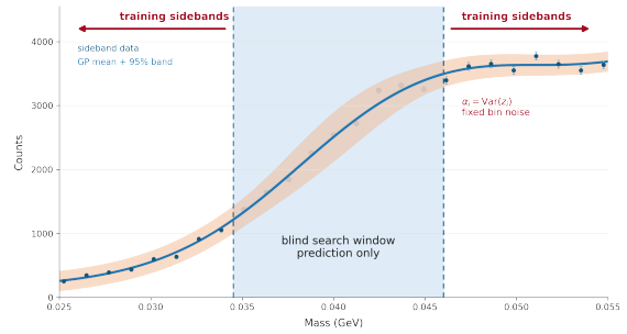
(b) Sideband-only training and blinded-window prediction. Filled markers show binned count data, vertical error bars show the fixed per-bin statistical noise, and the horizontal reference lines are count-axis guides used to compare sideband and blinded-window scales.
