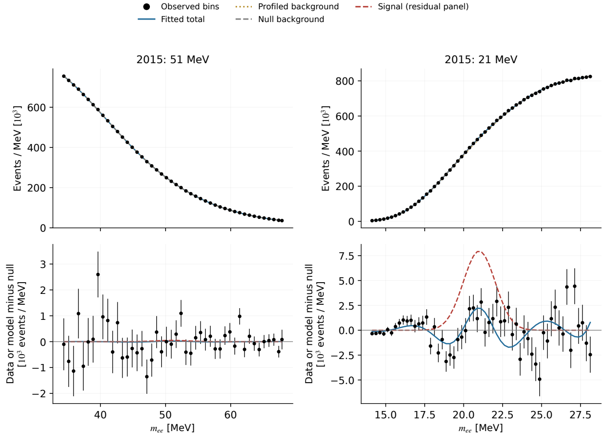
Figure 97: Traditional baseline fits to full 2015 data. At 51 and 21 MeV the nominal local coordinates are 0.131 and 5.580, with D/\text{dof} = 141.69/131 and 92.50/50 . Adjacent bins are summed for display: 0.75 MeV at the 51 MeV hypothesis, and 0.25 MeV at 21 MeV. Every fit still uses the original 0.25 MeV bins. Counts and residuals are divided by the actual displayed width, including a partial endpoint group. Bottom: data minus the refitted null background, with counting errors only. The red Gaussian is not the blue total change: the polynomial background also moves. Subtraction induces correlated residuals. The large 21 MeV root accompanies an inadequate overall fit. Table 21 retains all variants, including the badly fitting degree-two model at 51 MeV; neither extreme is a defensible physical significance.
