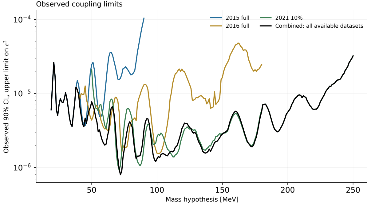
Figure 53: Observed coupling limits from the three individual released samples and the full maximal-available-dataset combination of Fig. 52. Only observed limits are shown. The combination is obtained from a shared-coupling likelihood with the fixed membership rule; it is not the envelope of the individual curves.
