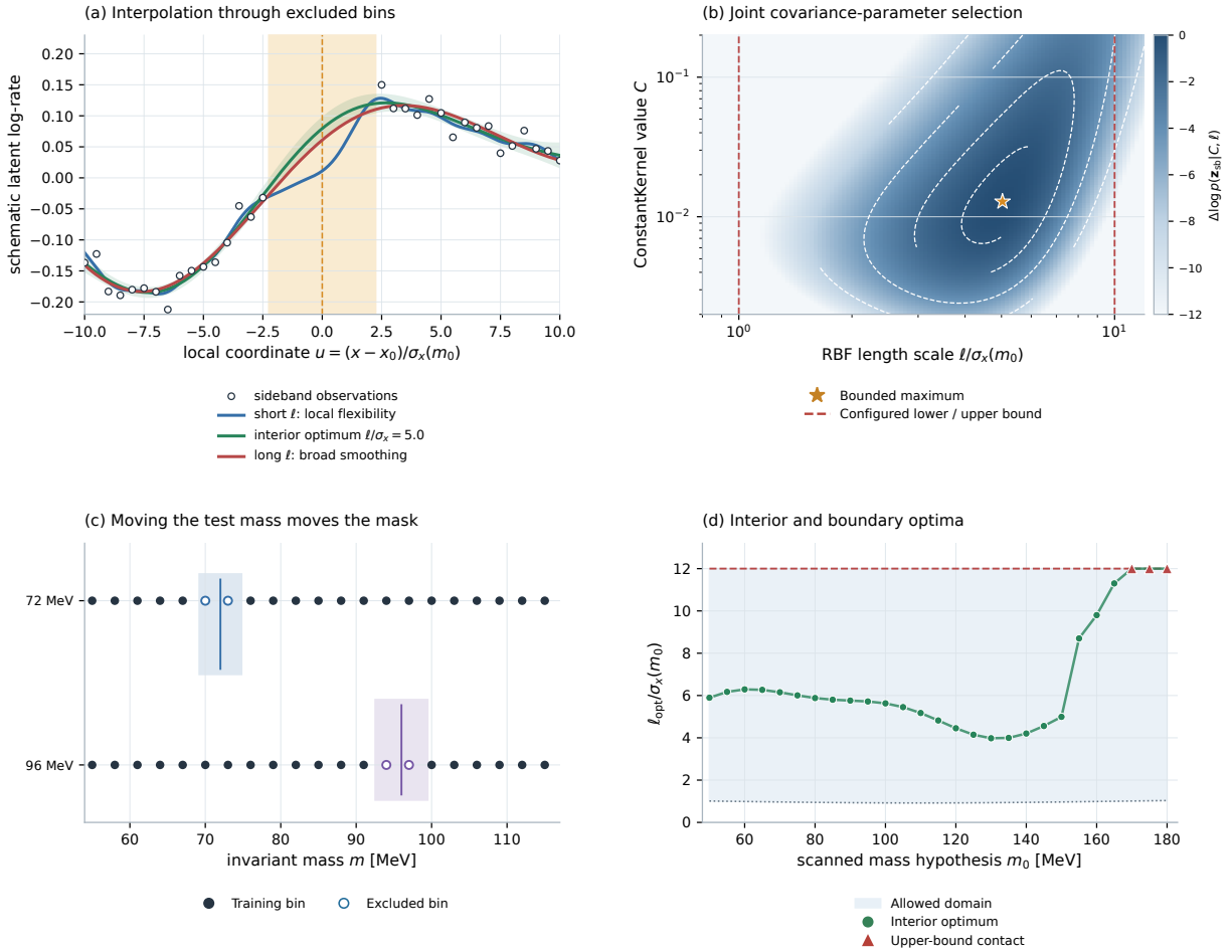
Figure 27: Meaning of per-mass-hypothesis hyperparameter optimization. Panel (a) shows one schematic sideband problem in u = (x - x_0)/\sigma_x(m_0) . The shaded 2.25\sigma_x interval is excluded from training; the three curves illustrate the different interpolation behavior allowed by short, interior, and long candidate length scales. Panel (b) shows the joint log-marginal-likelihood surface for the same synthetic sidebands. The star is the bounded maximum in (C, \ell) , and the elongated contours expose their possible tradeoff. Panel (c) shows that moving m_0 changes both the sideband mask and the local resolution scale that defines the allowed \ell interval. Panel (d) illustrates how a scan records an interior optimum differently from repeated upper-bound contact: the former is a conditional best fit within a nonbinding range, whereas the latter diagnoses an active numerical domain and motivates a predeclared range and closure study. The figure is explanatory only; it contains no HPS observations or fit results.
