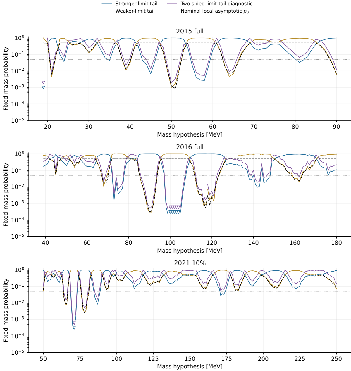
Figure 63: Empirical limit-tail diagnostics for each dataset. Unrefined points use 300 toys; selected coordinates use the saved independent 3,000- or 10,000-toy batches. Open downward triangles show one-sided 95% Monte Carlo upper bounds when no tail event is observed; for the two-sided diagnostic the bound is doubled and capped at one. These probabilities refer to the upper-limit statistic and are distinct from local asymptotic p_0 .
