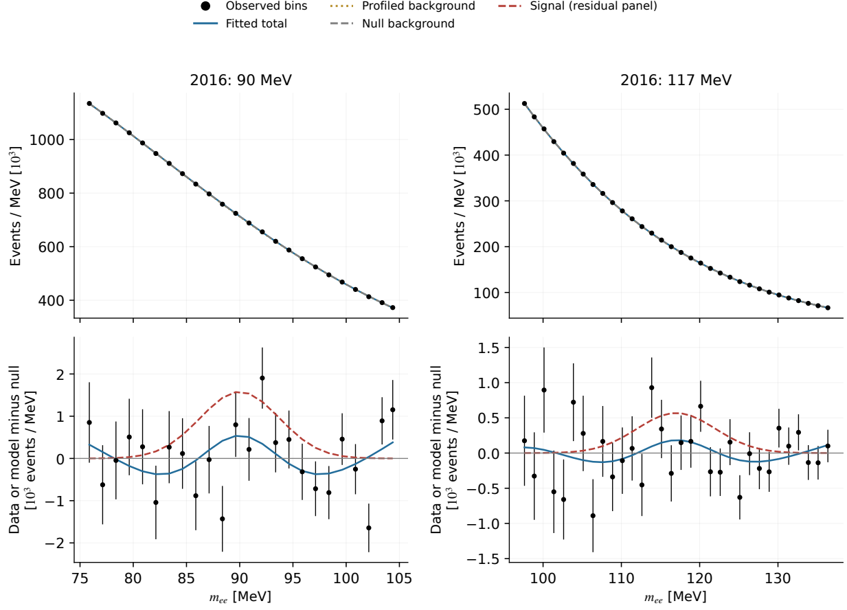
Figure 98: Traditional baseline fits to full 2016 data. At 90 and 117 MeV the nominal local coordinates are 1.998 and 1.525, with D/\text{dof} = 125.35/113 and 165.59/155 . The display sums five adjacent native bins to 1.25 MeV; any partial endpoint is retained. Counts, residuals and predictions are divided by each displayed width. Fits and probabilities still use the original 0.25 MeV bins. Both baseline positive roots are weaker than their GP values. Reducing the polynomial degree gives negative yields and larger deviances (Table 21). All alternatives are retained. Numerical convergence does not establish that a background describes the data; nominal local probabilities refer only to that model at the already selected mass.
