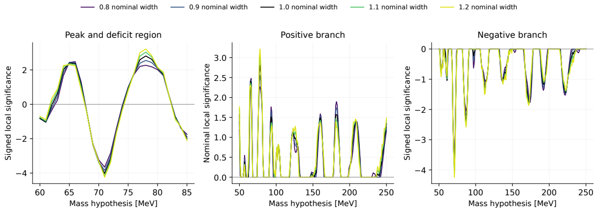
Figure 66: Local significance under the same template-width variations. The plotted signed local coordinate is r = \text{sign}(\hat{A})\sqrt{2[\text{NLL}(0) - \text{NLL}(\hat{A})]} ; its negative branch describes deficits. The 1.2-width template changes the 78 MeV value from 2.810 to 3.216 and the 71 MeV value from -4.019 to -4.239 . The 66 MeV reference changes from 2.366 to 2.478 for the 0.8-width template.
