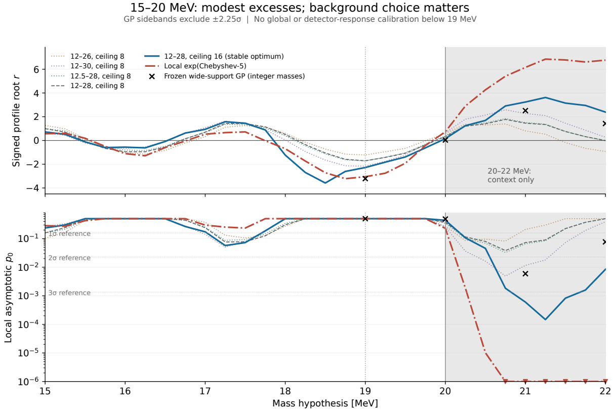
Figure 117: Signed local significance and local asymptotic excess probabilities. All four initial GP supports reach the inherited ceiling of eight resolution units. Raising the nominal-support ceiling to 16 removes every active boundary; ceilings 32 and 64 recover the same optima, with maximum root changes below 0.00054. The local polynomial is a separate background-family check. Gray shading identifies the 20–22 MeV bridge. Triangles mark the 10^{-6} display floor, not resolved global tails.
