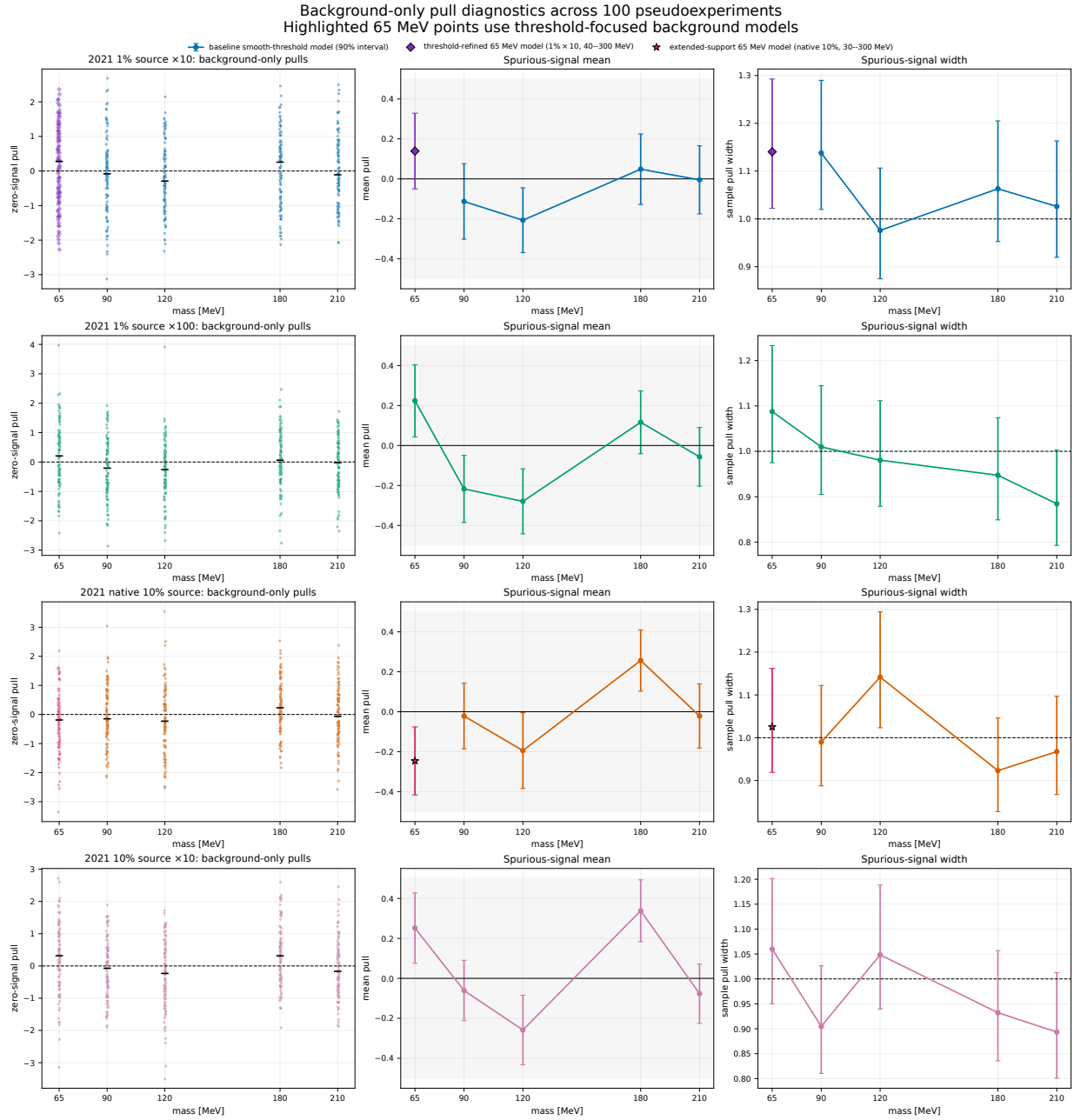
Figure 47: Zero-signal diagnostics for four 2021 exposure ensembles, with 100 pseudoexperiments per point. Circular markers show the baseline smooth-threshold model. At 65 MeV, diamonds and stars show the two threshold-focused tests defined in Table 7; they replace, rather than pool with, the baseline points. Bars are two-sided 90% intervals.
