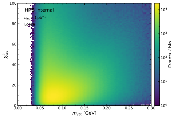
(e) Mass vs. vertex \chi^2 (data).
