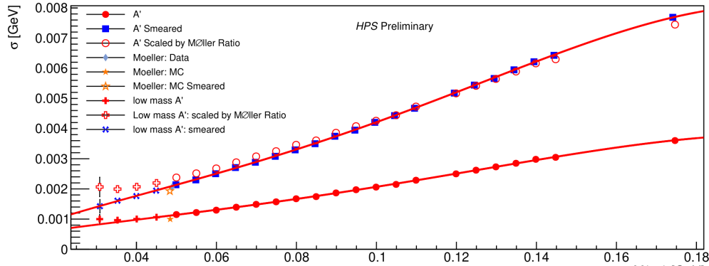
Figure 15: 2016 smeared- A' and Møller-based mass-resolution summary [28]. The smeared A' points show how the data-driven momentum-smearing correction is propagated away from the single Møller calibration point. The worsening resolution with mass broadens the signal window and is one of the main detector effects limiting prompt sensitivity at higher mass.
