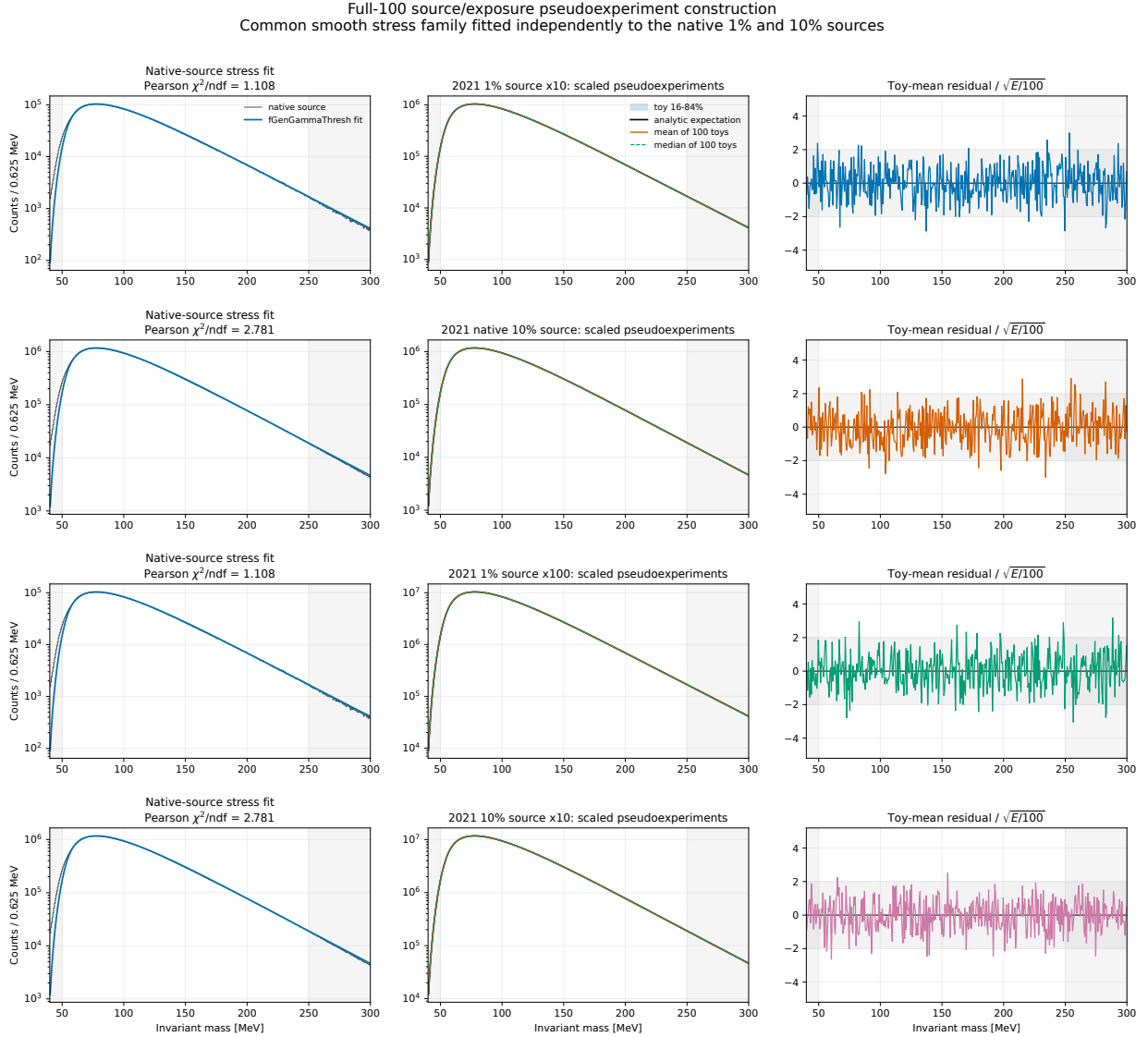
Figure 101: Invariant-mass construction of the full-100 ensembles, following the functional-form display of Fig. 46. Each row shows the native source and independently fitted stress truth (left), the scaled analytic expectation with the mean, median, and central 68% range of 100 background pseudoexperiments (middle), and the toy-mean residual divided by its expected standard error (right). Grey bands are support-only regions outside the 50–250 MeV search. The common analytic family isolates source/selection and normalization differences without claiming that either smooth function is a physical background generator.
