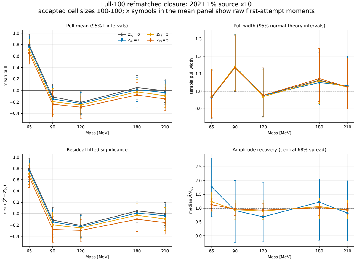
Figure 105: Full-100 refmatched closure for 1\% \times 10 . Every cell retains 100 accepted toys. The persistent positive 65 MeV pull means and the corresponding analytic-mean result are local stress-truth/model offsets; the other masses have near-unit widths and substantially smaller means. Crosses in the mean panel show raw first-attempt moments before the predeclared LML/reproducibility selection.
