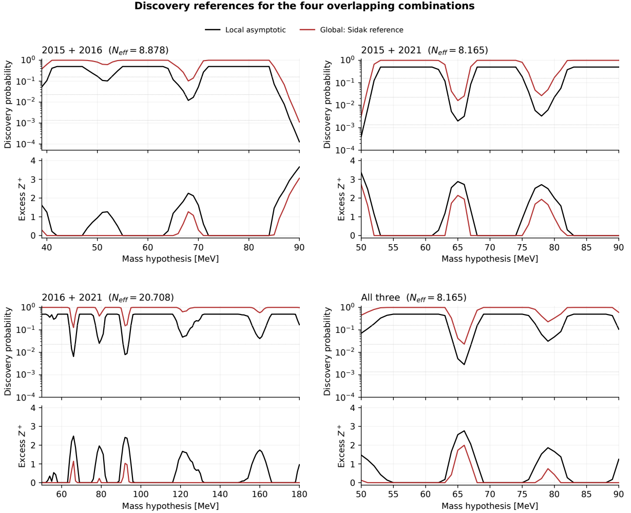
Figure 84: Discovery probabilities and aligned Z^+ values for all four overlapping combinations. Local asymptotic curves are black and Sidak global references are red. Each pair of panels shares its mass axis and uses one fixed N_{\text{eff}} over that scope's full overlap. The local curves are the unchanged shared-coupling fits. These are analytic Sidak references, distinct from the stress-centered correlated-field global probabilities above; no additional correction for selecting among overlapping scopes is included.
