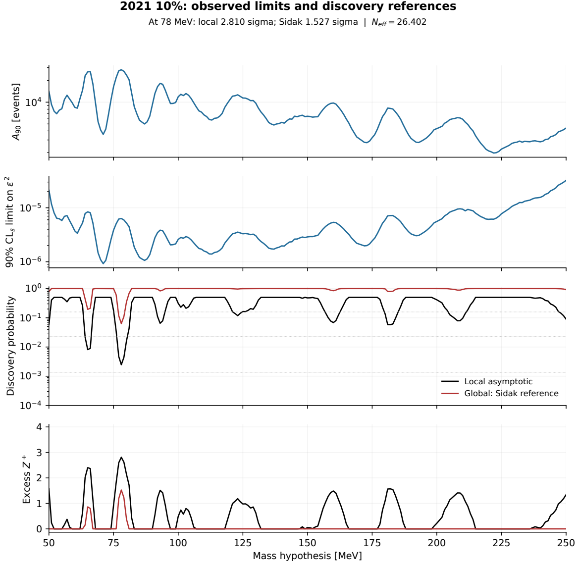
Figure 57: Corresponding observed 2021 10% scan on 50–250 MeV with 36–300 MeV GP support. The panels show the full-template A_{90} , minimal-visible \epsilon^2 limit, discovery probabilities, and aligned Z^+ values. Black is local and red is the Sidak reference with N_{\text{eff}} = 26.402 ; their values at 78 MeV are 2.810 and 1.527. Above the dimuon threshold the inherited branching correction enters the coupling conversion once; it does not change the visible electron-pair yield or local probability.
