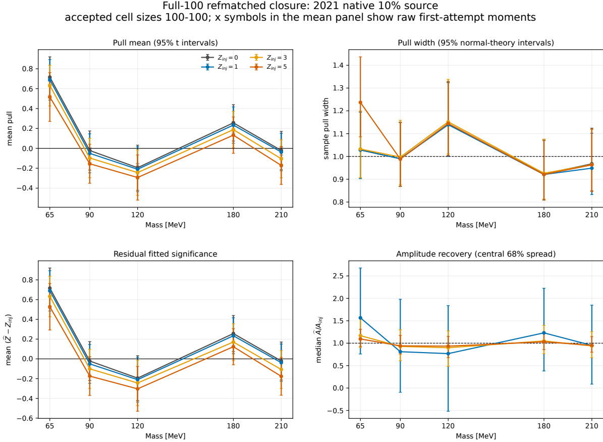
Figure 106: As in Fig. 105, for the native-10% ensemble. All cells retain 100 toys. The largest mean offset is at 65 MeV. The only accepted width outside 0.8–1.2 in the complete study is 1.237 for the 65 MeV, z = 5 cell; its normal-theory 95% interval is [1.086, 1.437].
