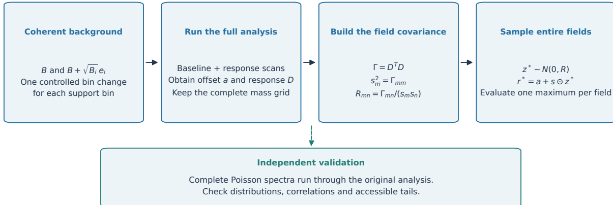
Figure 38: The computational gain in the significance-GP method. Full analysis scans of controlled perturbations estimate the field covariance once. Gaussian vector draws then produce many correlated scans without repeating those fits. A separate ensemble of complete Poisson experiments tests the approximation. This is an explanatory diagram of the archived HPS implementation, following Ref. [42]; the offset and width are retained explicitly.
