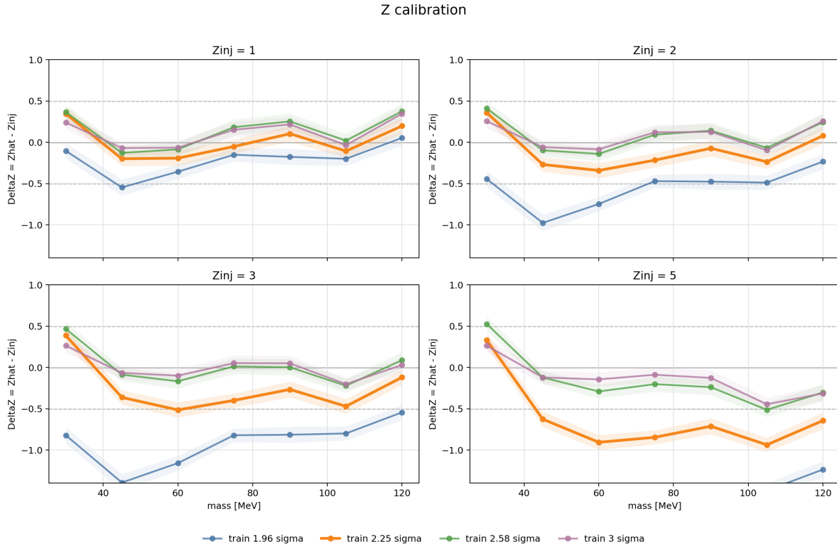
Figure 42: Residual fitted significance in the same historical 2015 training-exclusion study as Fig. 41. The common mass and injection grid compares the response after the signal strength has been set by its matched reference. Together with amplitude recovery, this diagnoses the signal-absorption cost of letting the GP train too close to the extraction window.
