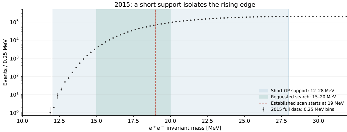
Figure 116: The same released full-2015 histogram, summed from 0.05 to 0.25 MeV bins. The chosen GP support is 12–28 MeV; the requested search is 15–20 MeV. The dashed line marks the lower boundary of the established scan, not the lower boundary of the available counts.
