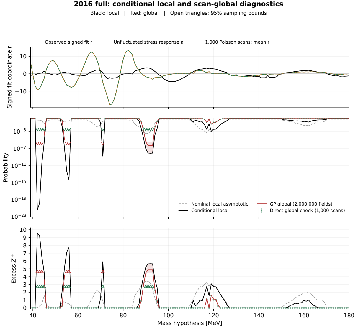
Figure 79: Profiled 2016 conditional global study with the same black-local/red-global convention and integer Z^+ guides. The GP ensemble now has 2,000,000 fields. At the leading 42 MeV threshold there are still zero exceedances: p < 1.498 \times 10^{-6} , or Z > 4.671 , as a one-sided 95% sampling bound within this Gaussian model. The independent direct check remains 0/1,000, giving only p < 0.002991 ( Z > 2.749 ). Open downward triangles in probability become upward triangles in Z ; they are bounds, not measured significances. This correlated-field global probability is different from the Sidak global reference.
