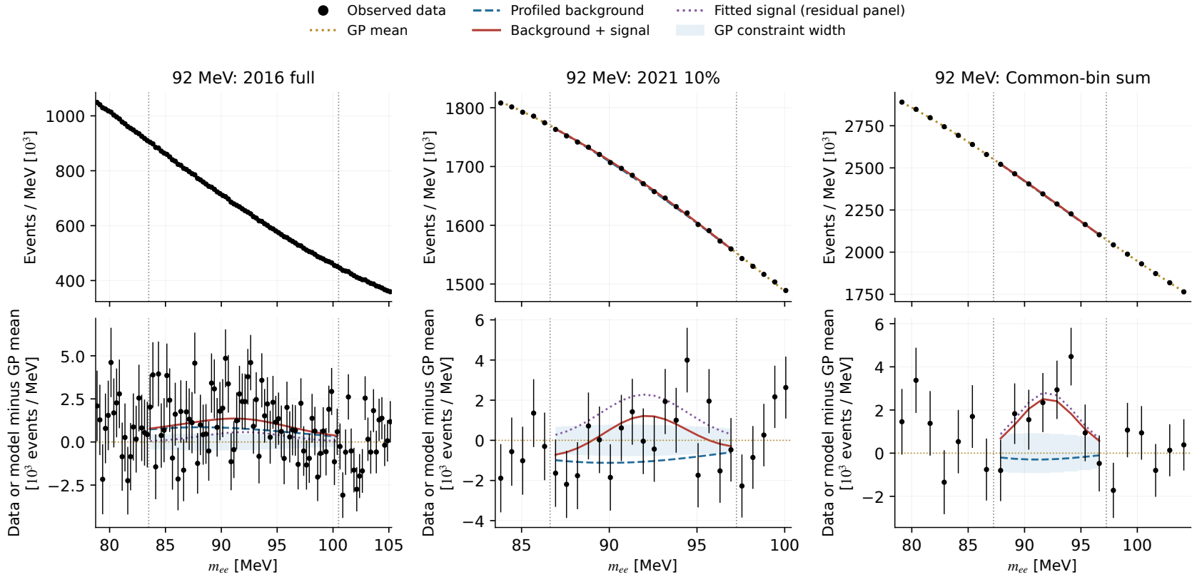
Figure 68: The 92 MeV common-coupling fit uses 2016 and 2021 and gives \hat{\epsilon}^2 = 2.97 \times 10^{-6} with nominal local significance 2.42. The separate preferred rates differ, as shown at the end of this results section. Bars show counting error only; residual shading shows the zero-centered GP constraint width, not fitted-background or total residual uncertainty.
