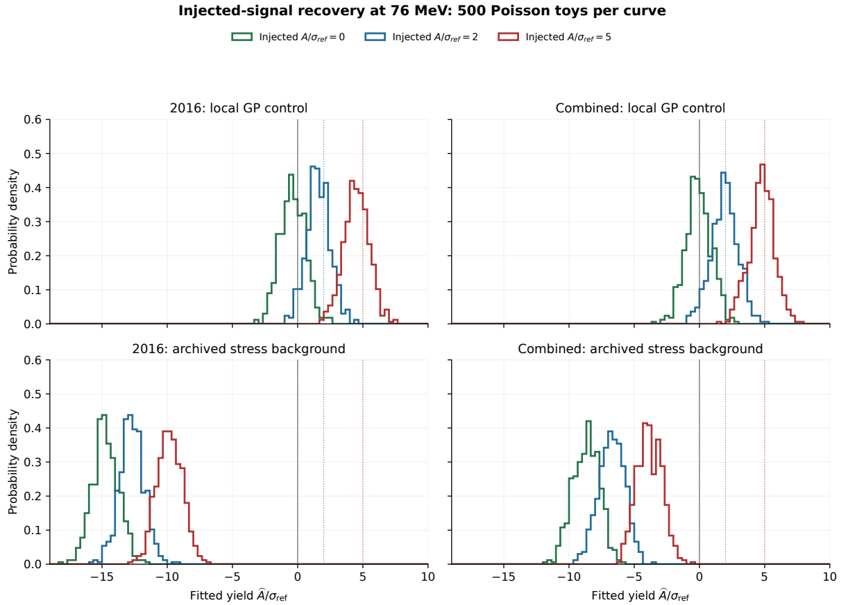
Figure 83: Saved 76 MeV signal-injection experiments, with identical axes for the local-GP controls (top) and archived stress backgrounds (bottom). Each curve has 500 independent Poisson spectra; dotted vertical guides mark the true injected yields 0, 2, 5 in units of that scope’s fixed \sigma_{\text{ref}} . The distributions move with injection, but the stress-background bias persists. These fitted-yield distributions show recovery and its failure mode explicitly; injection size five does not mean a measured 5\sigma signal. No new injection toys were generated for this display.
