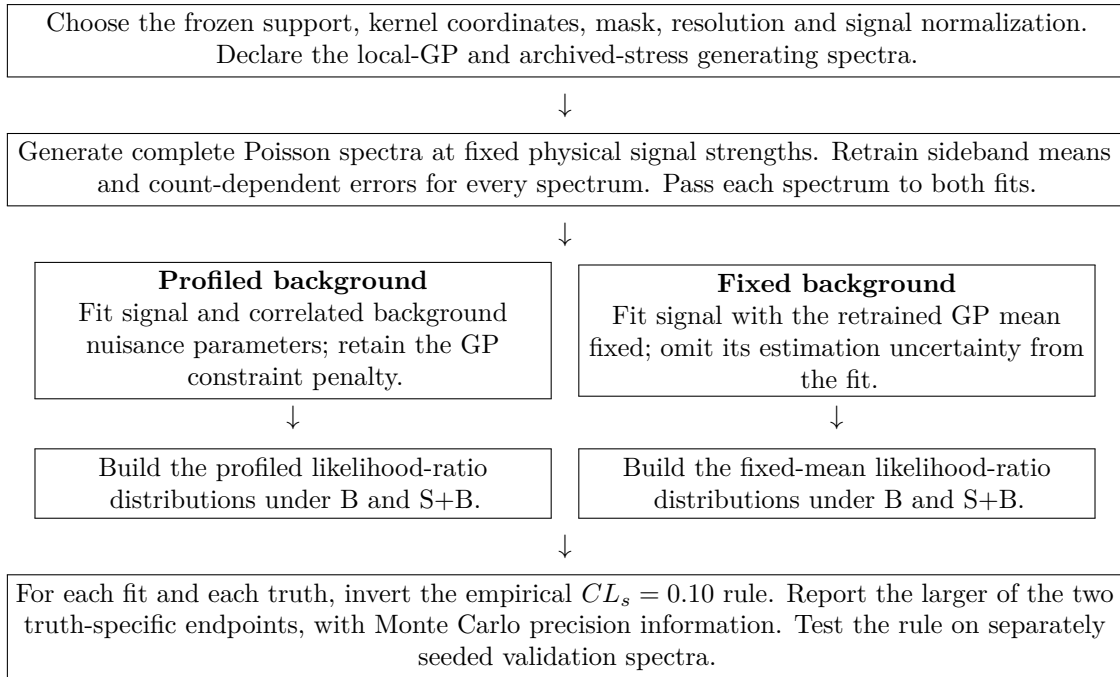
Figure 86: How the two background treatments are calibrated. Both branches receive identical spectra. The primary comparison uses two declared background truths for each method; it does not average the two methods or select whichever gives the tighter observed limit. B denotes background only and S+B denotes signal plus background.
