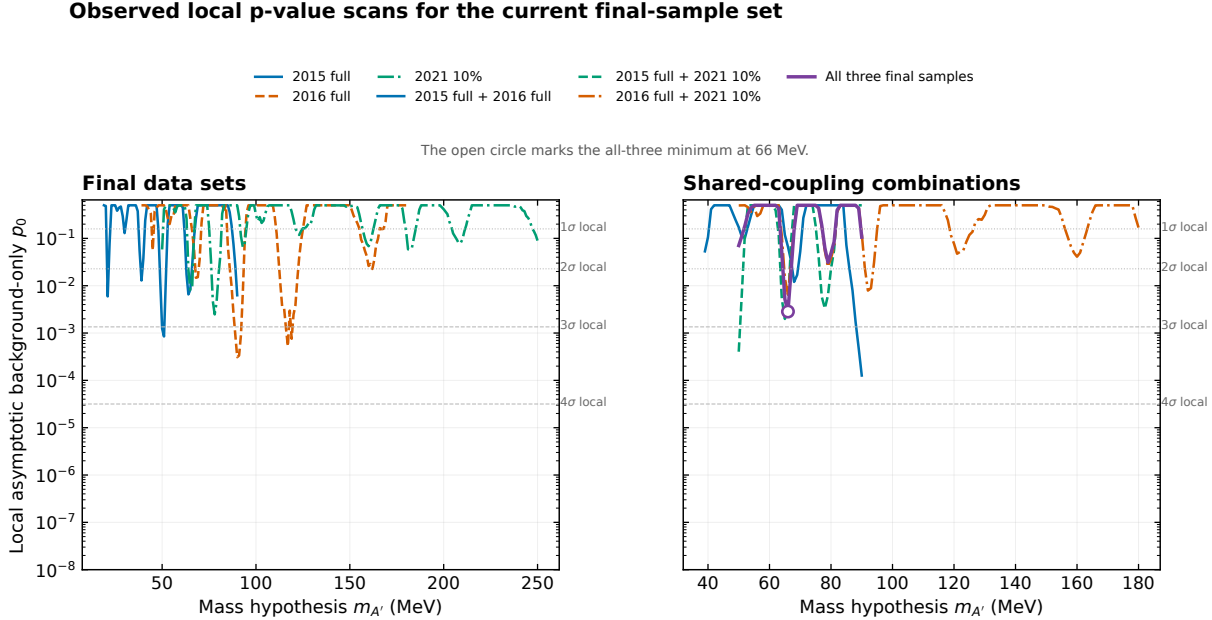
Figure 59: Local one-sided asymptotic background-only p_0 for the three standalone inputs, the three pairs, and the all-three combination. The values are conditional on the frozen GP supports and states. No look-elsewhere correction, global significance, or toy calibration is reported.
