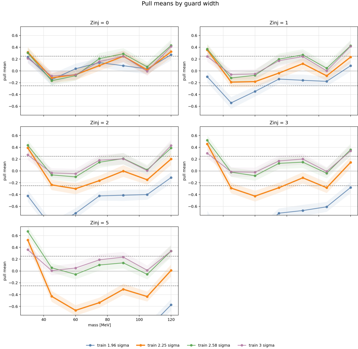
Figure 43: Signal-extraction pull means from the same historical training-exclusion comparison. The mass-dependent offsets supplement the recovery diagnostics in Figs. 41 and 42. These are historical conditional response tests for the stated generating truth and masks.
