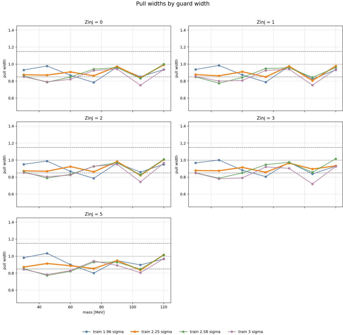
Figure 44: Signal-extraction pull widths from the same historical training-exclusion comparison. They test the reported uncertainty scale alongside the pull means in Fig. 43. The recovery, mean and width diagnostics informed the 2.25\sigma_m training choice; the subsequent extraction-geometry comparison is shown separately below.
