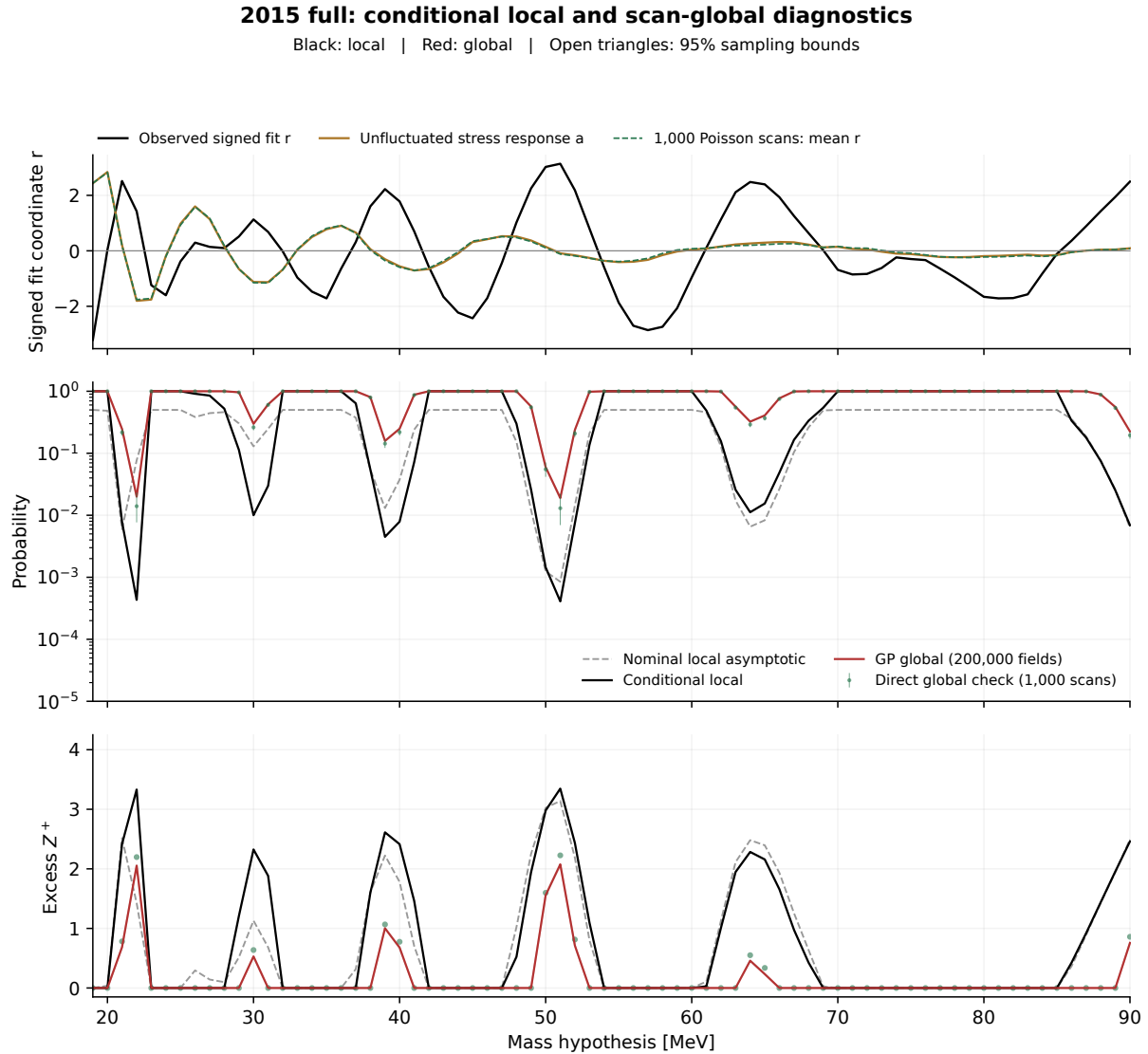
Figure 78: Profiled 2015 local and conditional GP global probabilities, with aligned Z^+ below. At the selected 51 MeV threshold the GP global probability is 0.018985 ( Z = 2.075 ); 13 of 1,000 direct scans exceed it. The GP ensemble contains 200,000 fields. Black is the conditional local curve and red the global curve; this global calculation uses correlated complete fields and is different from the Sidak global reference in the asymptotic plots. Shading and direct-scan bars give central 95% Monte Carlo intervals. The generating-background qualifications remain applicable.
