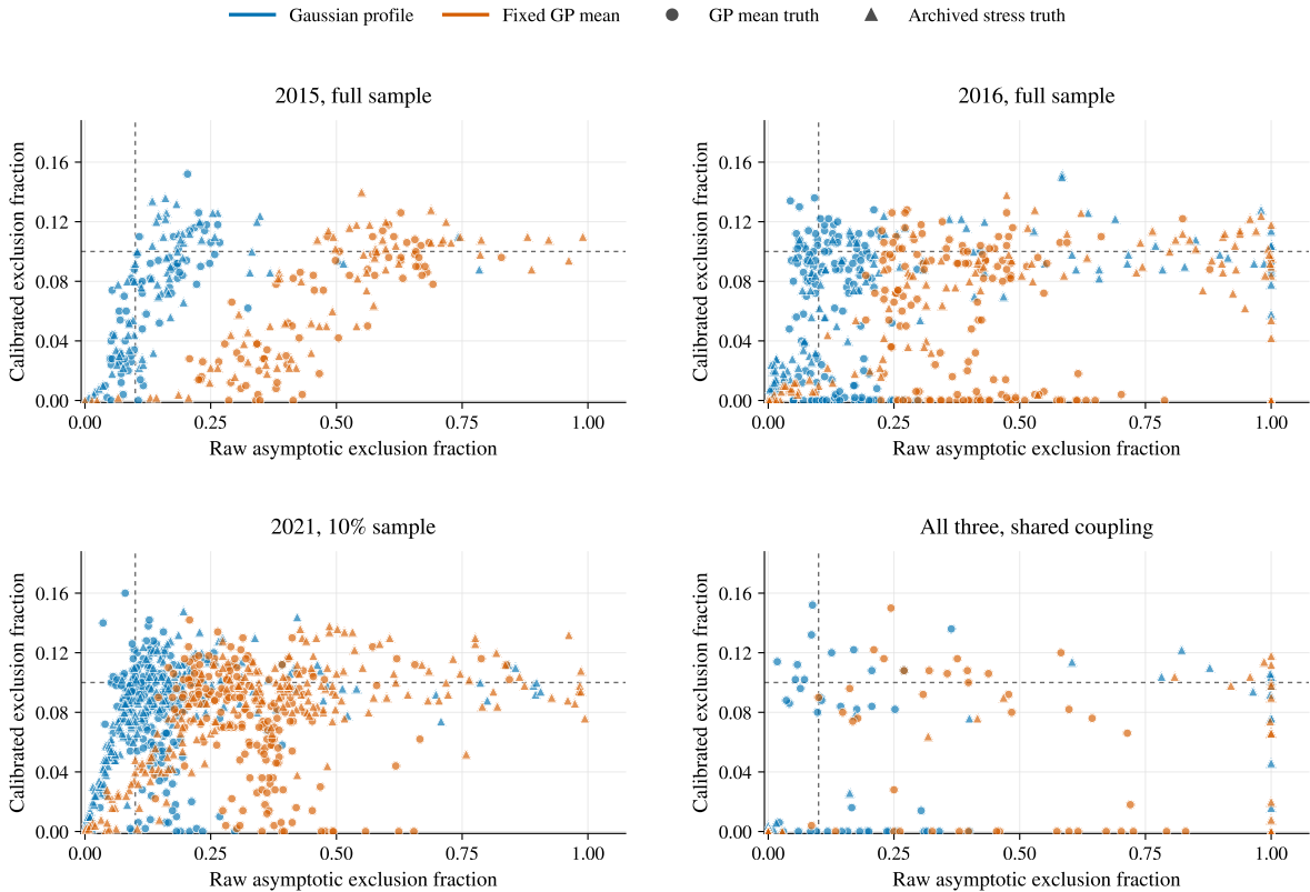
Figure 94: Independent validation with five-reference-error injections. The horizontal coordinate is the fraction of 500 spectra excluding the known injected yield with the raw asymptotic rule; the vertical coordinate uses the calibrated two-truth envelope. A point far to the right has an excessive raw exclusion rate. A point below the horizontal 0.10 guide indicates a conservative calibrated rate in that cell. The guides mark the nominal benchmark, not an expected discovery probability. Finite counts and Monte Carlo uncertainty limit the precision of each conclusion.
