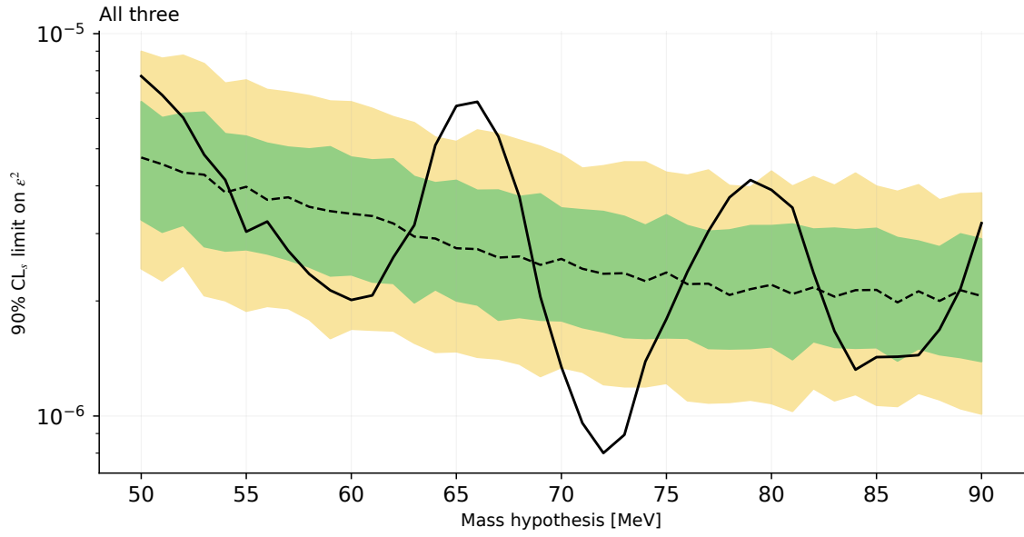
Figure 60: The all-three shared-coupling result on its common 50–90 MeV interval. Green and yellow show central 68% and 95% pointwise ranges, and the dashed curve is the median of 300 conditional background-only toys at each mass. The observed curve uses the same bounded asymptotic construction as the standalone fits.
