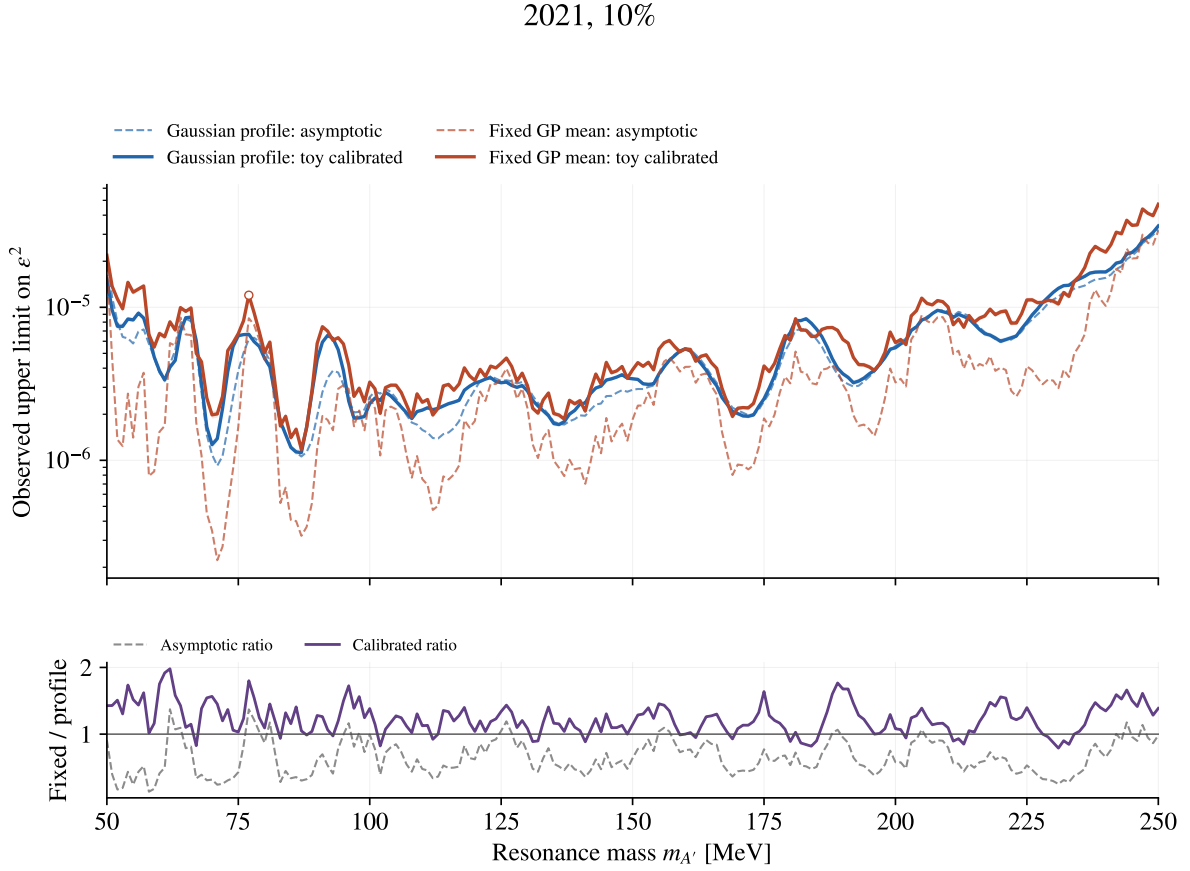
Figure 89: The same comparison for native 2021 10%. Both methods use the same physical sample and background-truth alternatives; the observed comparison does not measure an expected sensitivity gain.
