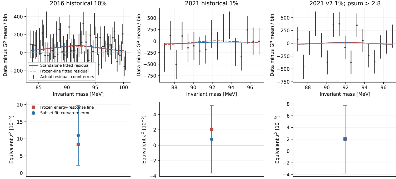
Figure 6: Actual smaller-sample histograms, with standalone and frozen-line fits. The line is the original v5.5.0 response at fixed 92 MeV, mapped through each histogram’s density using inherited resolution and radiative-fraction proxies. These are not calibrated efficiency predictions. The lower panels compare equivalent amplitudes and local curvature errors.
