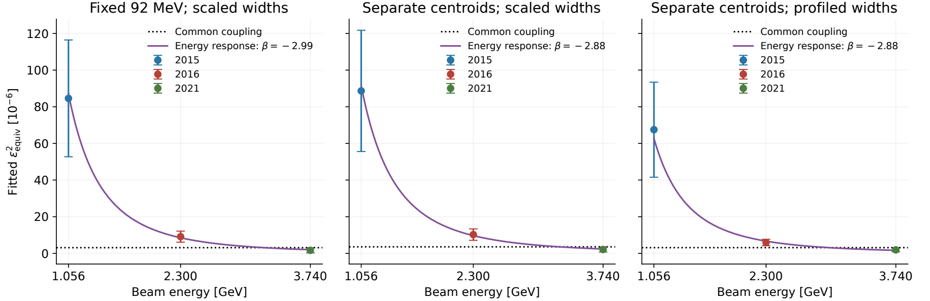
Figure 2: A counterpart of v5.5.0 Figure 2. Points are independently fitted nonnegative campaign amplitudes, with curvature errors conditional on their fitted shapes. Dotted lines show the common-coupling normalization; purple curves show the fitted energy response. Each model profiles its own allowed shapes on the same data and background constraint. Thus the floating-shape points and curve need not use identical centroids or widths. These are equivalent template normalizations, not measured particle couplings.
