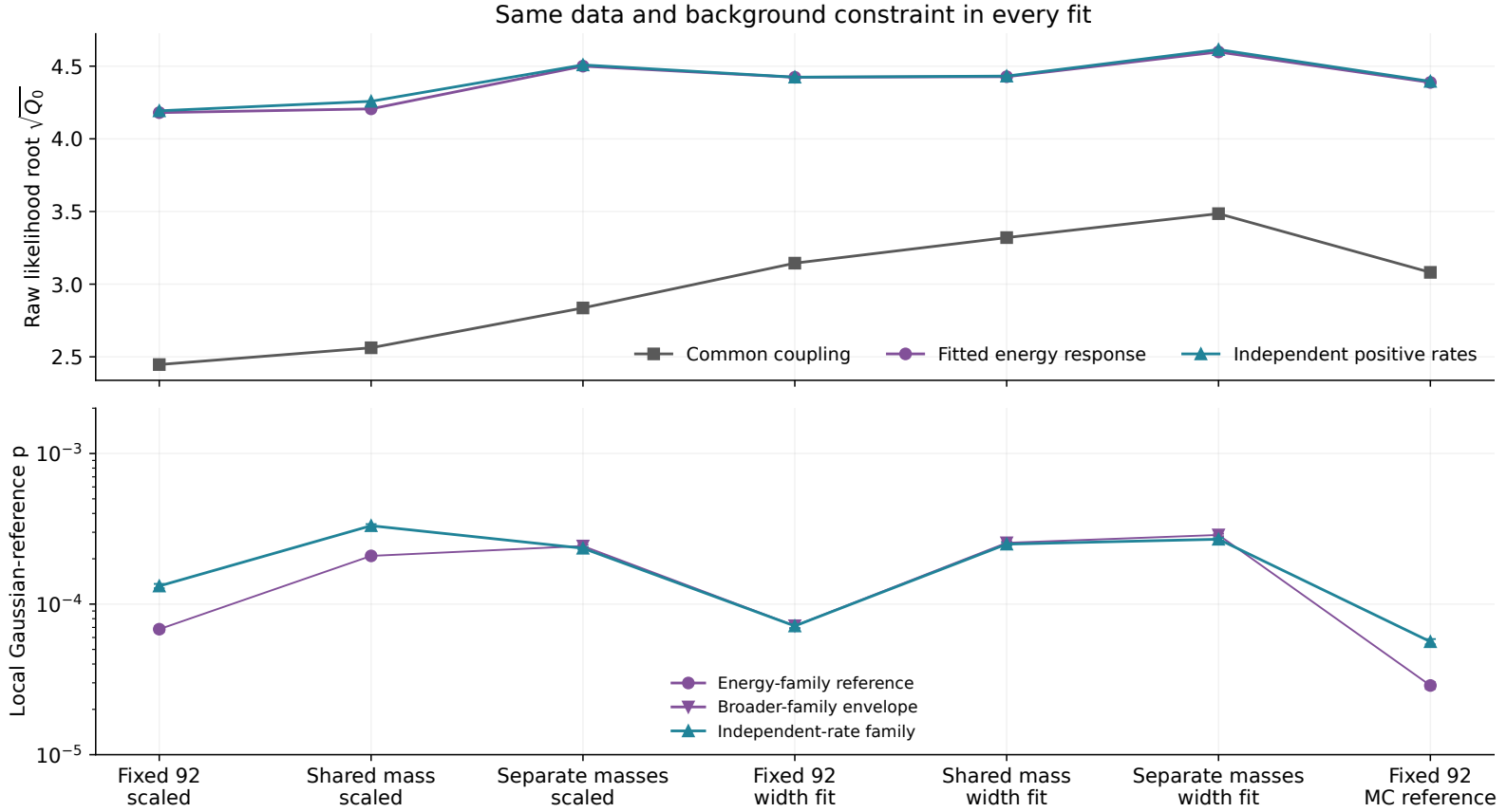
Figure 4: Top: exact conditional Poisson/Gaussian likelihood roots for three rate models. Bottom: predictive-Gaussian reference probabilities, with Monte Carlo error bars. Purple circles use the energy family itself; purple downward triangles use its broader independent-amplitude reference envelope. Blue triangles use independent rates. Lines guide the eye across distinct hypotheses, not nested steps in one scan. The final point is the fixed-MC control.
