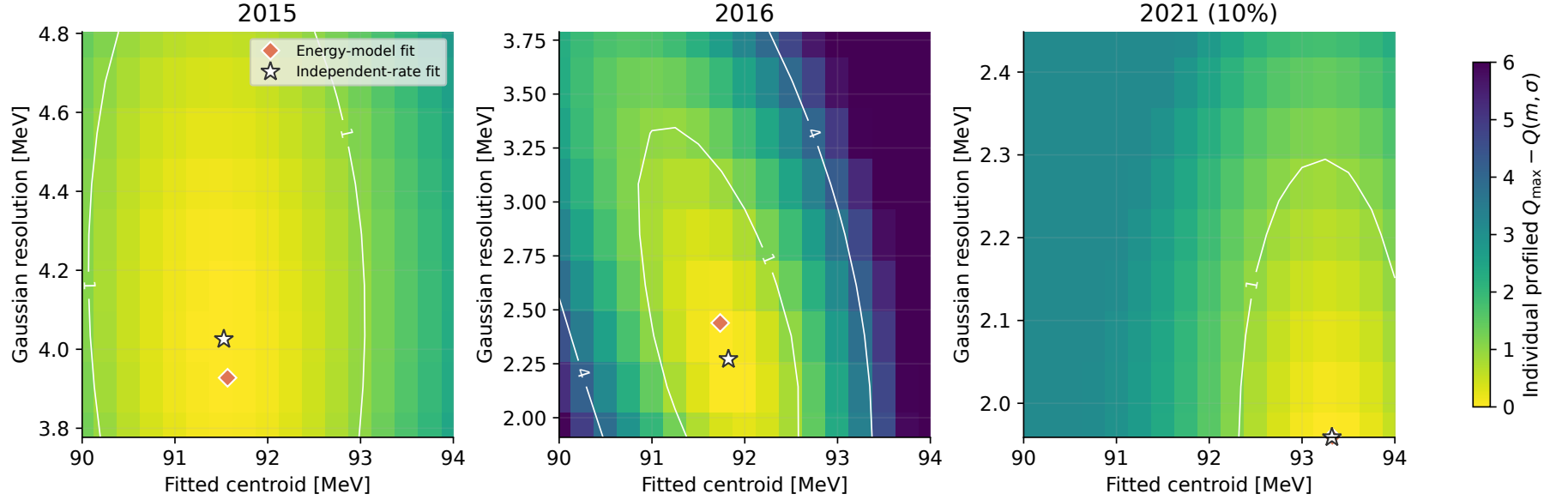
Figure 3: Individual amplitude-profiled shape surfaces with the MC-centered penalty. Colors and contours give differences in penalized Q_0 ; contours at 1 and 4 are descriptive. Diamonds mark the energy-model solution and stars independent rates. The lower and upper edges are MC-reference and scaled widths; 2021 reaches the lower edge.
