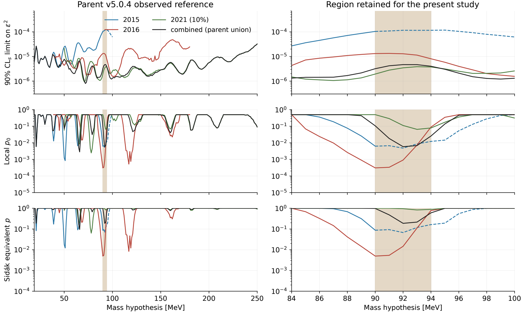
Figure 1: The unchanged v5.0.4 limits, local asymptotic p_0 , and Sidák-equivalent probabilities are the reference being combined. Shading marks 90–94 MeV; dashed 2015 segments denote its exploratory extension. Black is the parent union, whose active campaigns change with mass. The heuristic mapping is p_{\text{Sidak}} = 1 - (1 - p_0)^{N_{\text{eff}}} , using N_{\text{eff}} = 14.521, 16.062, 26.402 for the campaigns and 35.381 for the union. These are not trials factors calibrated for the new fits.
