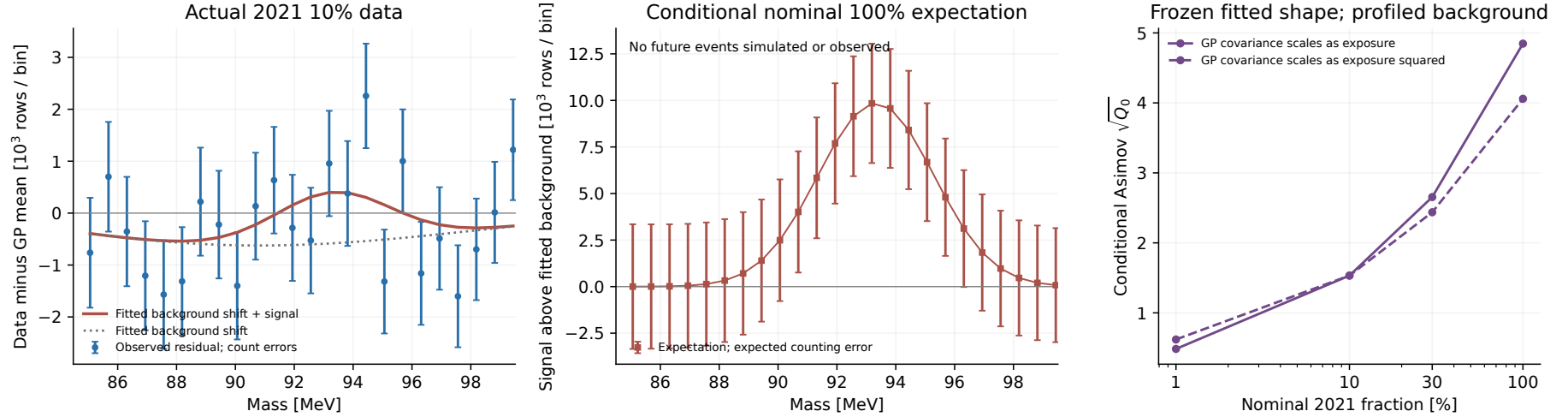
Figure 7: Left: actual 2021 10% residuals and the current combined-model fit. Middle: the expected signal at nominal full exposure if that fitted line and background persist. The subtraction changes from the GP mean on the left to the fitted background in the middle, as labeled. Future points are expectations, with expected counting-error bars; no future data or random pseudo-data are shown. Right: exact background-profiled Asimov likelihood roots for the frozen fitted shape under two assumed GP-covariance scalings.
