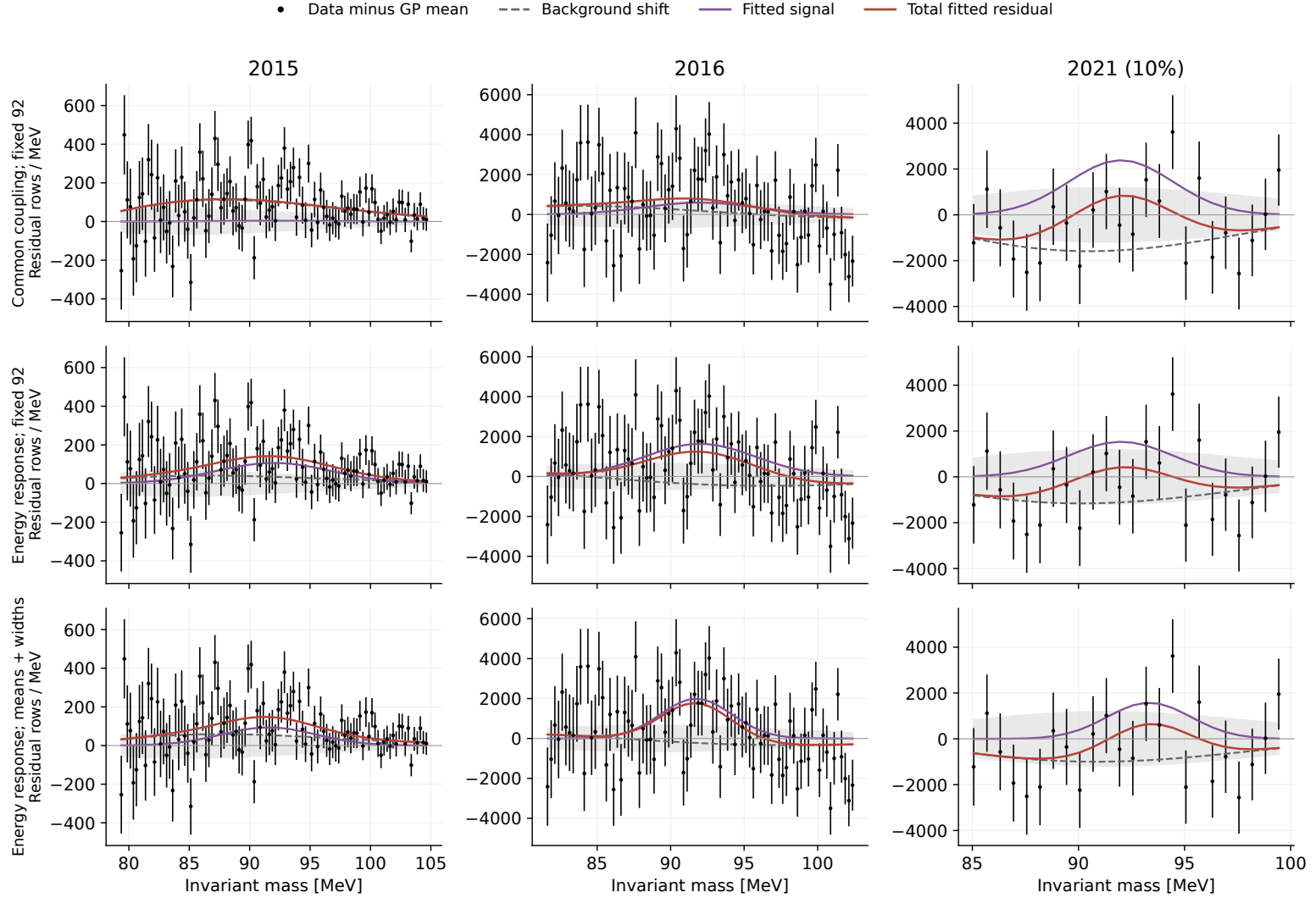
Figure 5: The same bins and GP mean appear in every row. Black points subtract that mean; error bars contain counting uncertainty only. Gray shading is the GP constraint standard deviation, the dashed line its fitted background adjustment, purple the signal, and red their sum. The top row imposes common coupling at 92 MeV; the middle fits the energy response at 92 MeV; the bottom also profiles separate centroids and bounded resolutions. Background adjustments remain visible rather than being attributed to the signal.
