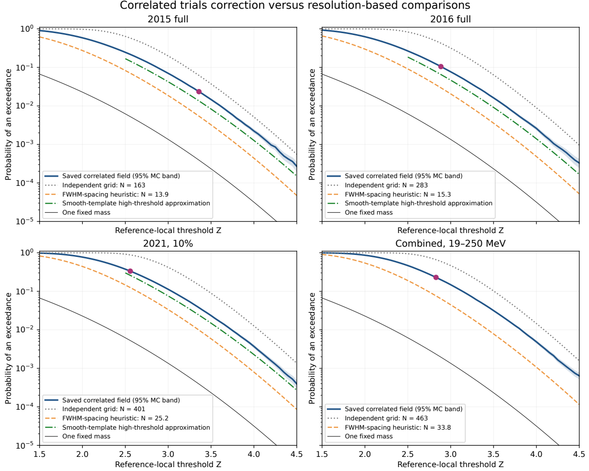
Figure 5: Reproduction of v5.8.3 Figure 5. Every curve in a panel is evaluated at the same reference-local threshold. The gray and orange curves are alternative counting approximations, while green describes an ideal smooth-template field. Blue uses the actual fitted-score covariance under the fixed nominal source. No new observed information enters this comparison.
