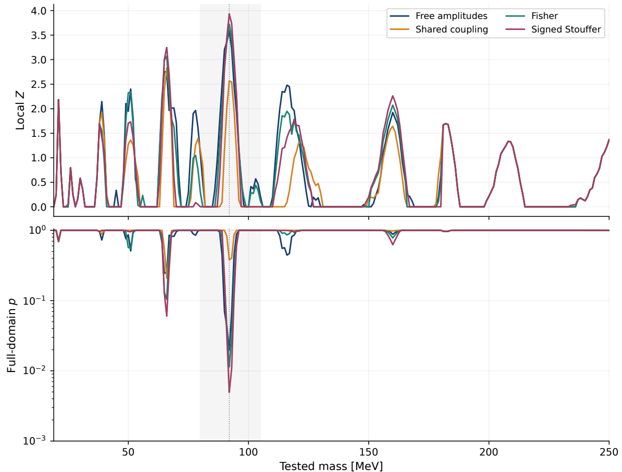
Figure 13: Baseline comparison from the earlier v5.8.5 report. All curves use the \pm 2.25\sigma_m mask and the 1 MeV mass grid; the global probabilities refer to the full 19–250 MeV domain. The shaded interval is a post-observation diagnostic zoom. The shared-coupling and independent-amplitude likelihoods impose different physical restrictions, while Fisher combines gated local probabilities and signed Stouffer combines continuous signed reference scores. These curves are strongly related uses of the same events.
