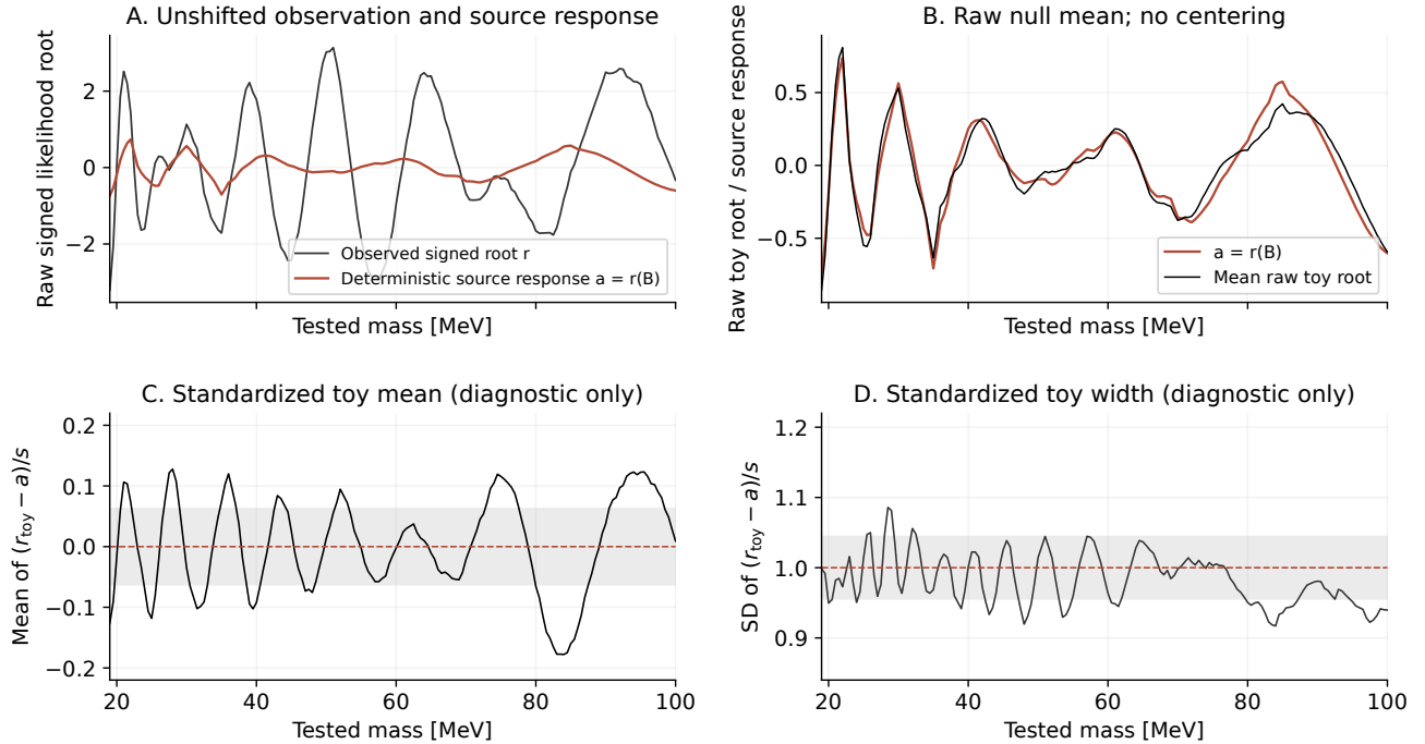
Figure 6: 2015 full: extension of Figure 4 in the consolidated v5.8.5 report. A: the unshifted observed root and deterministic source response. B: the mean raw toy root and the same deterministic response. C/D: standardized toy mean and width, used only to inspect the conditional response approximation; the observed local curves in Figure 2 are not standardized. Gray bands mark approximate pointwise one-standard-error scales for 256 Gaussian draws, not simultaneous acceptance bands.
