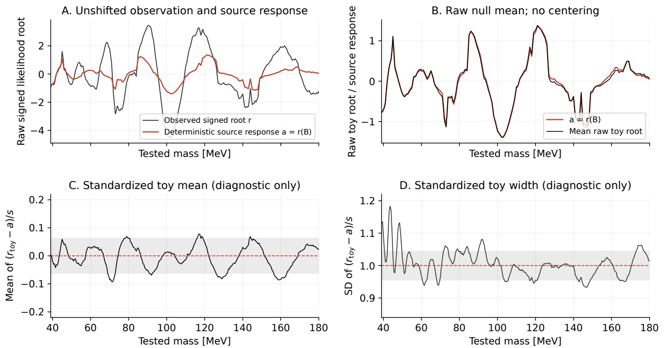
Figure 7: 2016 full: extension of Figure 4 in the consolidated v5.8.5 report. A: the unshifted observed root and deterministic source response. B: the mean raw toy root and the same deterministic response. C/D: standardized toy mean and width, used only to inspect the conditional response approximation; the observed local curves in Figure 2 are not standardized. Gray bands mark approximate pointwise one-standard-error scales for 256 Gaussian draws, not simultaneous acceptance bands.
