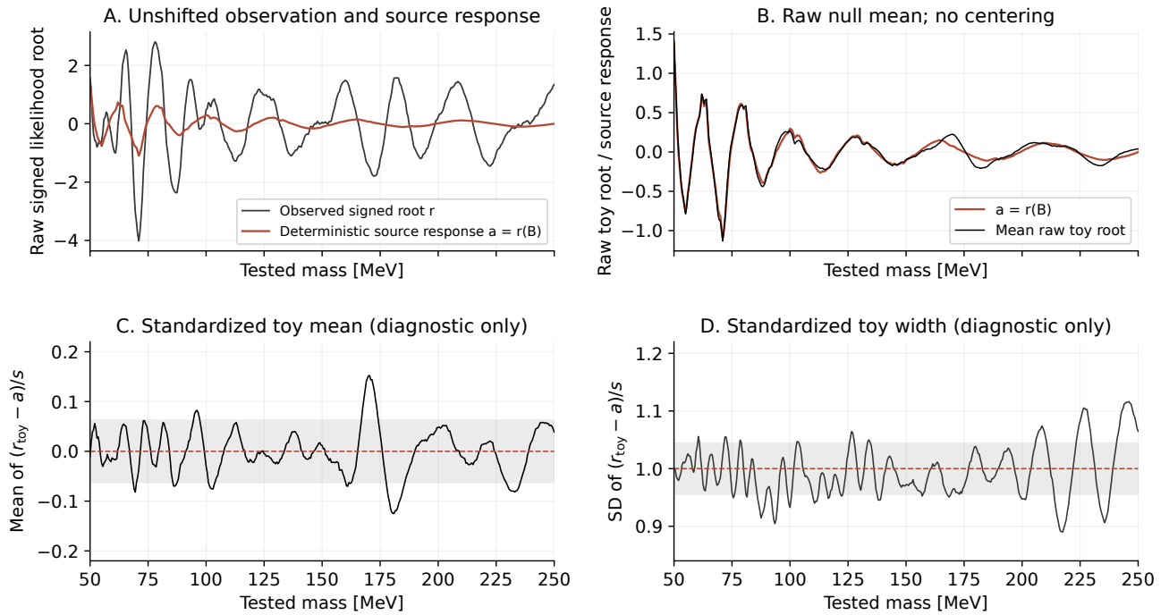
Figure 8: 2021 native 10%: extension of Figure 4 in the consolidated v5.8.5 report. A: the unshifted observed root and deterministic source response. B: the mean raw toy root and the same deterministic response. C/D: standardized toy mean and width, used only to inspect the conditional response approximation; the observed local curves in Figure 2 are not standardized. Gray bands mark approximate pointwise one-standard-error scales for 256 Gaussian draws, not simultaneous acceptance bands.
