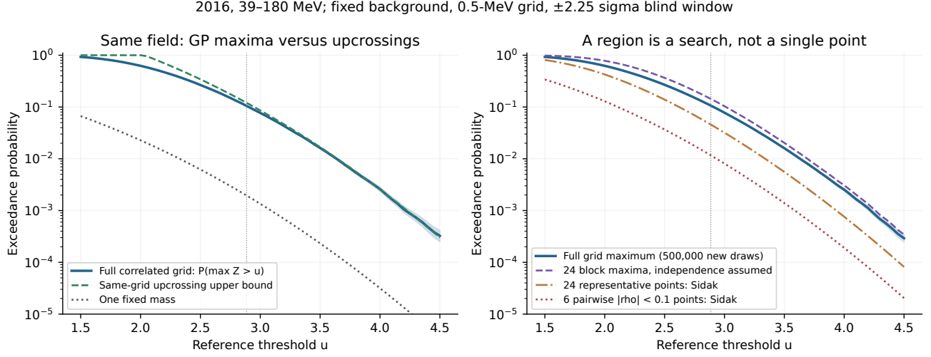
Figure 11: Retained 2016 comparison with the source and test held fixed. Left: the sampled Gaussian maximum is less conservative than the analytic upcrossing bound for the same finite grid. Right: counting representative points misses searches within the intervening regions; treating the properly calculated region maxima as independent errs in the other direction in this example. The left curve reuses 200,000 saved fields; the right uses 500,000 fresh fields with the same covariance. Shading denotes binomial 95% intervals for the joint maxima. These are fixed-background diagnostics.
