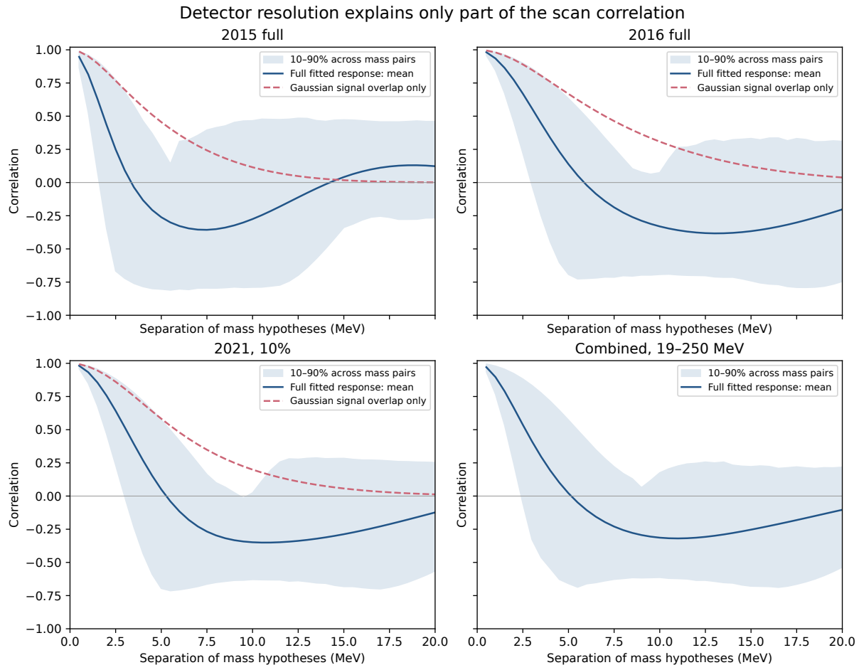
Figure 4: Reproduction of v5.8.3 Figure 4. The fitted-response correlation is compared with Gaussian-template overlap. Shading describes variation across mass pairs, not uncertainty in a measured correlation. These are the saved nominal-source fields, with no new fits.
