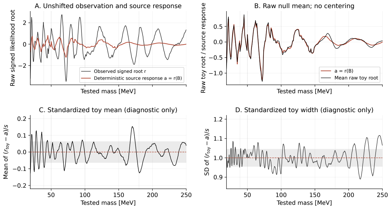
Figure 9: Shared coupling: extension of Figure 4 in the consolidated v5.8.5 report. A: the unshifted observed root and deterministic source response. B: the mean raw toy root and the same deterministic response. C/D: standardized toy mean and width, used only to inspect the conditional response approximation; the observed local curves in Figure 2 are not standardized. Gray bands mark approximate pointwise one-standard-error scales for 256 Gaussian draws, not simultaneous acceptance bands. Vertical lines mark changes in contributing datasets; these are not independent additional searches.
