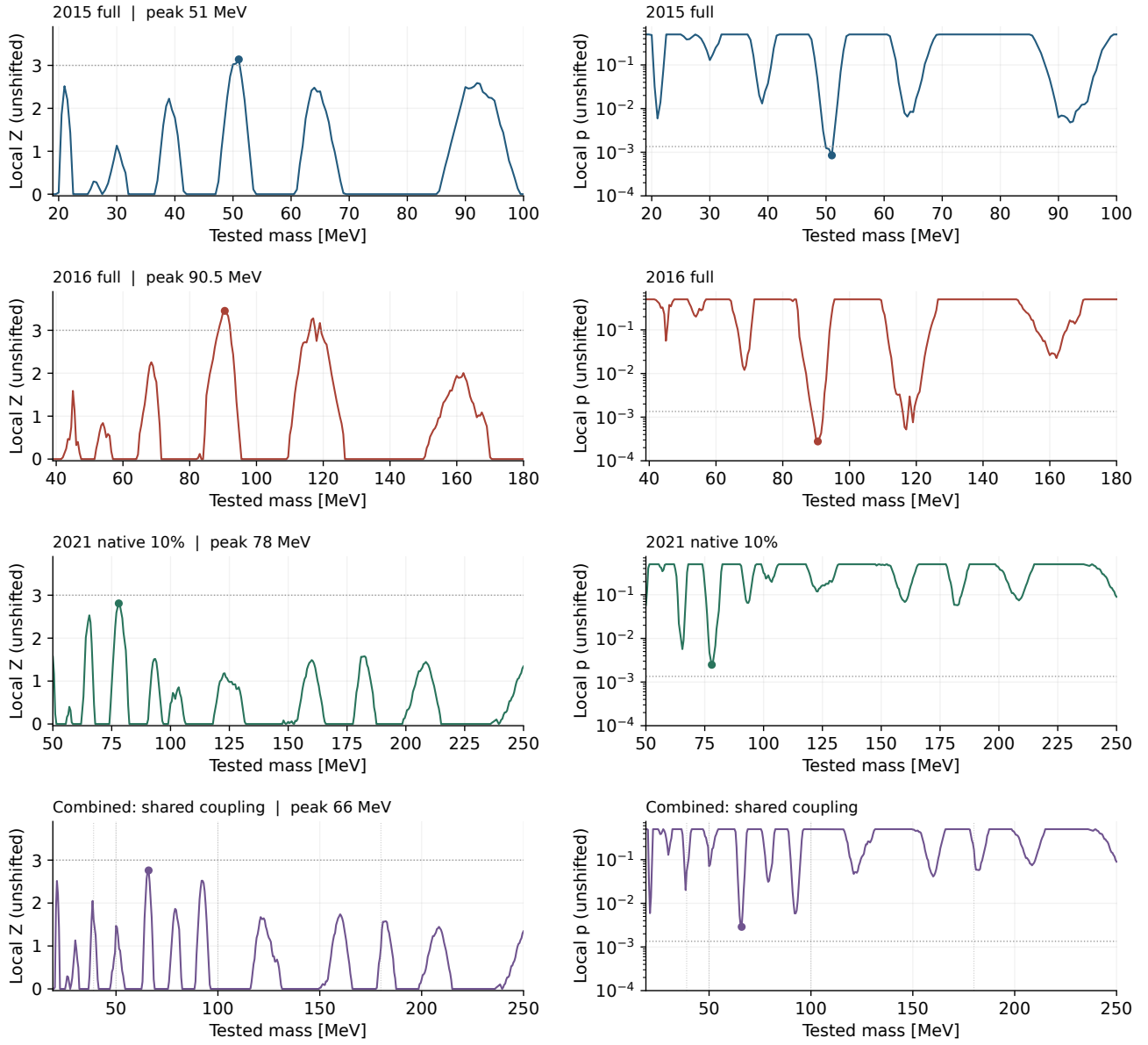
Figure 2: The requested non-recalibrated local significance and p-value curves for every dataset and the shared-coupling combination. Left: Z = \max(r_{\text{obs}}, 0) . Right: p = \bar{\Phi}(Z) ; dotted horizontal lines mark the conventional local 3\sigma level. Dots identify the raw maximum of each scope. Neither panel uses the reference offset or response scale. The mass ranges differ by dataset; dotted vertical lines in the combined row mark changes in contributing datasets.
