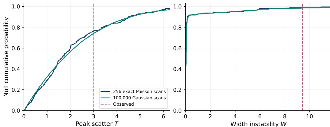
Figure 14: The earlier v5.8.5 coherence check on 80–100 MeV. The lower tail, not the upper tail, measures unusually close peak locations. The observed clustering gives 195/256 direct lower-tail counts, or add-one probability 0.76265, and is not unusual under the fixed-source null. The four historical widths enter this archived sensitivity diagnostic; this review makes no new width choice.
