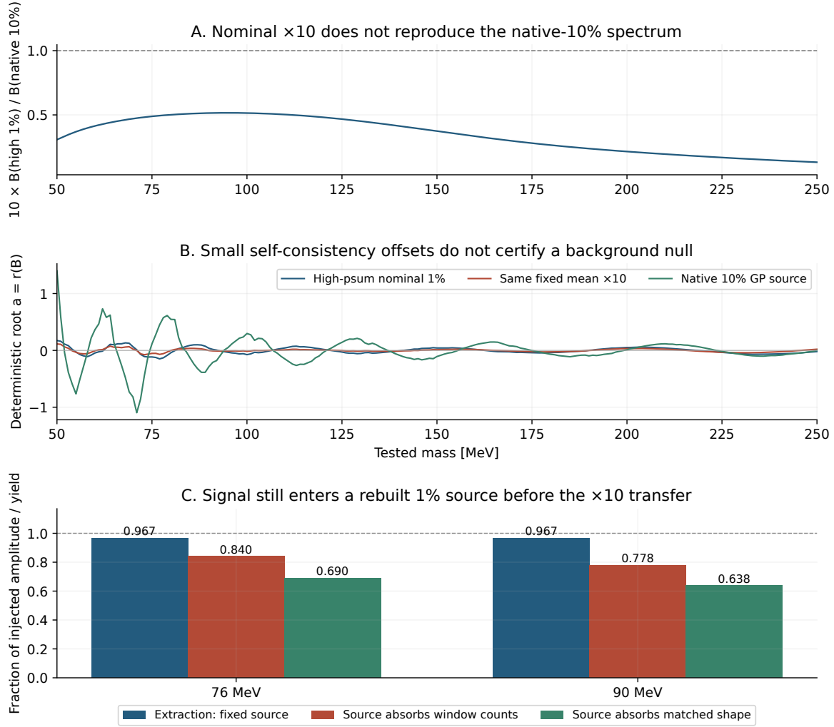
Figure 10: New fixed-width 2021 controls. A: the nominally scaled high-psum source is only about 13–52% of the native-10% GP mean over 50–250 MeV, with substantial shape dependence. B: deterministic source responses using the same extraction settings. C: fixed-source recovery versus source rebuilding after a known signal injection. The two source-learning bars use different projections of the same rebuilt mean; neither is a probability. The smaller offsets in B do not repair the transfer mismatch or the absorption in C.
