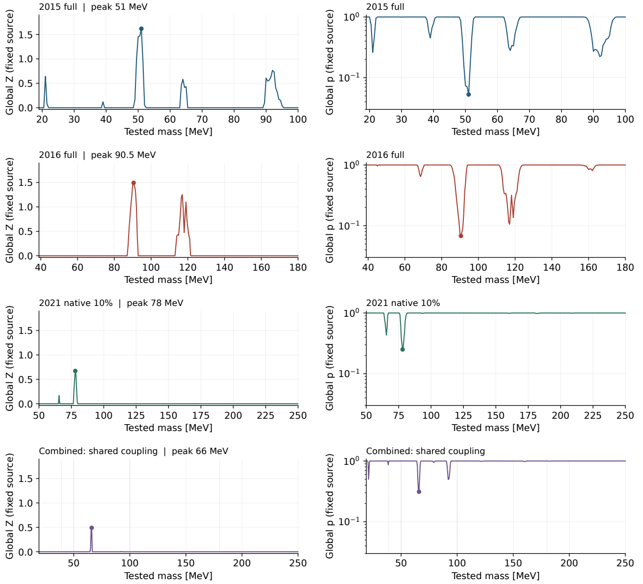
Figure 3: Global probabilities and displayed Z for the raw maximum , conditional on each unchanged nominal GP source. The observed likelihood roots are unshifted. Each tail searches the entire support of its row, not only the mass shown on the horizontal axis. Dots identify the same raw peaks as Figure 2; a fixed maximum distribution preserves their ranking. Shading represents finite Gaussian-field sampling only. These global panels have a different probability construction from the asymptotic local panels.
