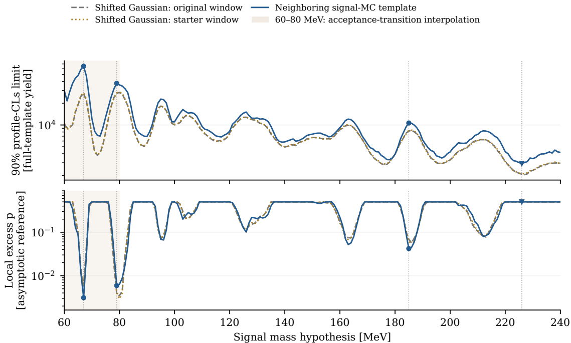
2021 10% observed spectrum: compare the assumed signal shapes
