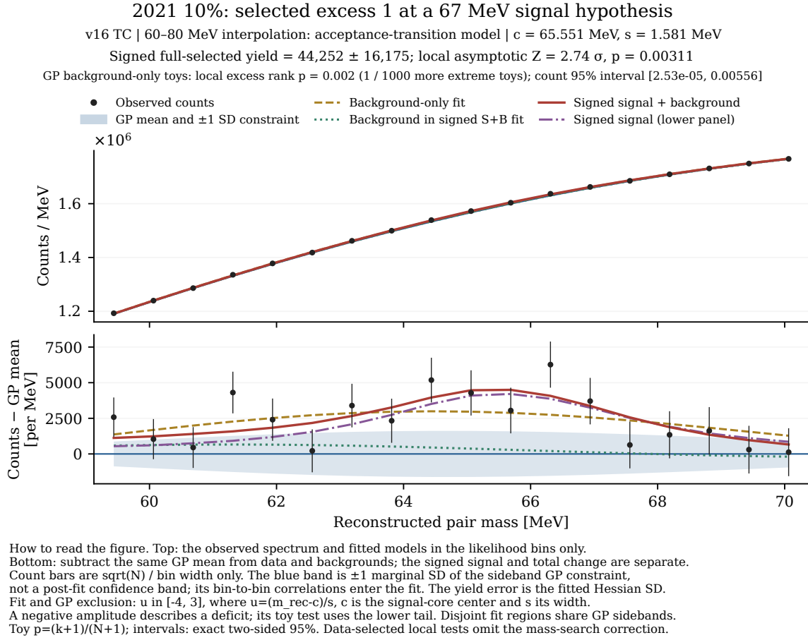
Figure 34. How to read the figure. Black points are observed counts per MeV with count-only \sqrt{N}/\Delta m bars. Blue is the sideband GP mean with its marginal one-standard-deviation constraint band, not a post-fit confidence band. Gold profiles the background with signal fixed to zero. Green is the background component of the signed signal-plus-background fit; red is its total. The lower panel subtracts the GP mean and shows the signed signal separately in purple. Correlated background uncertainties enter the likelihood. All model curves are restricted to the fitted bins, which are excluded from GP training. Yield errors are conditional profile-Hessian standard deviations. The displayed probabilities are local; selection in the observed mass scan is not included. The annotated positive local significance is the asymptotic likelihood reference; the separate toy rank uses 1,000 GP-source backgrounds.
