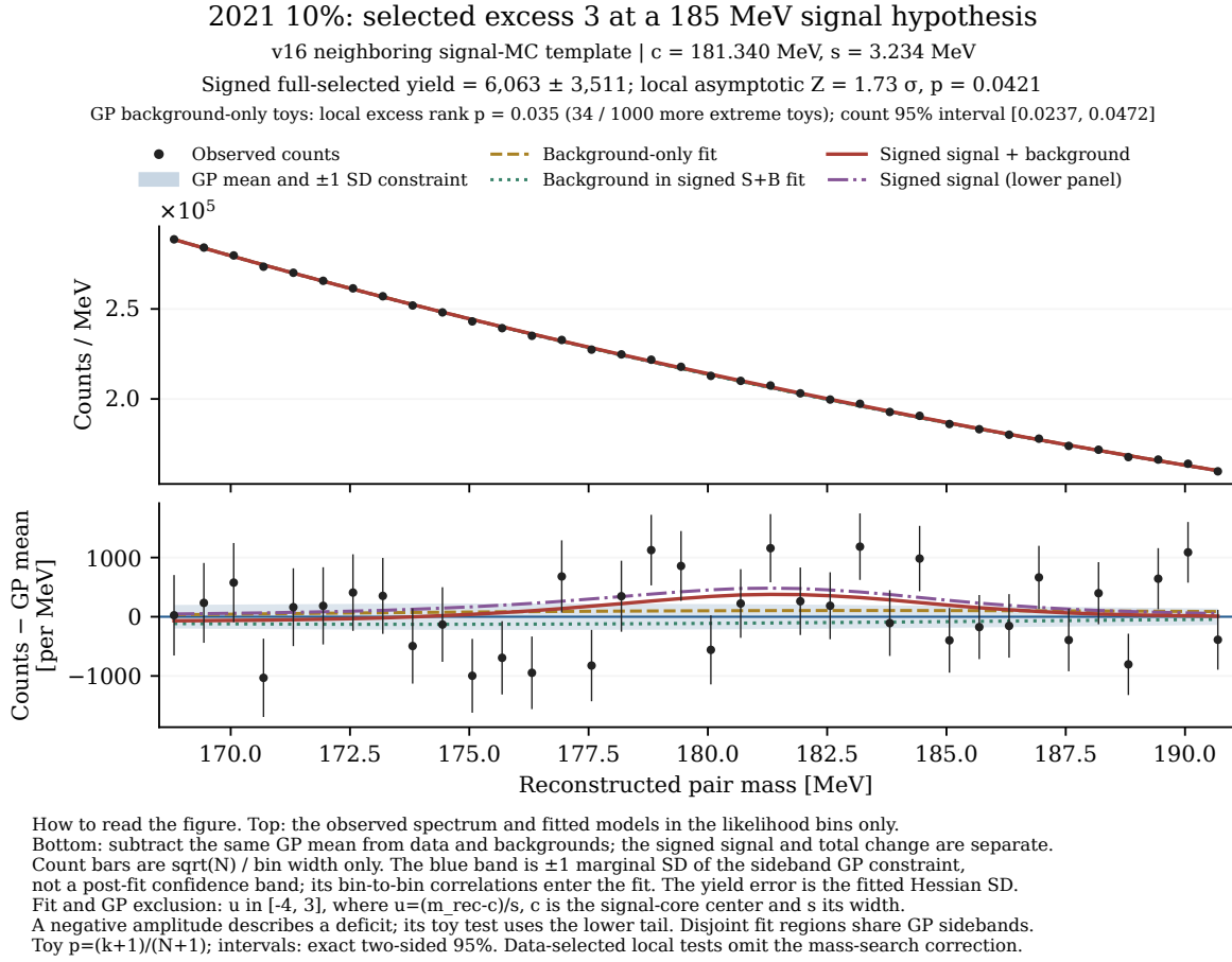
Figure 36. How to read the figure. Black points are observed counts per MeV with count-only \sqrt{N}/\Delta m bars. Blue is the sideband GP mean with its marginal one-standard-deviation constraint band, not a post-fit confidence band. Gold profiles the background with signal fixed to zero. Green is the background component of the signed signal-plus-background fit; red is its total. The lower panel subtracts the GP mean and shows the signed signal separately in purple. Correlated background uncertainties enter the likelihood. All model curves are restricted to the fitted bins, which are excluded from GP training. Yield errors are conditional profile-Hessian standard deviations. The displayed probabilities are local; selection in the observed mass scan is not included. The annotated positive local significance is the asymptotic likelihood reference; the separate toy rank uses 1,000 GP-source backgrounds.
