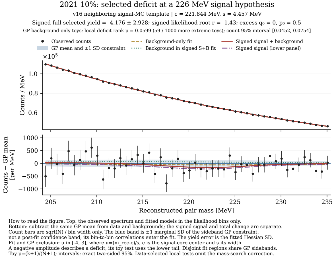
Figure 37. How to read the figure. Black points are observed counts per MeV with count-only \sqrt{N}/\Delta m bars. Blue is the sideband GP mean with its marginal one-standard-deviation constraint band, not a post-fit confidence band. Gold profiles the background with signal fixed to zero. Green is the background component of the signed signal-plus-background fit; red is its total. The lower panel subtracts the GP mean and shows the signed signal separately in purple. Correlated background uncertainties enter the likelihood. All model curves are restricted to the fitted bins, which are excluded from GP training. Yield errors are conditional profile-Hessian standard deviations. The displayed probabilities are local; selection in the observed mass scan is not included. The negative signed fit describes a downward fluctuation; the nonnegative-signal best fit is the background-only curve.
