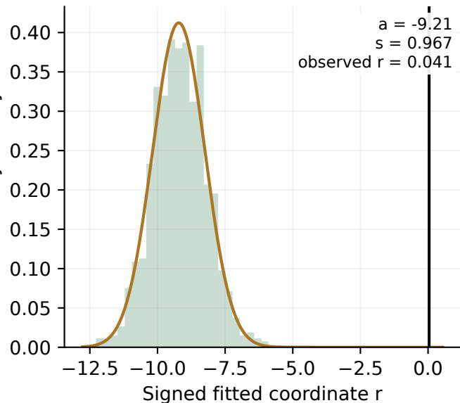
2016 at 42 MeV
