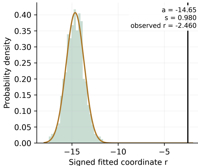
2016 at 76 MeV
