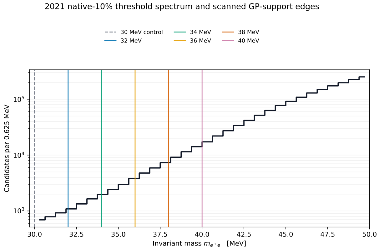
Figure 50: Native 2021 10% source histogram near threshold. Vertical lines mark the 30 MeV control and the five candidate lower edges of the GP support. The logarithmic vertical scale makes the low-count shoulder and rapid turn-on visible.
