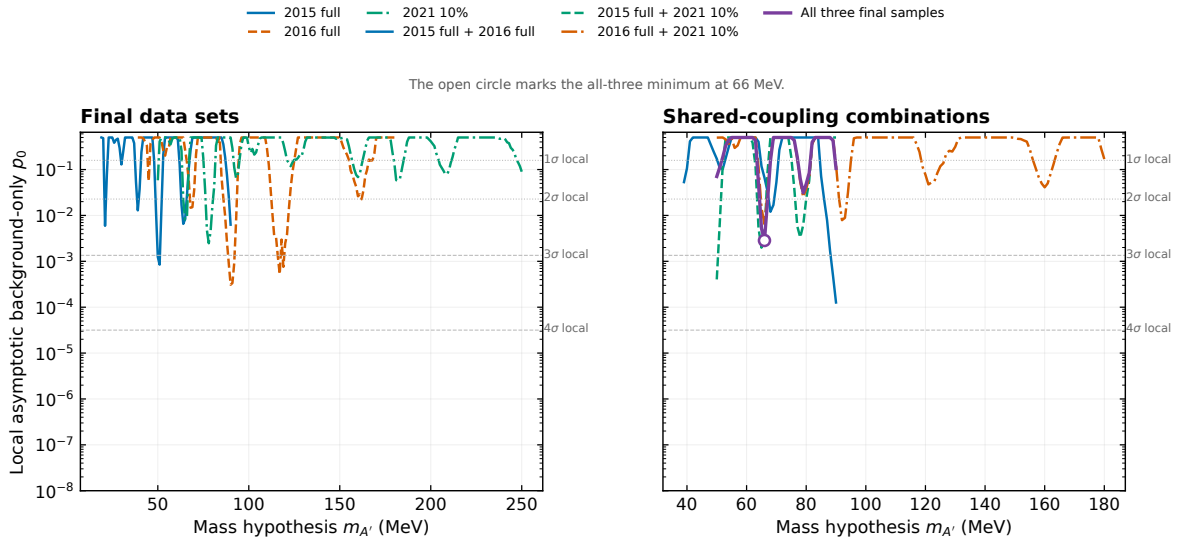
Figure 126: Historical parent Figure 59: final asymptotic pvalues. This saved display uses the former 2015 endpoint of 90 MeV. The corresponding v5.0.4 result is Figure 59.
