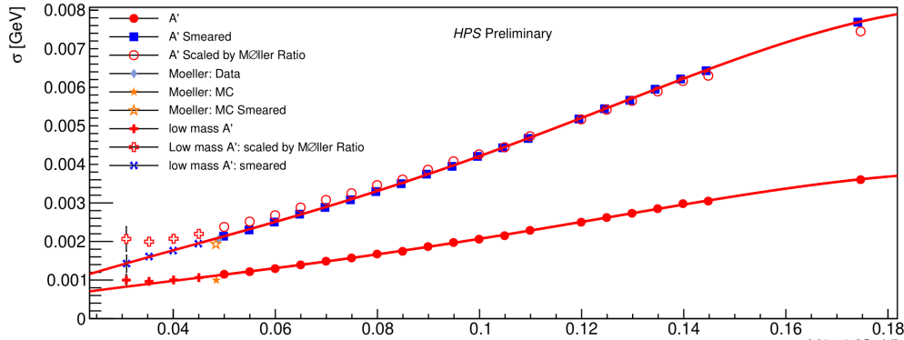
Figure 15: 2016 smeared- A' and Møller-based mass-resolution summary [31]. The smeared A' points show how the data-driven momentum-smearing correction is propagated away from the single Møller calibration point. The worsening resolution with mass broadens the signal window and is one of the main detector effects limiting prompt sensitivity at higher mass.
