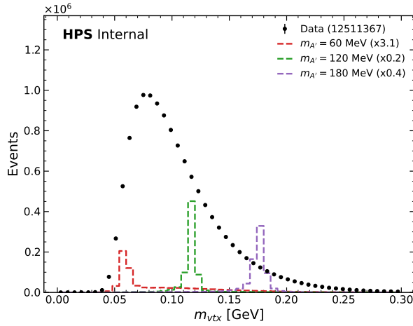
(a) Vertex invariant mass.
