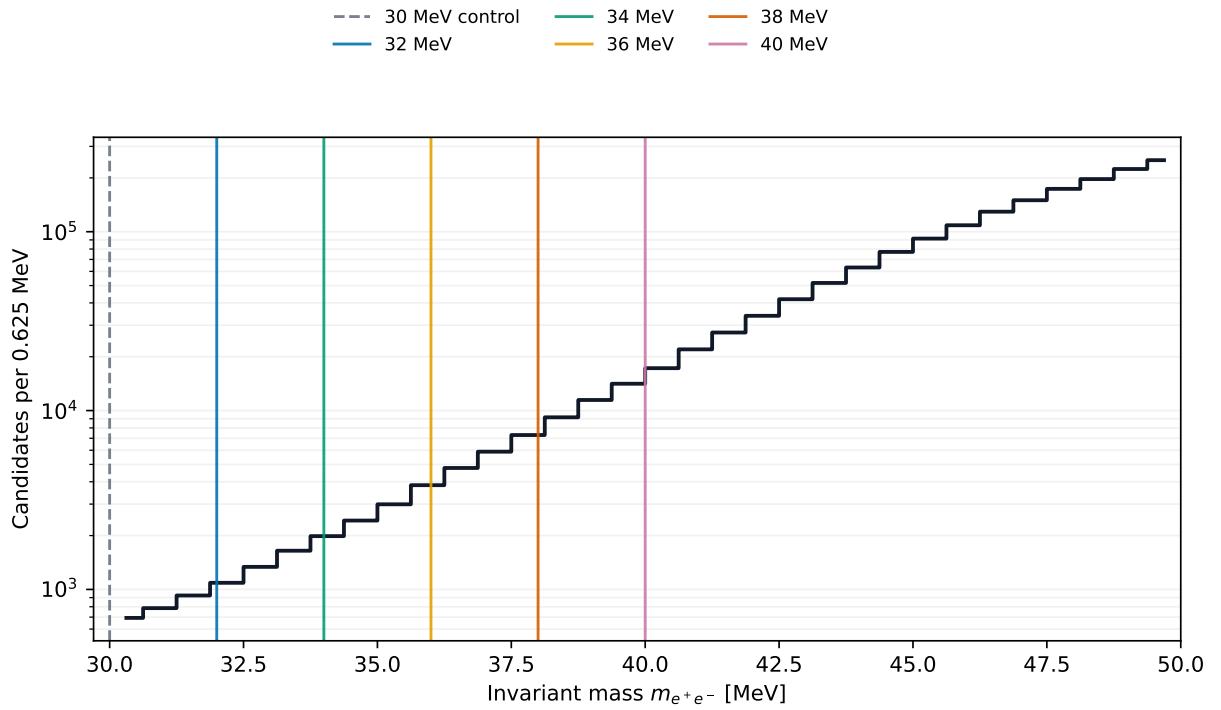
Figure 52: Native 2021 10% source histogram near threshold. Vertical lines mark the 30 MeV control and the five candidate lower edges of the GP support. The logarithmic vertical scale makes the low-count shoulder and rapid turn-on visible.
