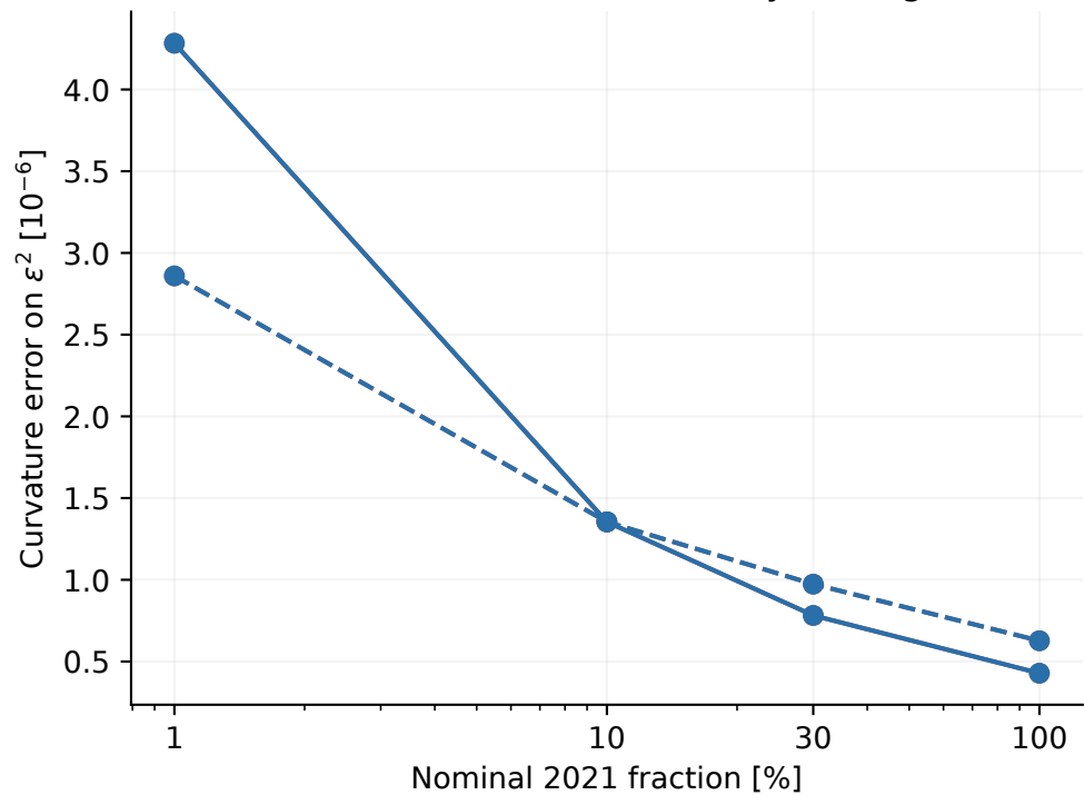
Two assumed GP-uncertainty scalings
