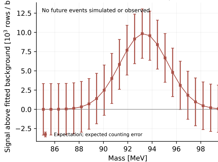
Conditional nominal 100% expectation
