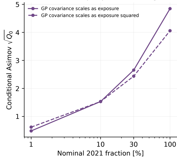
Frozen fitted shape; profiled background
