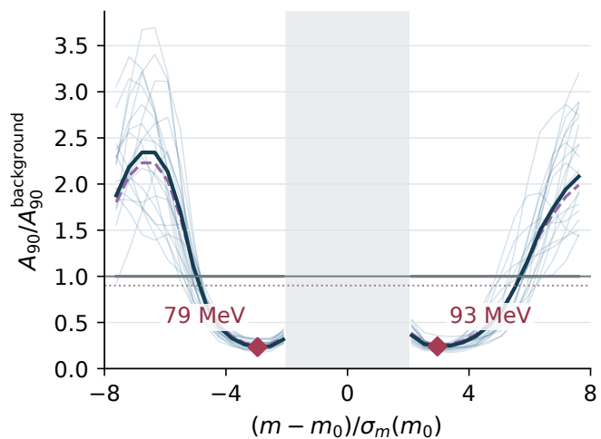
Limit ratio in the two search flanks
