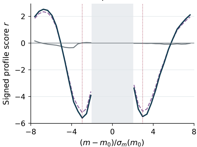
Asimov fit response in the flanks
