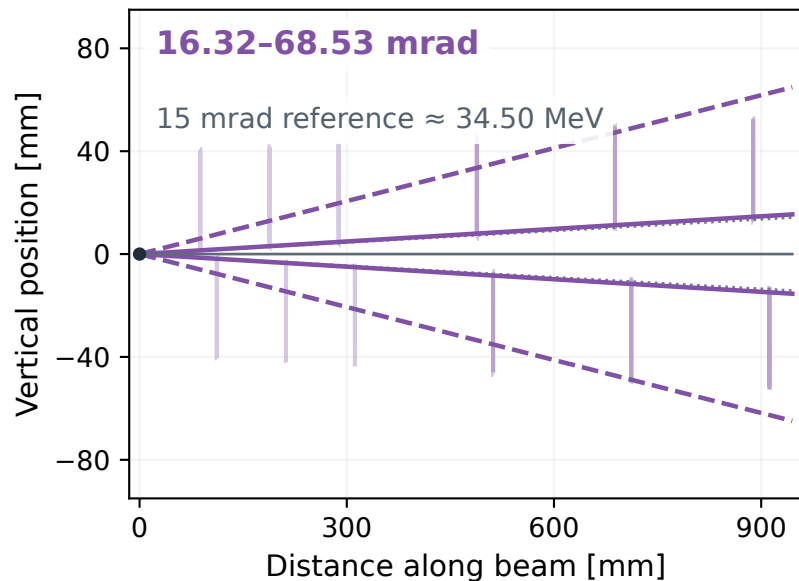
HPS 2016 | 2.300 GeV
