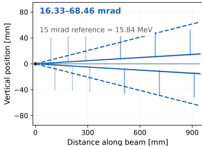
HPS 2015 | 1.056 GeV
