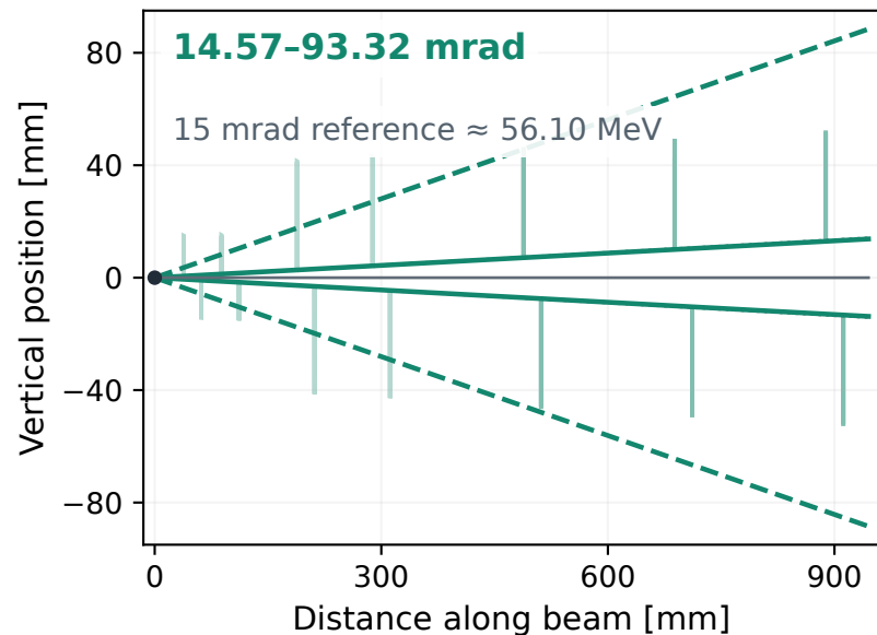
HPS 2021 | 3.740 GeV
