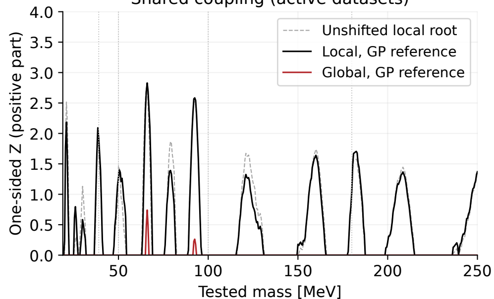
Shared coupling (active datasets)
