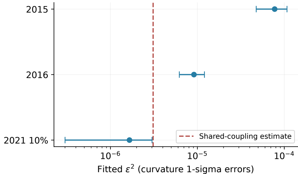
92 MeV: separate fitted couplings
