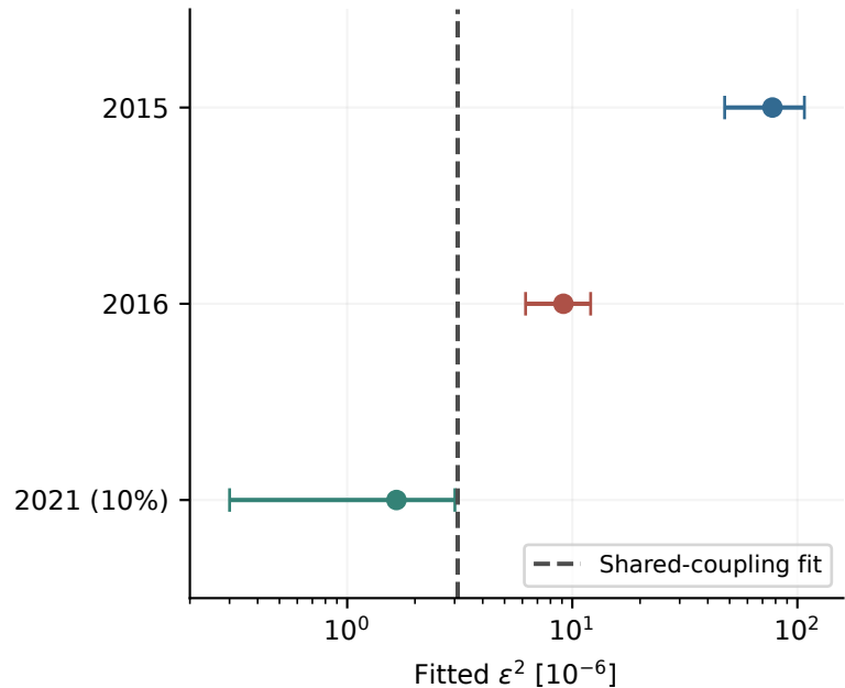
At 92 MeV: common mass is not common rate
