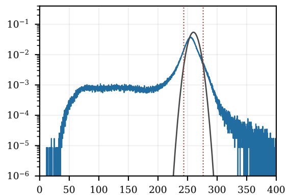
Reconstructed m_{ee} (MeV)
