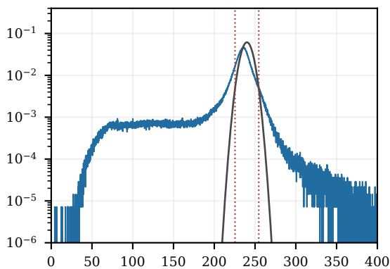
Reconstructed m_{ee} (MeV)
