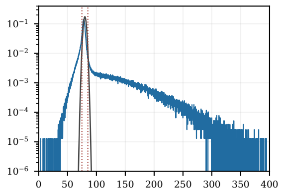
140 MeV; N_{\text{eff}}=1,966,199
