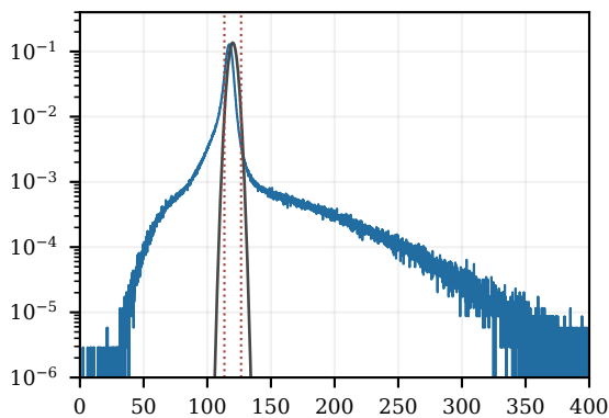
180 MeV; N_{\text{eff}}=1,998,339
