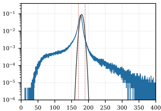
240 MeV; N_{\text{eff}}=1,388,655
