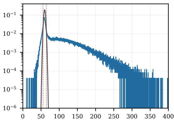
120 MeV; N_{\text{eff}}=3,448,406
