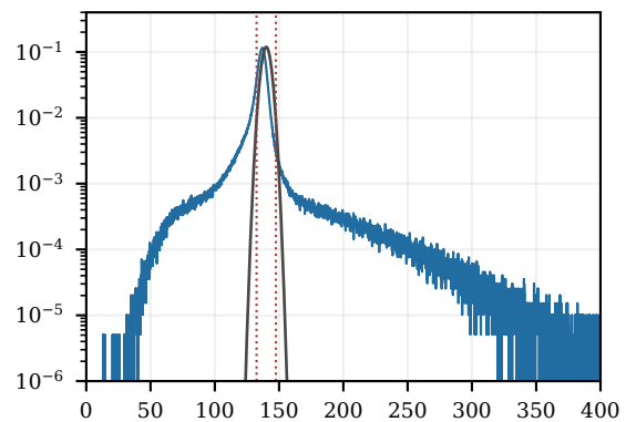
200 MeV; N_{\text{eff}}=1,837,830
