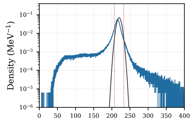
Reconstructed m_{ee} (MeV)
