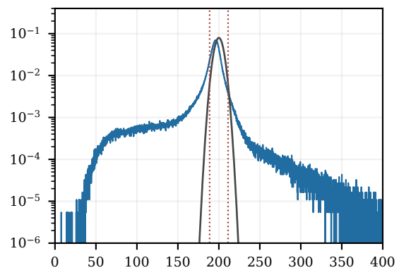
260 MeV; N_{\text{eff}}=1,157,665
