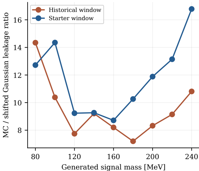
Compare shapes in the same bins
