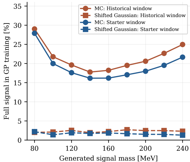
Signal MC has more tail probability
