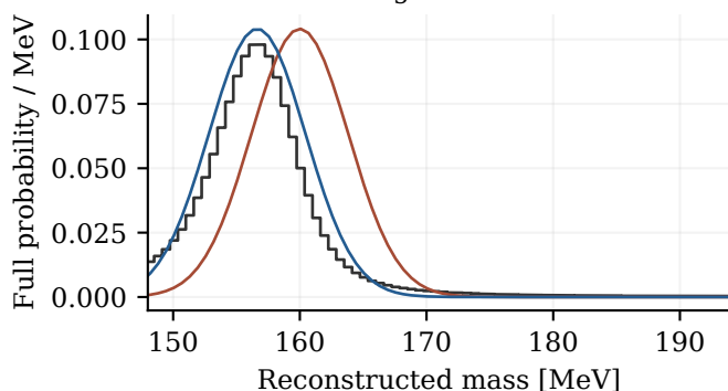
Generated signal mass 160 MeV
