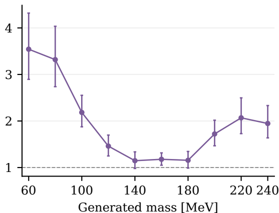
Relative background-only yield noise after response scaling
