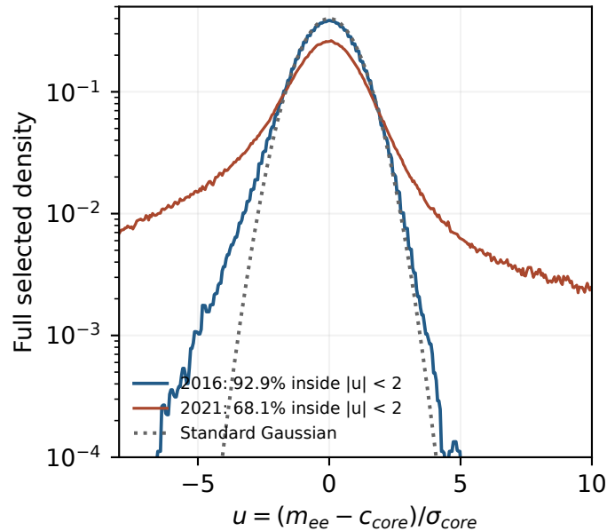
100 MeV samples
