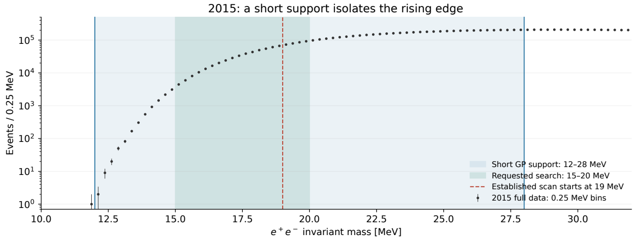
Figure 25: The same released full-2015 histogram, summed from 0.05 to 0.25 MeV bins. The chosen GP support is 12–28 MeV; the requested search is 15–20 MeV. The dashed line marks the lower boundary of the established scan, not the lower boundary of the available counts.
