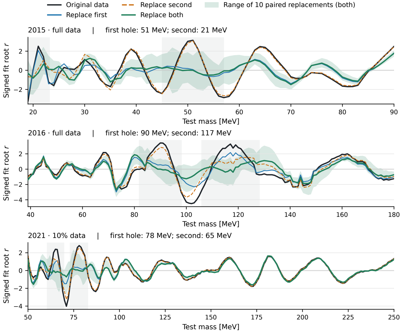
Figure 5: Observed scans before and after replacement. Black: original data. Blue and dashed orange: deterministic replacement of the first or second listed region. Green: both. The light green envelope spans the ten paired, conditional GP-plus-Poisson replacements with both holes filled; it is not a confidence band. Gray vertical regions show the primary holes. Curves join the existing 1 MeV hypotheses without extra smoothing. The ordinate is a signed profile root, not a newly calibrated significance. Removing a peak’s own bins predictably weakens that feature; the informative changes are in the surrounding pattern and retained regions.
