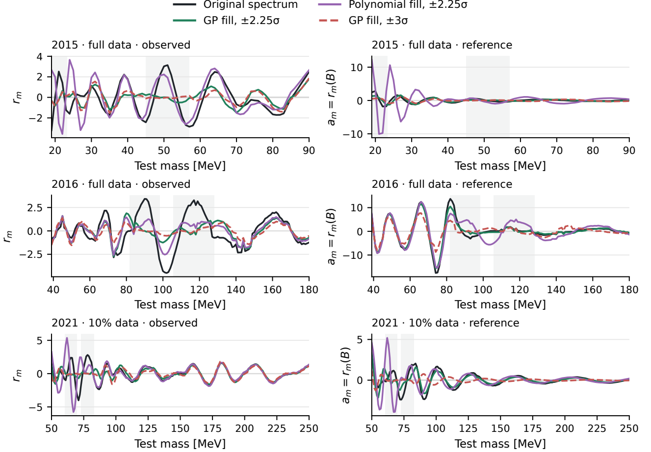
Figure 6: Both-hole replacements in observed counts (left) and the reference spectrum (right). Green: primary GP mean. Purple: exponential-polynomial fill. Dashed red: wider GP holes. The reference ordinate a_m = r_m(B) is the fitted root, not the background event rate. Gray shading marks primary holes; wider holes extend beyond it. All outcomes remain visible, including unsuccessful interpolation. No altered spectrum supplies a new observed-data probability.
