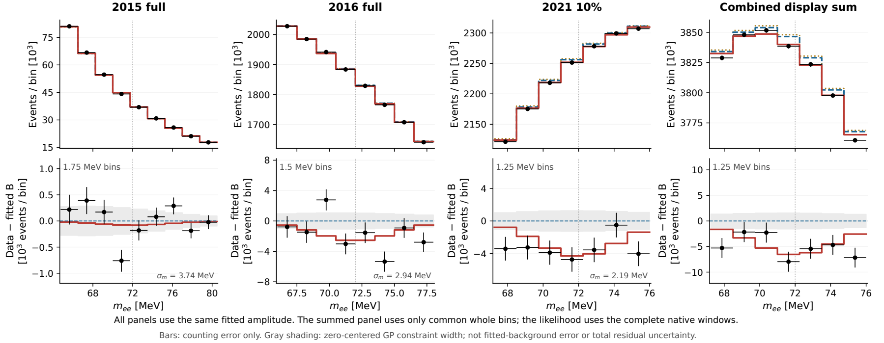
Figure 13: The deepest raw combined deficit has r = -3.49 and a signed auxiliary amplitude \hat{\epsilon}^2 = -4.88 \times 10^{-6} . All three separate amplitudes are negative, with 2021 providing the strongest individual contribution. Negative templates describe missing events relative to the fitted background, not a physical negative coupling.
