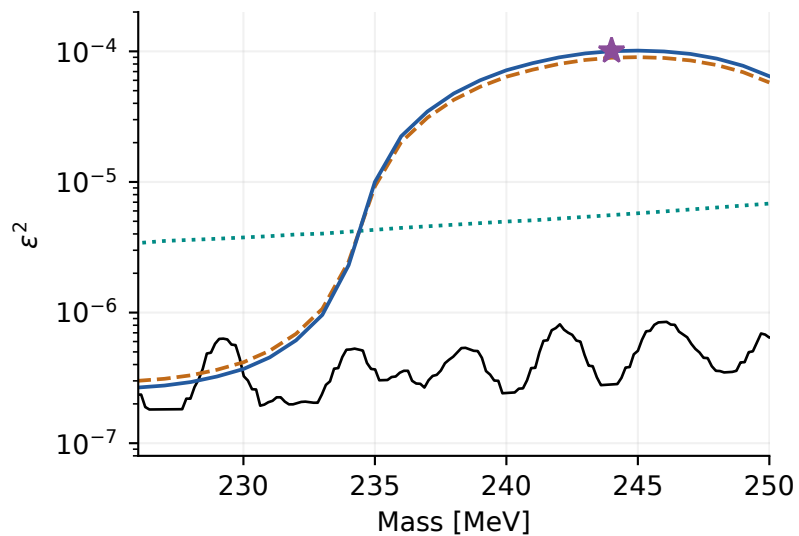
Historical 1% to 100%: 244 MeV
