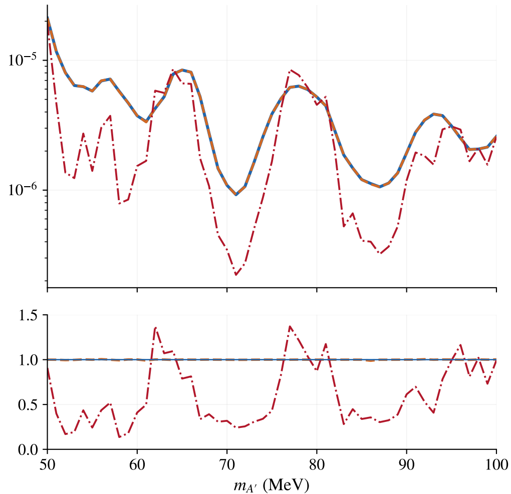
Low-mass detail
