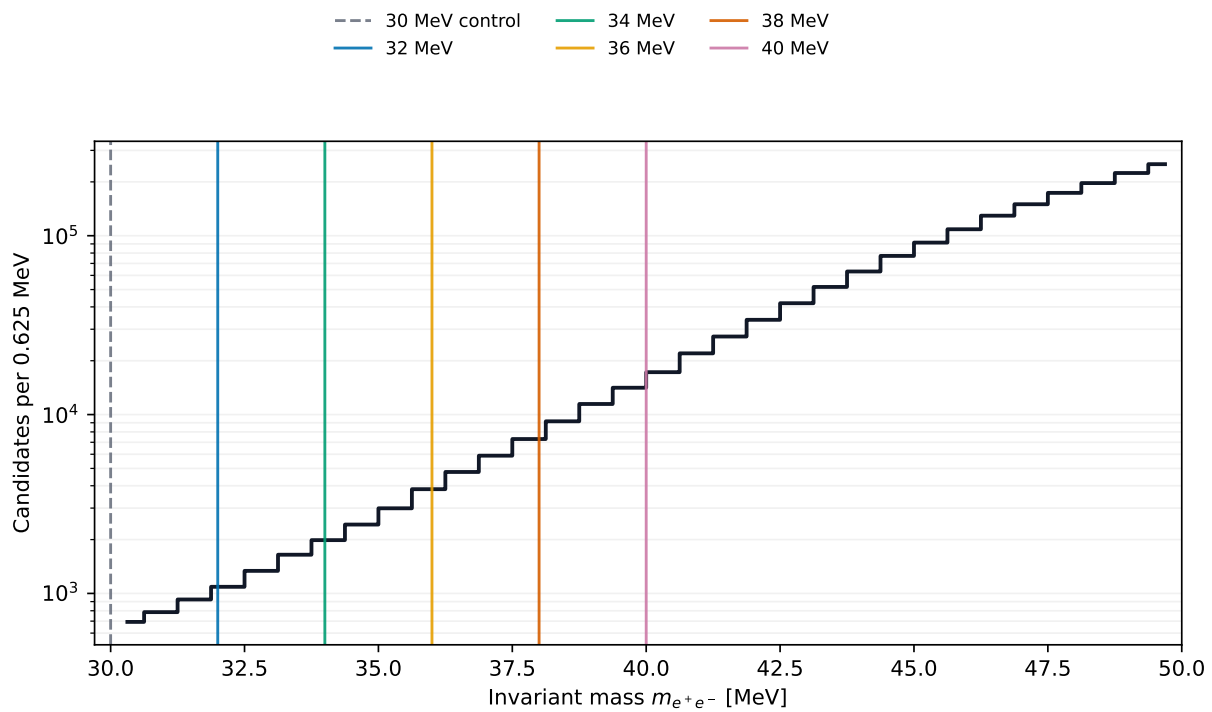
Figure 50: Native 2021 10% source histogram near threshold. Vertical lines mark the 30 MeV control and the five candidate lower edges of the GP support. The logarithmic vertical scale makes the low-count shoulder and rapid turn-on visible.
