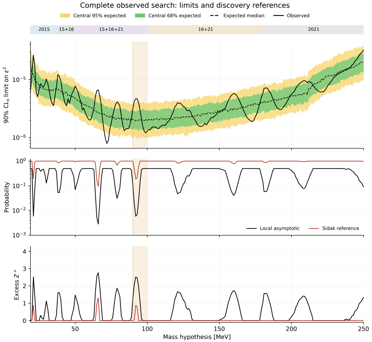
Figure 52: Complete 19–250 MeV observed search, with the preassigned active datasets shown above the curves. The upper panel shows 90% \text{CL}_s limits and the median, central 68% and central 95% ranges of the 300 conditional background-only toys per mass, with newly computed bands at the added 2015 coordinates. The next two panels show the fixed-mass asymptotic p_0 and its normal-quantile significance, with the local reference in black and the Sidak reference in red. The latter uses N_{\text{eff}} = 35.381 for the complete search; its value at 66 MeV is Z_{\text{Sidak}} = 1.305 , compared with local Z = 2.765 . The observed polyline connects every adjacent tested mass, including membership transitions; no numerical endpoint is changed by those connections. The physical visible-branching correction is applied once above the dimuon threshold. These are pointwise bands; 2016-inclusive values retain the numerical exception.
