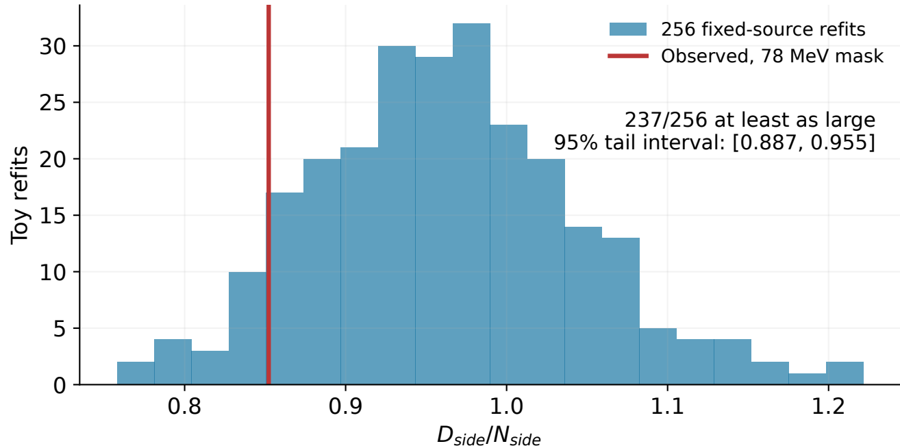
Conditional reference at 78 MeV
