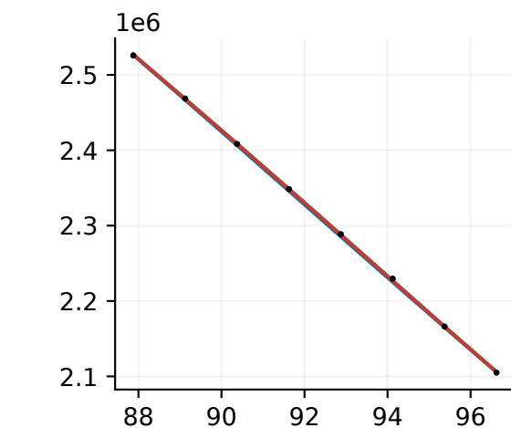
Common-bin sum
