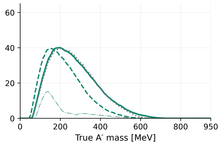
HPS 2021 | 3.740 GeV
