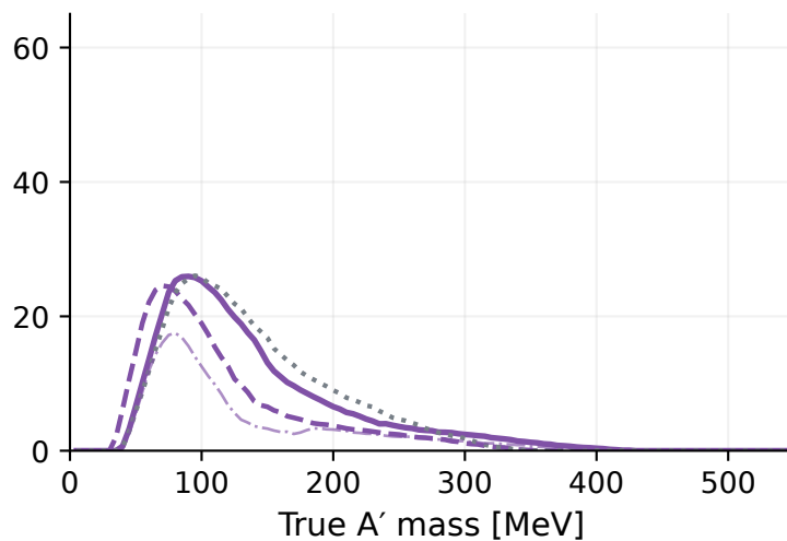
HPS 2016 | 2.300 GeV
