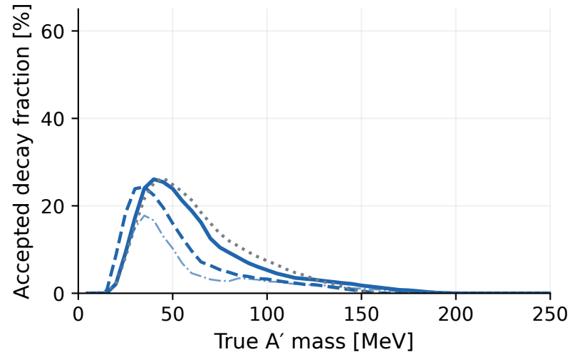
HPS 2015 | 1.056 GeV
