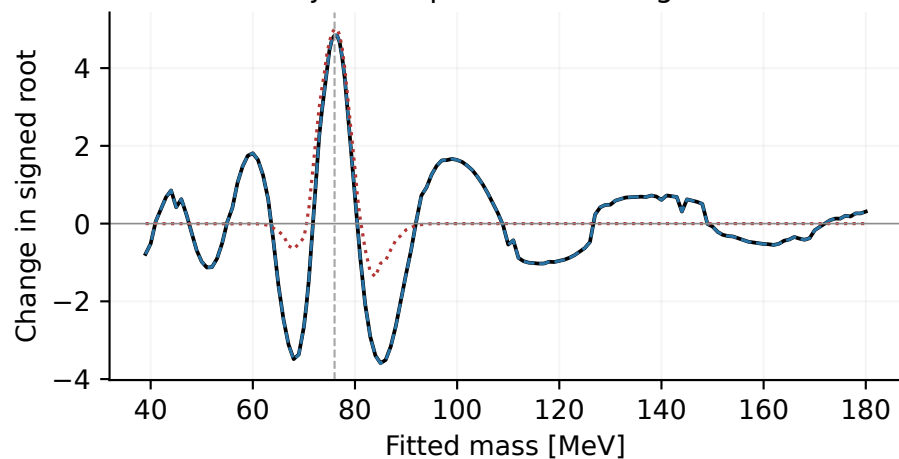
Size-five injection: positive and negative echoes
