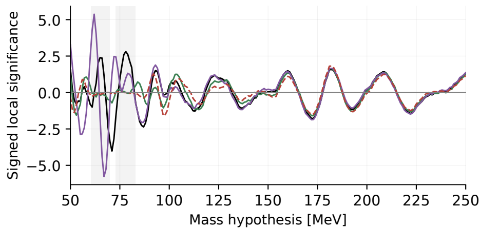
2021 observed data
