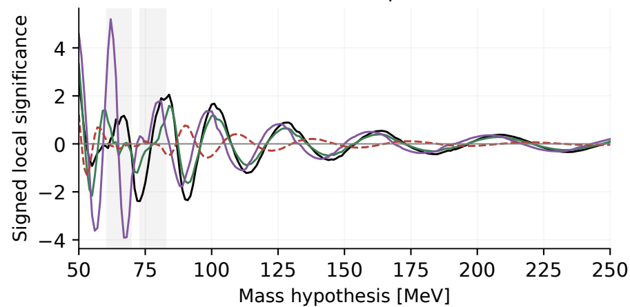
2021 reference spectrum
