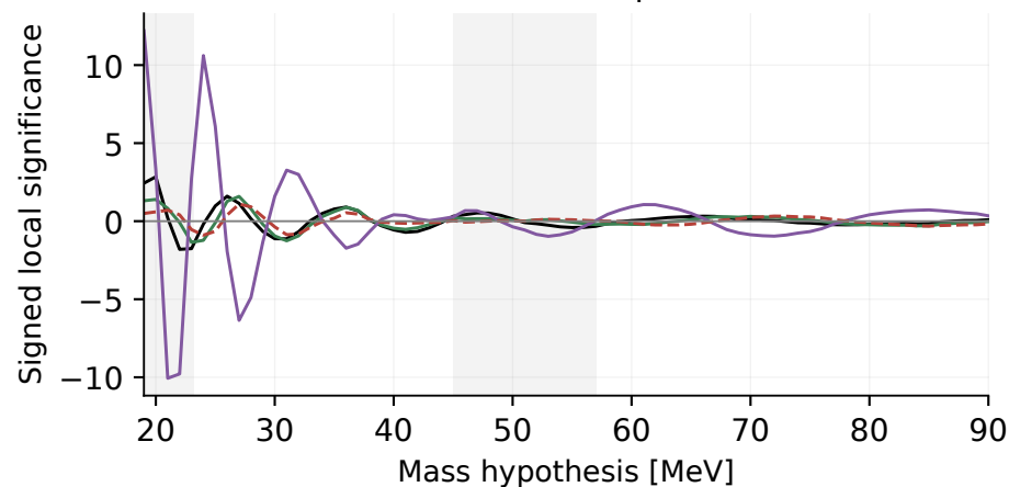
2016 reference spectrum
