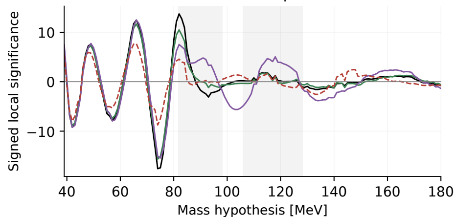
2021 reference spectrum
