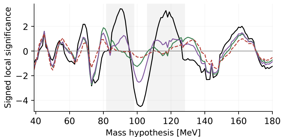
2021 observed data
