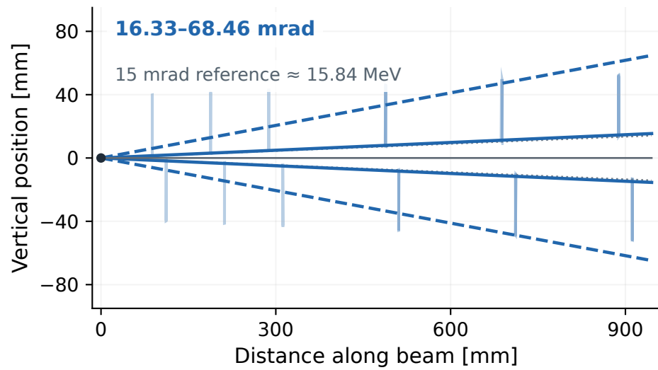
HPS 2015 | 1.056 GeV
