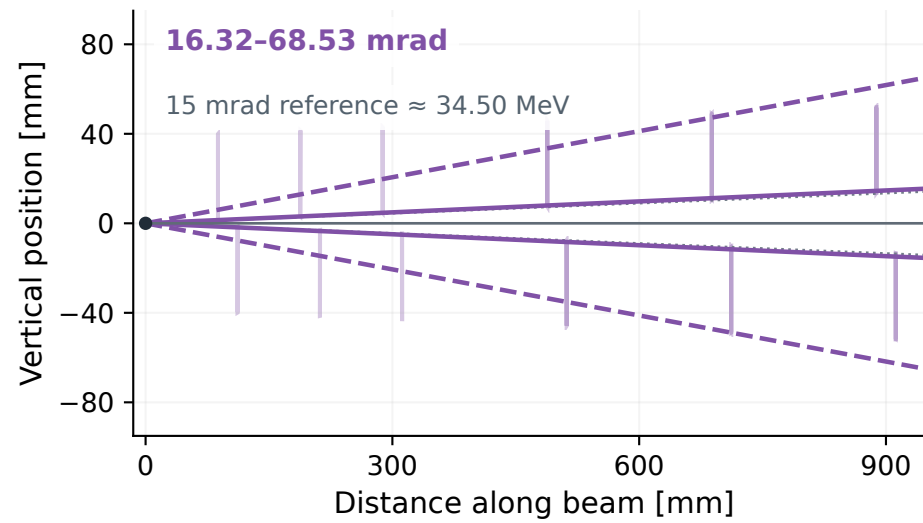
HPS 2016 | 2.300 GeV
