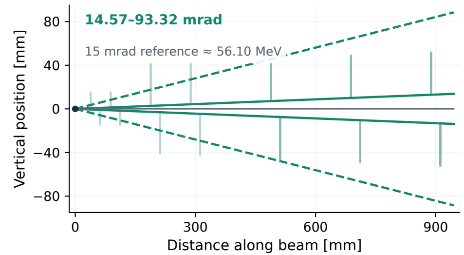
HPS 2021 | 3.740 GeV
