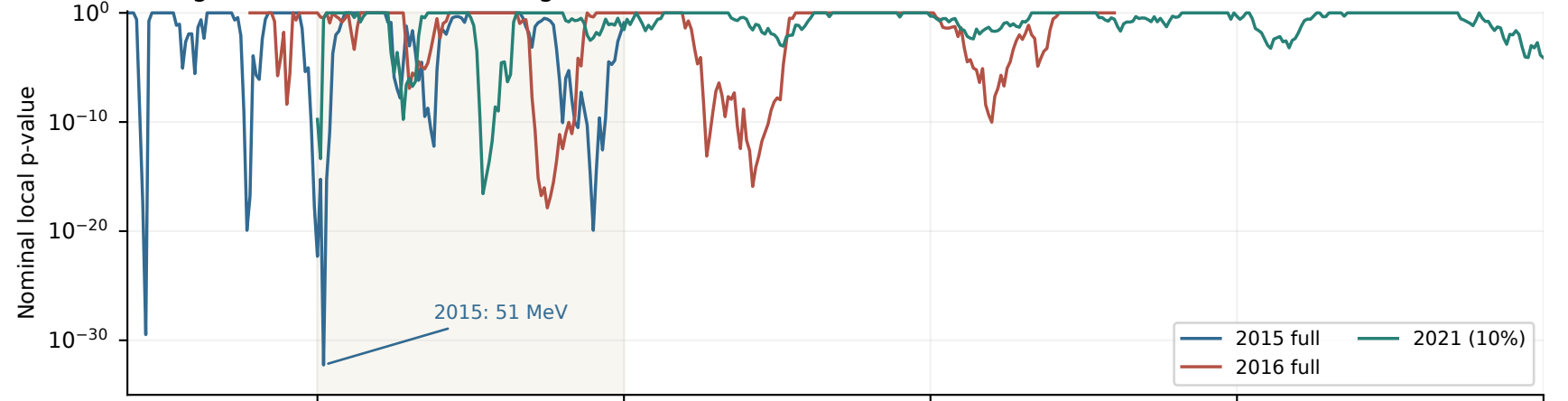
Background held fixed in the signal likelihood ( C = 0 )
