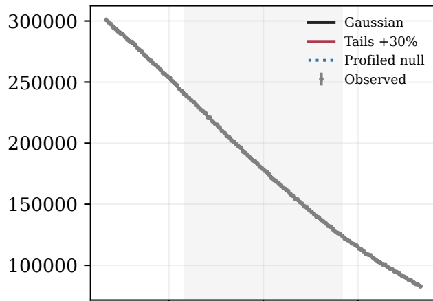
Full 2016, 90 MeV
