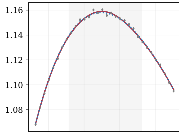
2021 (10%), 78 MeV
