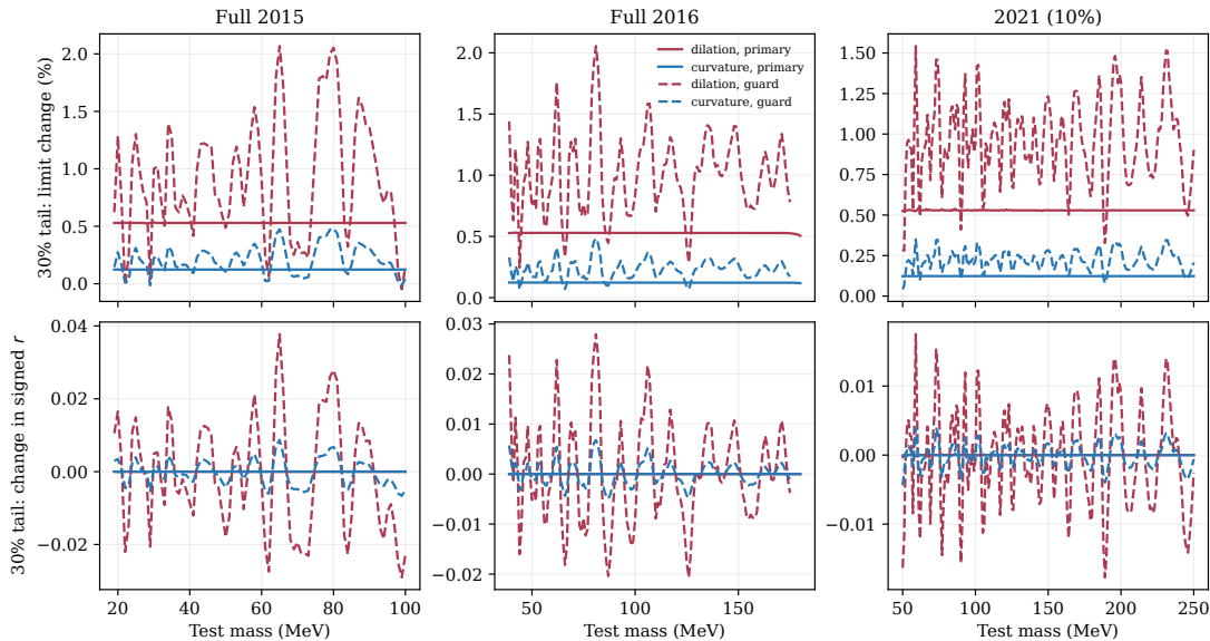
Figure 8: Response of the observed inference at the largest declared tail change, k = 1.3 : percent changes in the limit and changes in the signed likelihood root are compared with the Gaussian at each mass. Both tail families are shown, and primary and guard results retain their separate Gaussian references. Features in a mass scan reuse sideband information and should not be counted as independent evidence.
