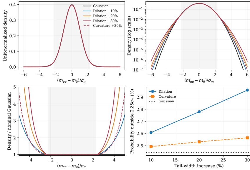
Figure 1: Smooth-dilation signal shapes and the 30% curvature control in units of the nominal mass resolution. The density curves use full-line normalization; the tail fraction panel summarizes both families. Changes to the unnormalized shape begin at the primary blind-window boundary.
