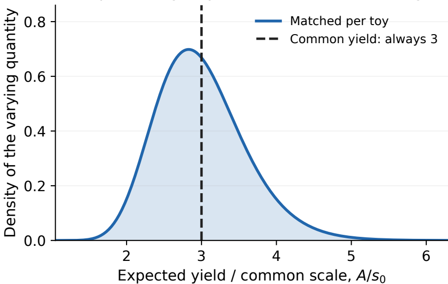
Expected signal yield varies under matching
