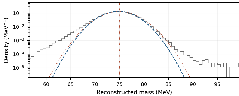
75 MeV; N = 280,200
