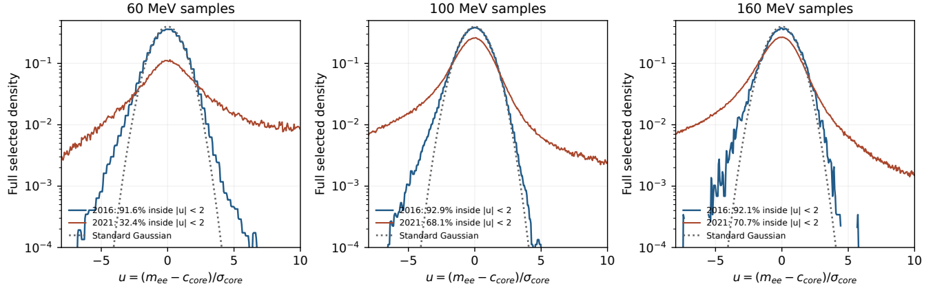
Figure 6. How to read the figure. Each year is aligned by its own fitted core center and width. Curves retain full selected normalization, including the saved 2021 overflow normalization. The percentages give the probability within |u| < 2 . The 2016 samples are more concentrated around their cores. This compares the supplied samples; it does not identify whether reconstruction, selection, calibration or another difference causes the change.
