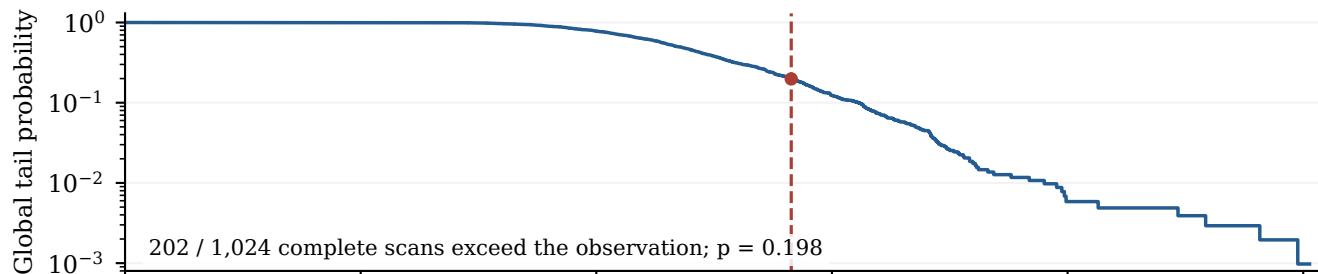
Combined: 2015 Gaussian + 2016 and 2021 MC
