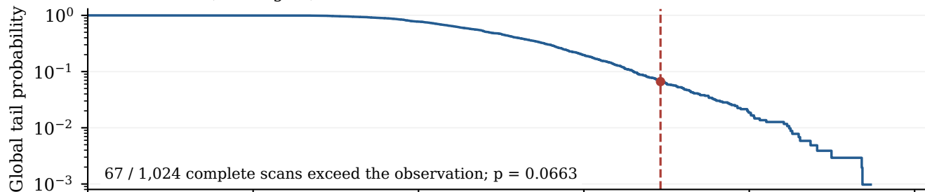
2016: full data, MC signal, \pm 2.5u
