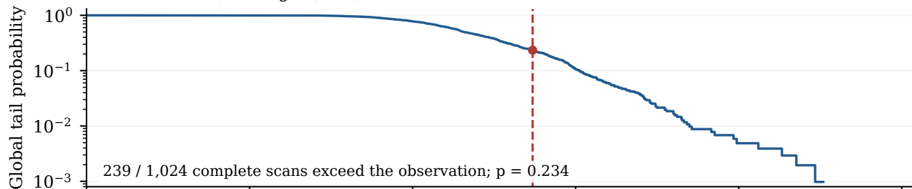
2021: 10% data, MC signal, [-4, +3]u
